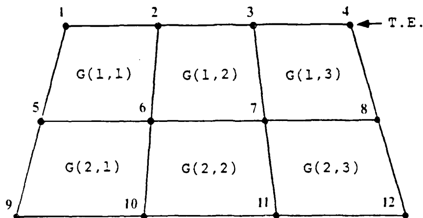
Figure 12. Finite Element Representation of the Wake
