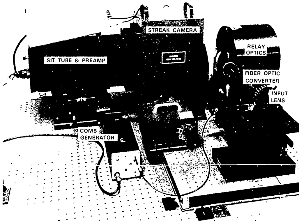
Figure 3: Photograph of first-generation system
