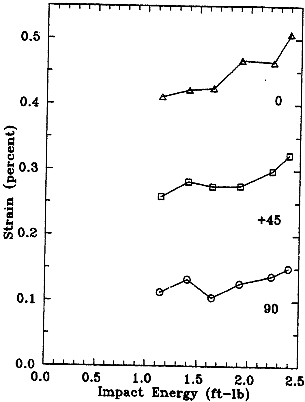
Figure 3.7. Maximum Strains as a Function of Impact Energy, [\pm 45]_{3s} Panels
