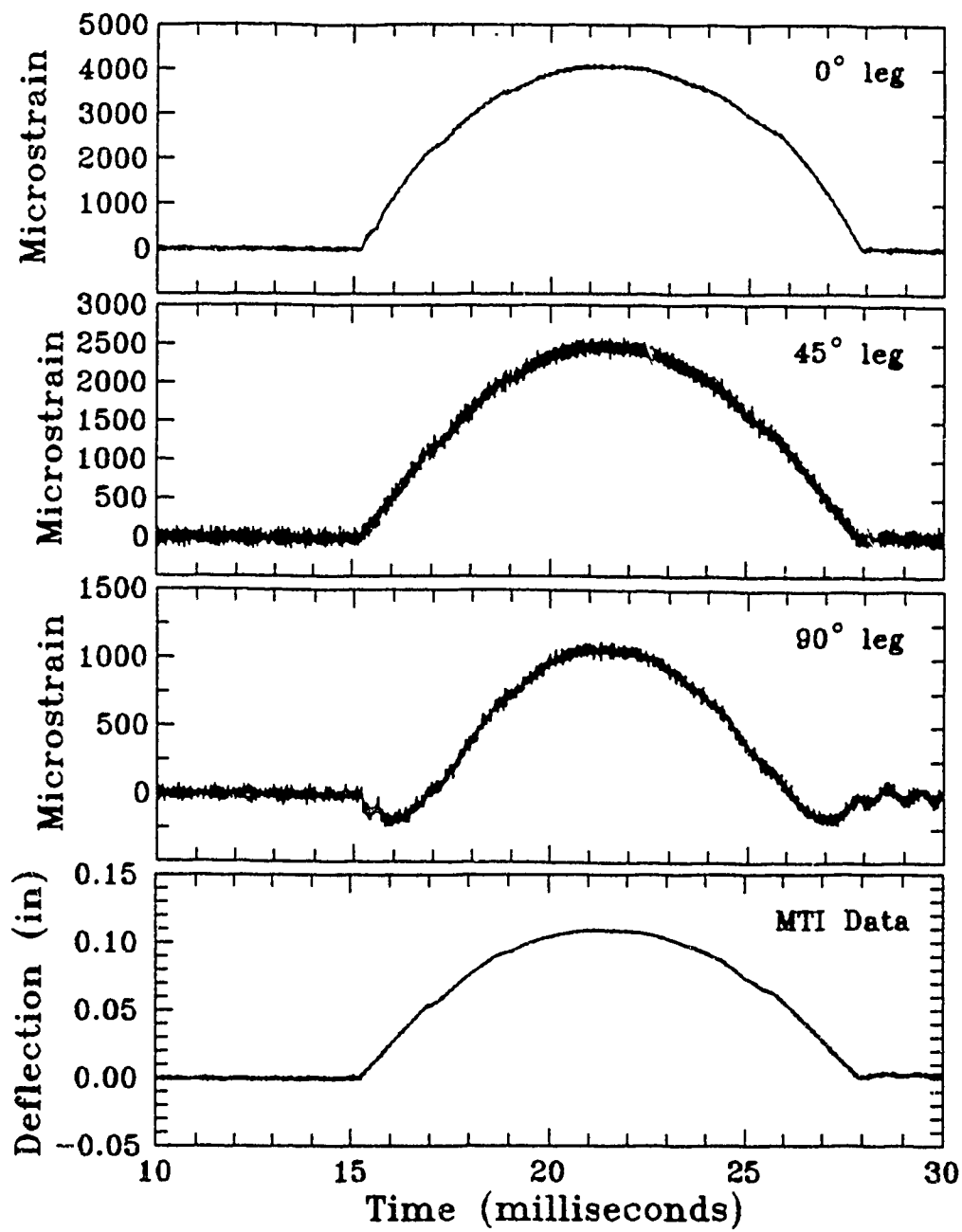
Figure B.45. Strain and Deflection for [\pm 45]_{3S} Panel, Impact Energy = 1.14 ft-lb
