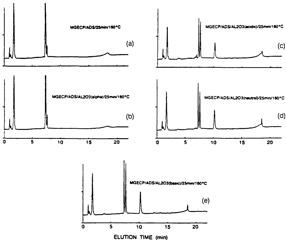
Figure 6. HPLC traces for a stoichiometric MGCEP/ADS (a) unfilled, (b) 50 phr corundum filled, (c) 50 phr A/A filled, (d) 50 phr A/N filled, and (e) 50 phr A/B filled mixtures heated for 25 minutes at 160°C.
