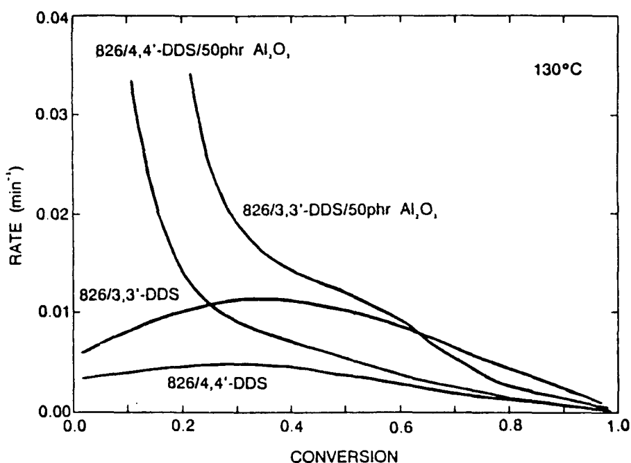
Figure 3. Isothermal rate versus extent of reaction traces from DSC at 130°C for unfilled and 50 phr activated aluminum oxide filled stoichiometric resin mixtures.
