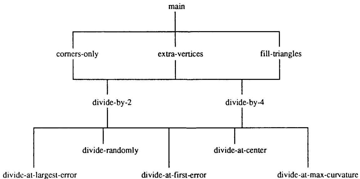
Figure 7. Adaptive Subdivision Variation Hierarchy
