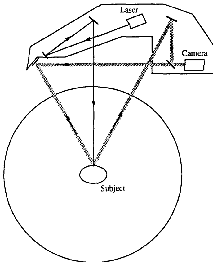
Figure 1. Schematic View of Cyberware Digitizer
