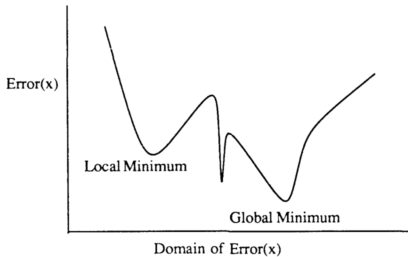
Figure 12. Local Minima in an Error Function
