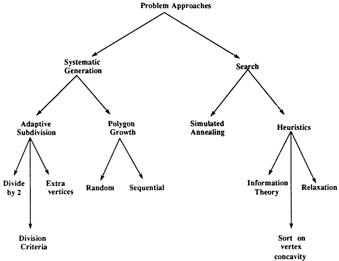
Figure 2. General Approaches to Data Reduction
