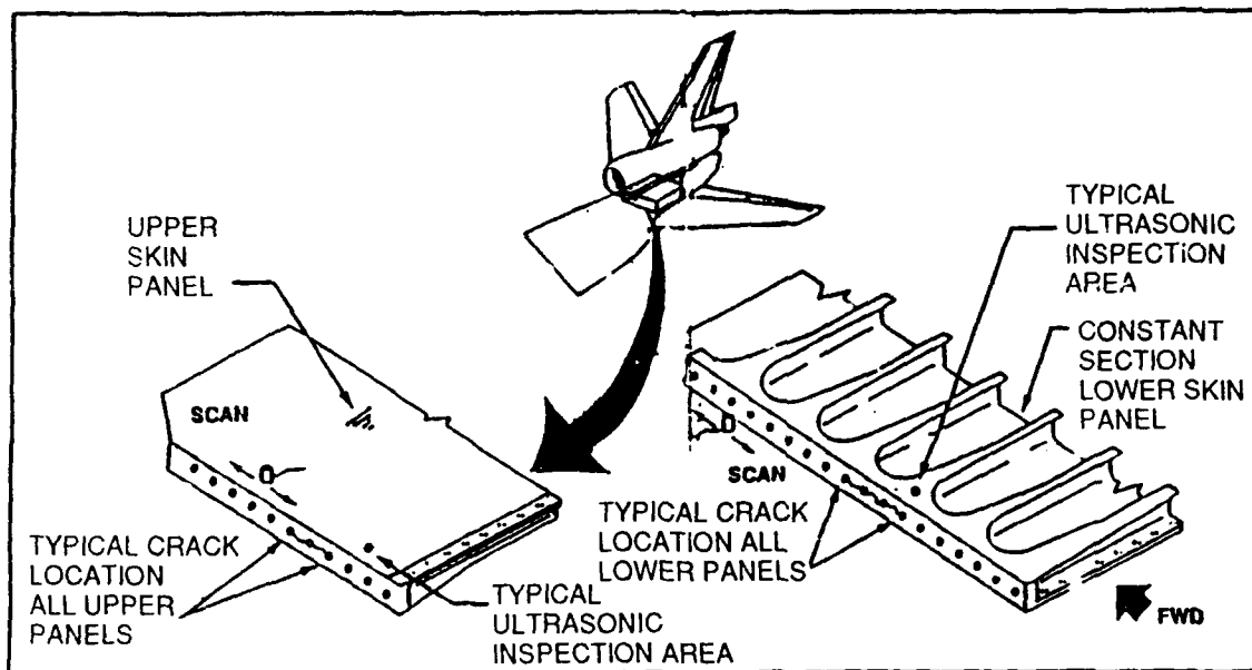
Figure 9. Typical crack environment for ultrasonic inspection.
