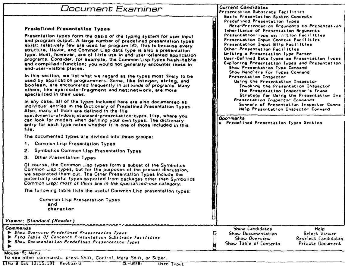
Figure 2. Document Examiner
