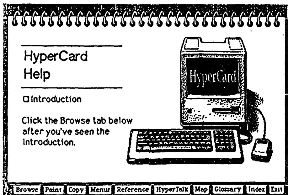
Figure 5. HyperCard Help
