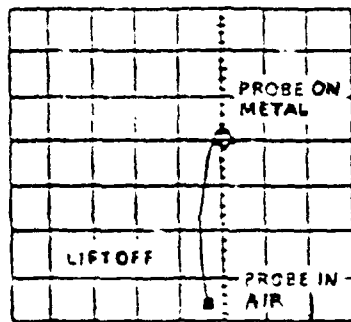
(A) EDDY CURRENT RESPONSE NO CORROSION
