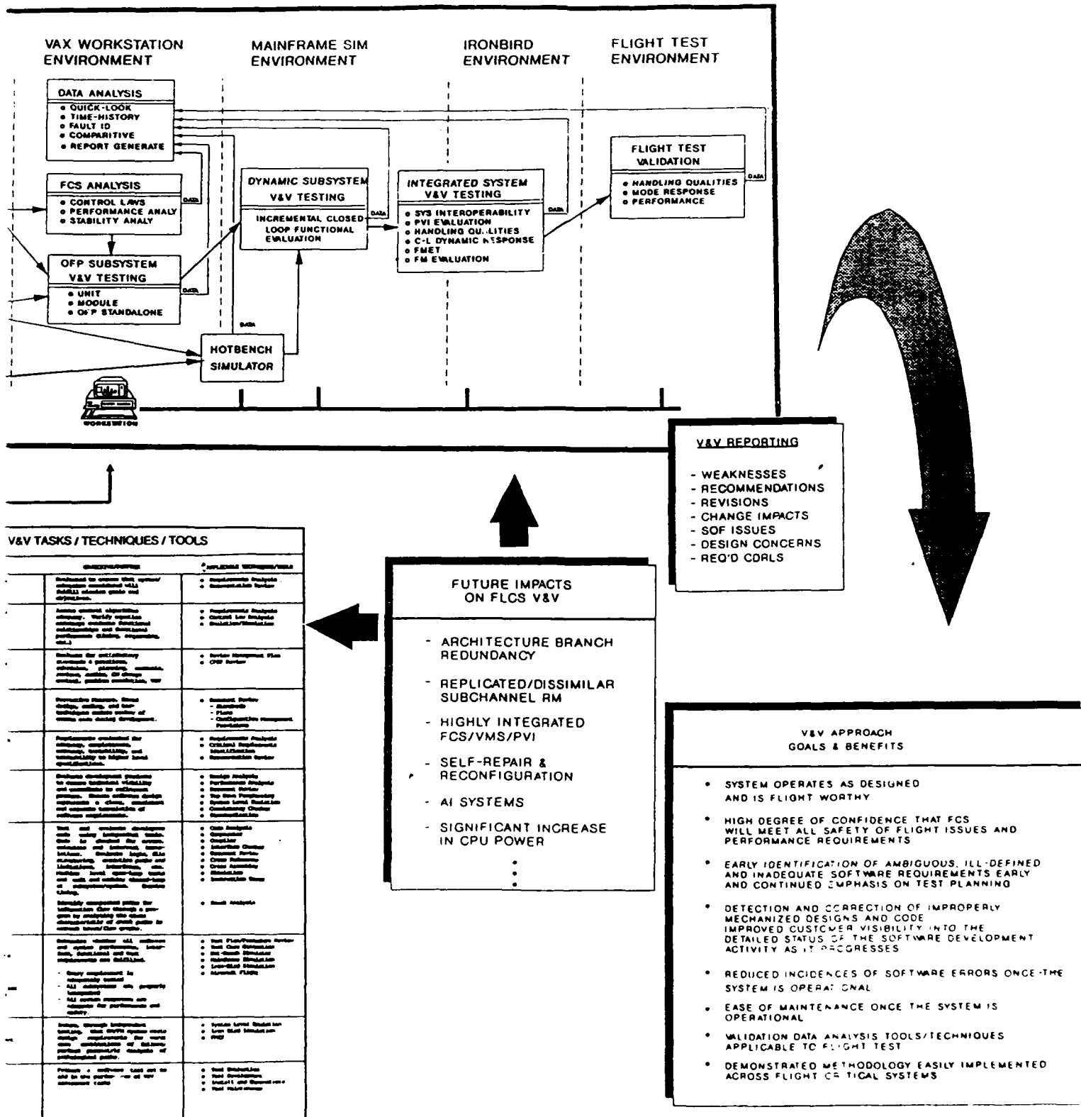
FIGURE 3.5.1-1 V&V METHODOLOGY DEVELOPMENT APPROACH
