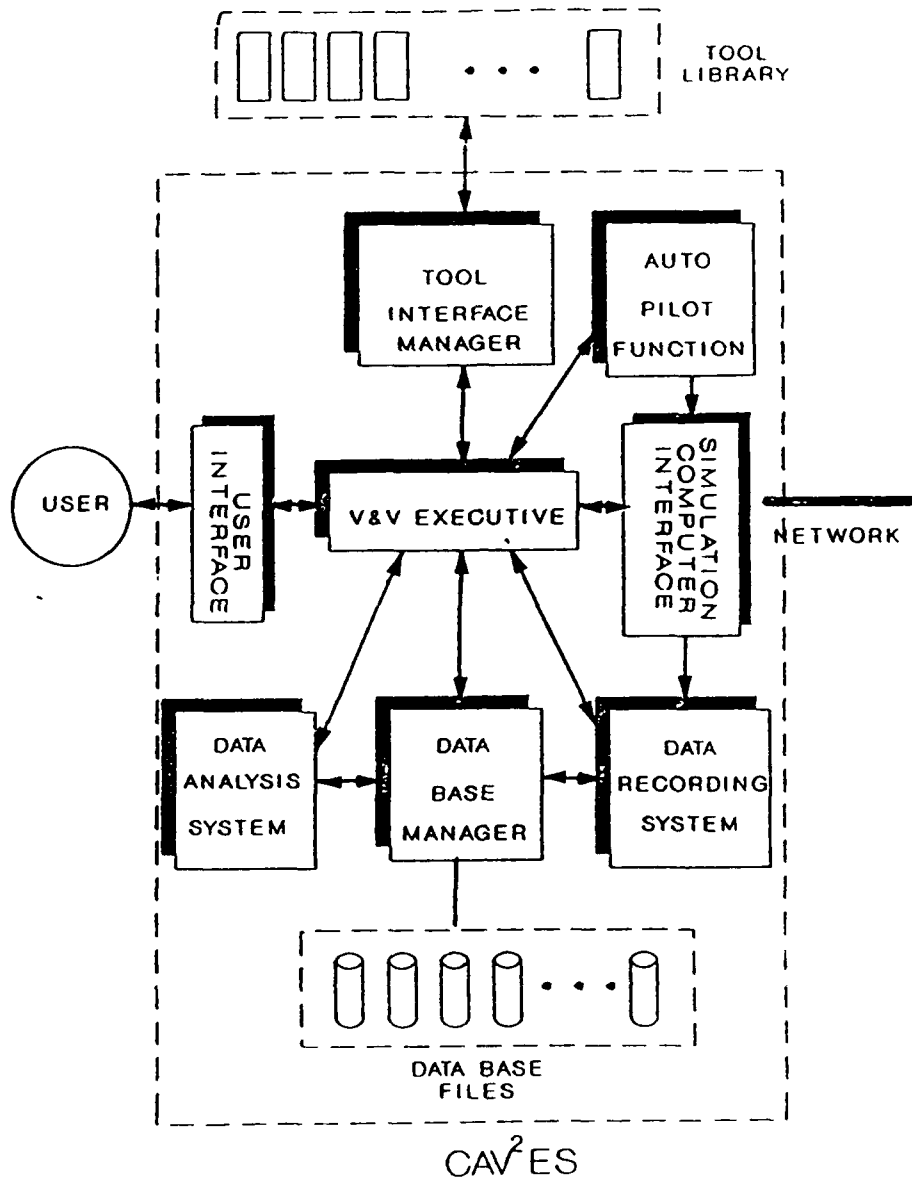
Figure 3.5.2-1 Computer Aided Verification and Validation Engineering System (CAV 2 ES)
