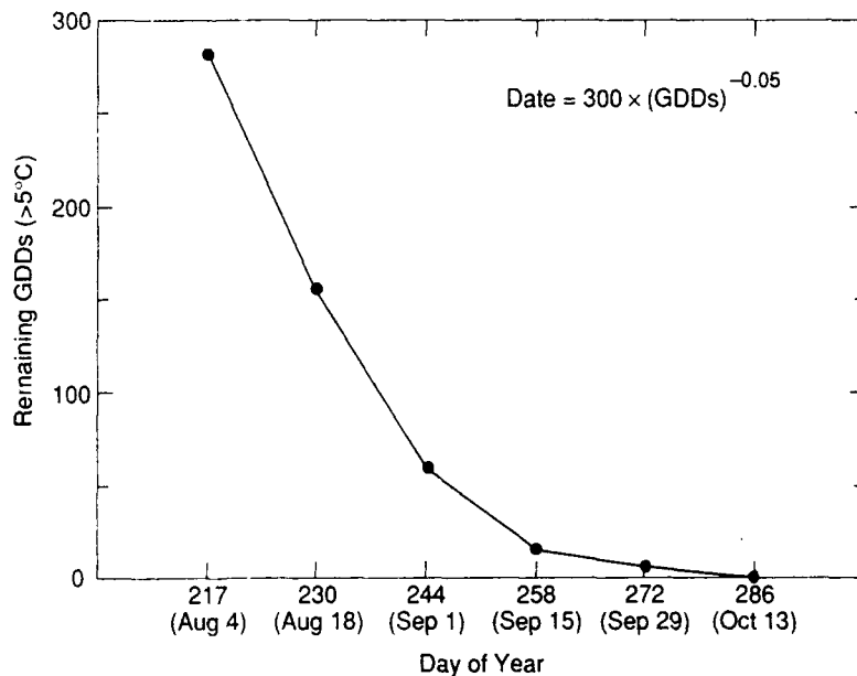
Figure 5. Fall growing degree-day curve for Fairbanks, Alaska, constructed from U.S. Weather Bureau data (daily maximum and minimum air temperatures) from 1986.
