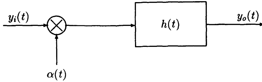
Figure 3.1: Block Diagram of Compressive Receiver Model
