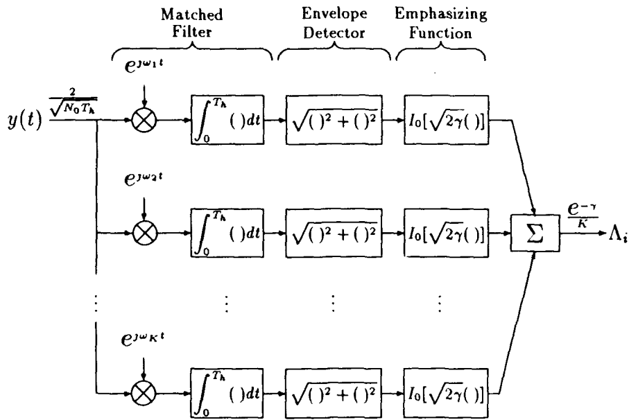
Figure 2.1: Block Diagram of Single-Epoch Likelihood Function
