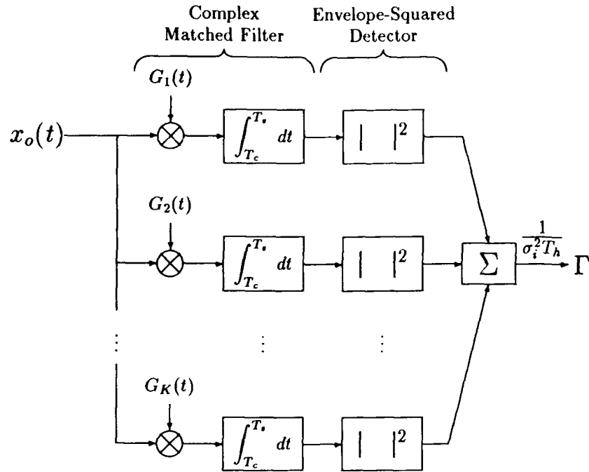
Figure 3.2: Locally Optimal Single-Epoch Detector
