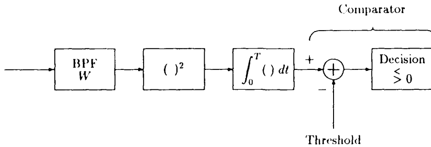
Figure 1.1: Wideband Energy Detector
