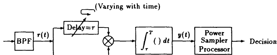
Figure 1.3: Autocorrelation Detector
