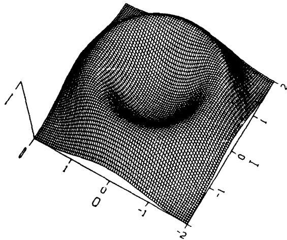
Figure 4.3: Complex adf
