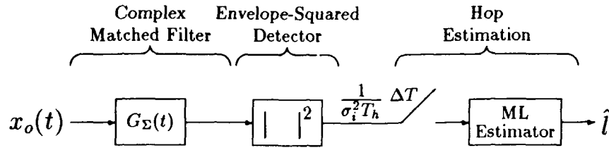
Figure 3.4: Hop Frequency Estimator
