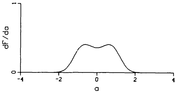
Figure 4.2: The adf of Modulated Sine Wave and Noise
