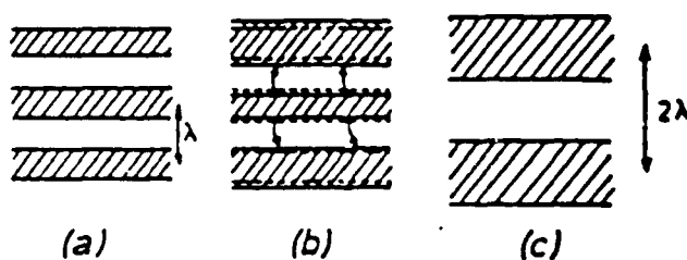
FIGURE 24 Schematic diagram of the coarsening of perfect layers by diffusion-induced doubling (Spaepen, 1985).
