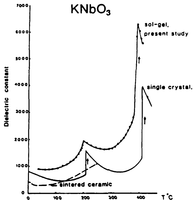
FIGURE 4 Superior properties of sol-gel samples.
