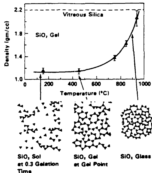
FIGURE 3 Densification microstructures for SiO 2 gels. (Reprinted by permission of the publishers, Butterworth & Co. (Publishers) Ltd.®, from Polymer 28 , 533, D. Ulrich, 1987)
