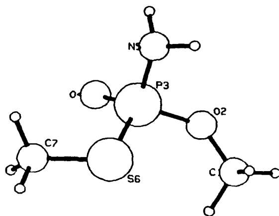
Figure 2. Simulant 1, O-Methyl-S-Methyl : Aminophosphorothiolate
