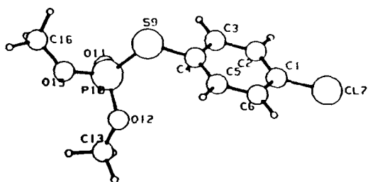
Figure 7. Simulant 6, Bis(O-Methyl)-Chlorophenyl Phosphorothiolate
