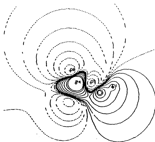
Figure 19. Electrostatic Map/Simulant 7
