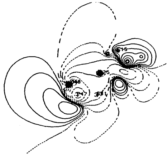
Figure 21. Difference Map/VX and Simulant 2
