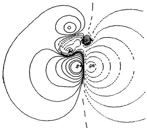
Figure 16. Electrostatic Map/Simulant 4
