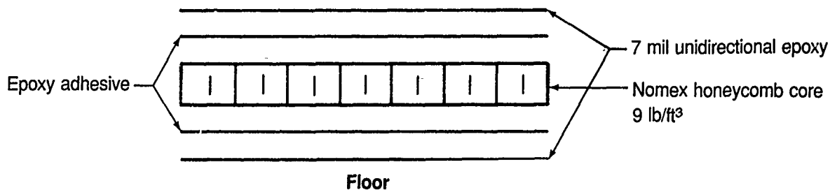
Figure C-2. Typical Panel Installation
