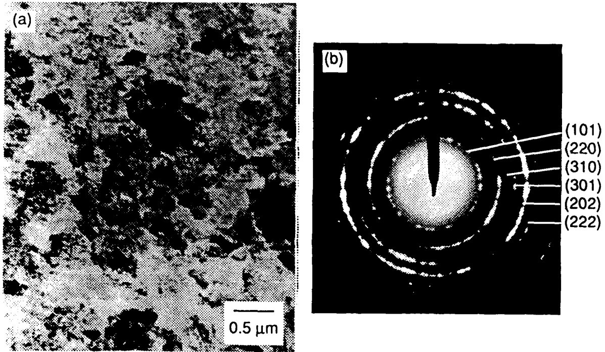
Figure 3. Microstructure of a foil containing 93 at% Be shows a very fine grain size with no evidence of inclusions. Selected area diffraction of the foil shows only the presence of the TiBe_{12} phase.
