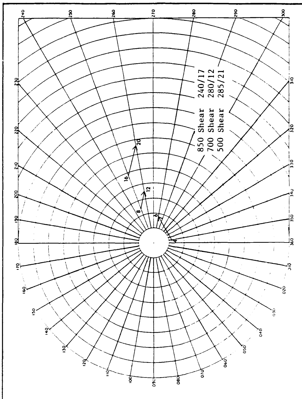
FIG. III-C-2b Shear vectors for the 850 mb, 700 mb, and 500 mb maps for D3-1800 LST for Station #3.
