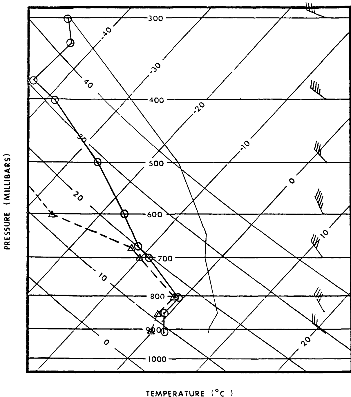
FIG. III-B-5 Dodge City, KS 72451 DDC for 1200 GMT 03 April 1984. The sounding shows cooling from the previous 24 h trace (the thin line to the right of the sounding). Note the cooling is deep, extending above the 400 mb level. The tropopause is at 376 mb. The lapse rate of the sounding is close to the wet adiabatic lapse rate. The mP air is above the 800 mb level, and the potential temperature at the bottom of the mP air is 16° C. Some colder air, probably cP is in the lower level. This is a typical mP front passage.
