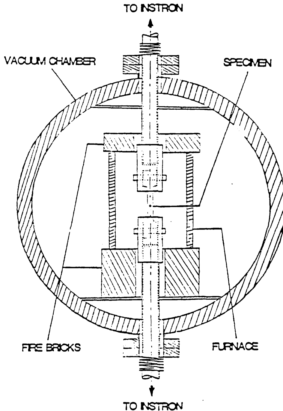
FIG 3: A SCHEMATIC OF THE HIGH TEMPERATURE VACUUM CHAMBER USED FOR THE TENSILE TEST.
