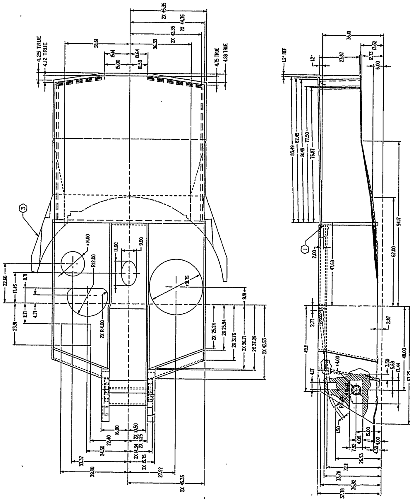
FIG 2 TURRET GEOMETRY 12
