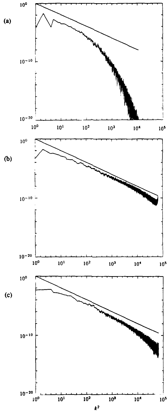
Fig. 10 — Autocorrelation spectra (log of magnitude squared) vs. log of squared wavenumber for (a) Mass density, \tau = 1.0 , (b) Mass density, \tau = 2.0 , (c) Mass density, \tau = 4.0 , (d) Velocity, \tau = 2.0 , (e) Nonsolenoidal component of the velocity, \tau = 2.0 , (f) Solenoidal component of the velocity, \tau = 2.0 , (g) magnetic field, \tau = 2.0 .
