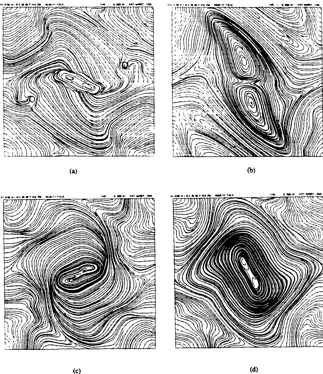
Fig. 6 — Plots of the generalized stream function for M = 1.0 and S = 50 giving direction of velocity ((a) and (c)) and magnetic field ((b) and (d)) at respective times t = 3.0 and 7.0 .
