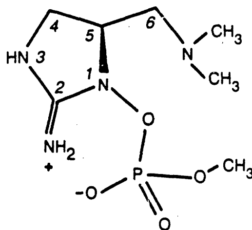
anatoxin - a(s) (m/z 252) C 7 H 17 N 4 O 4 P
