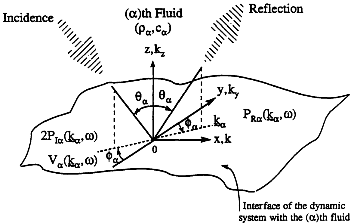
Fig. 4. Incident pressure P_{I\alpha}(k_\alpha, \omega) , specularly reflected pressure P_{R\alpha}(k_\alpha, \omega) , and velocity V_\alpha(k_\alpha, \omega) on the interface between the (\alpha) th fluid and the plane dynamic system.
