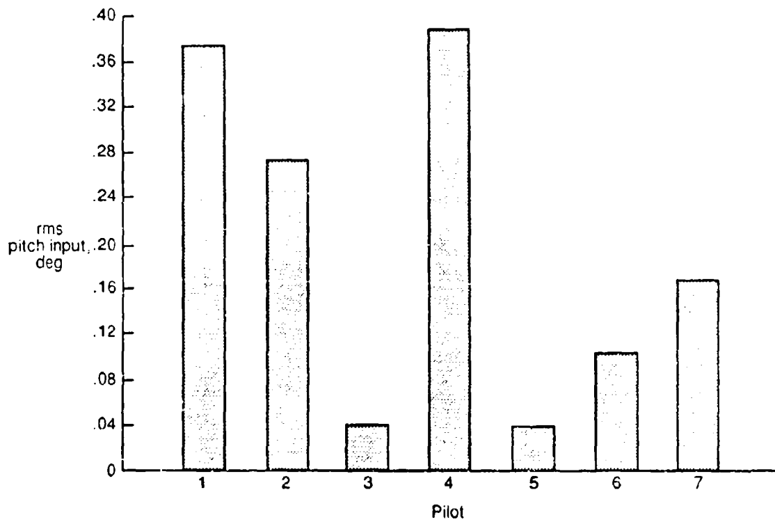
Figure 23. Mean rms pitch input for each pilot.
