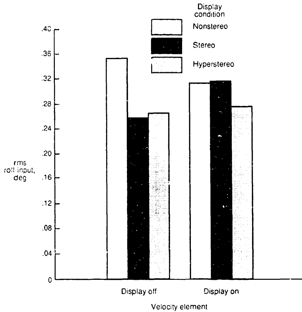
Figure 59. Mean rms roll input for each display condition with velocity display element "on" and "off."
