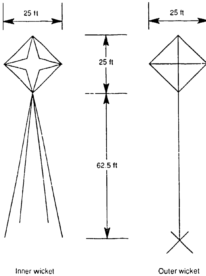
Figure 1. Diagram of inner and outer wickets.
