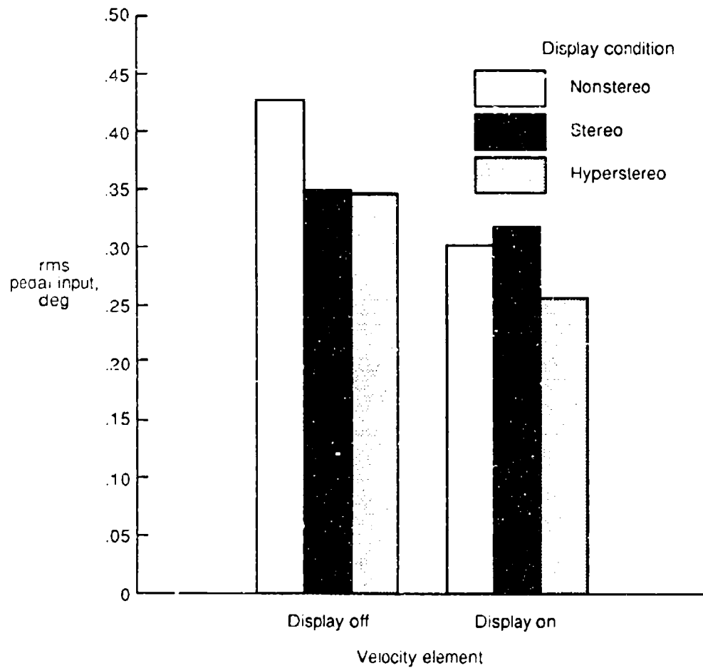
Figure 36. Mean rms pedal input for each display condition with velocity display element "on" and "off."
