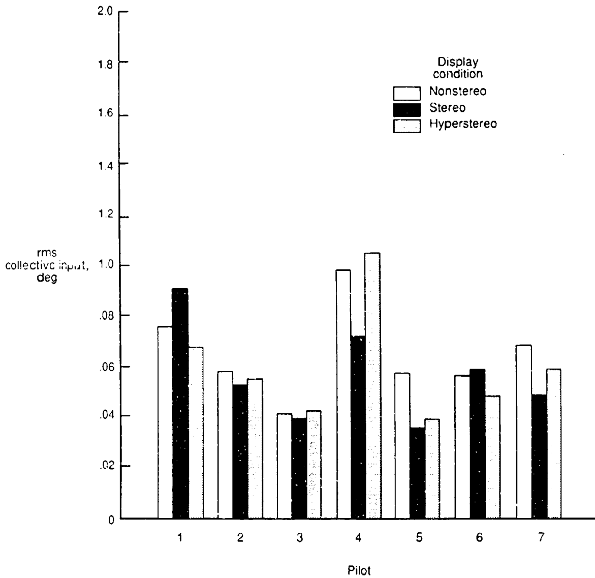
Figure 40. Mean rms collective input for each pilot across display conditions.
