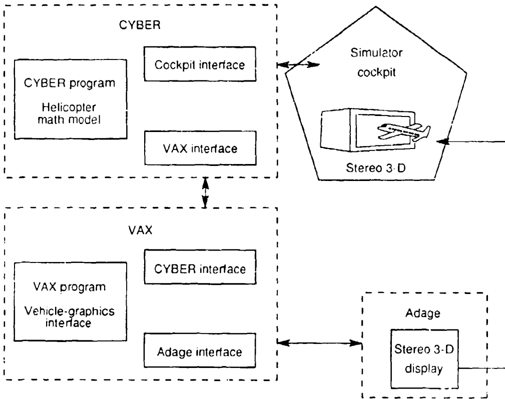
Figure 8. Three-stage computer pipeline used in study.
