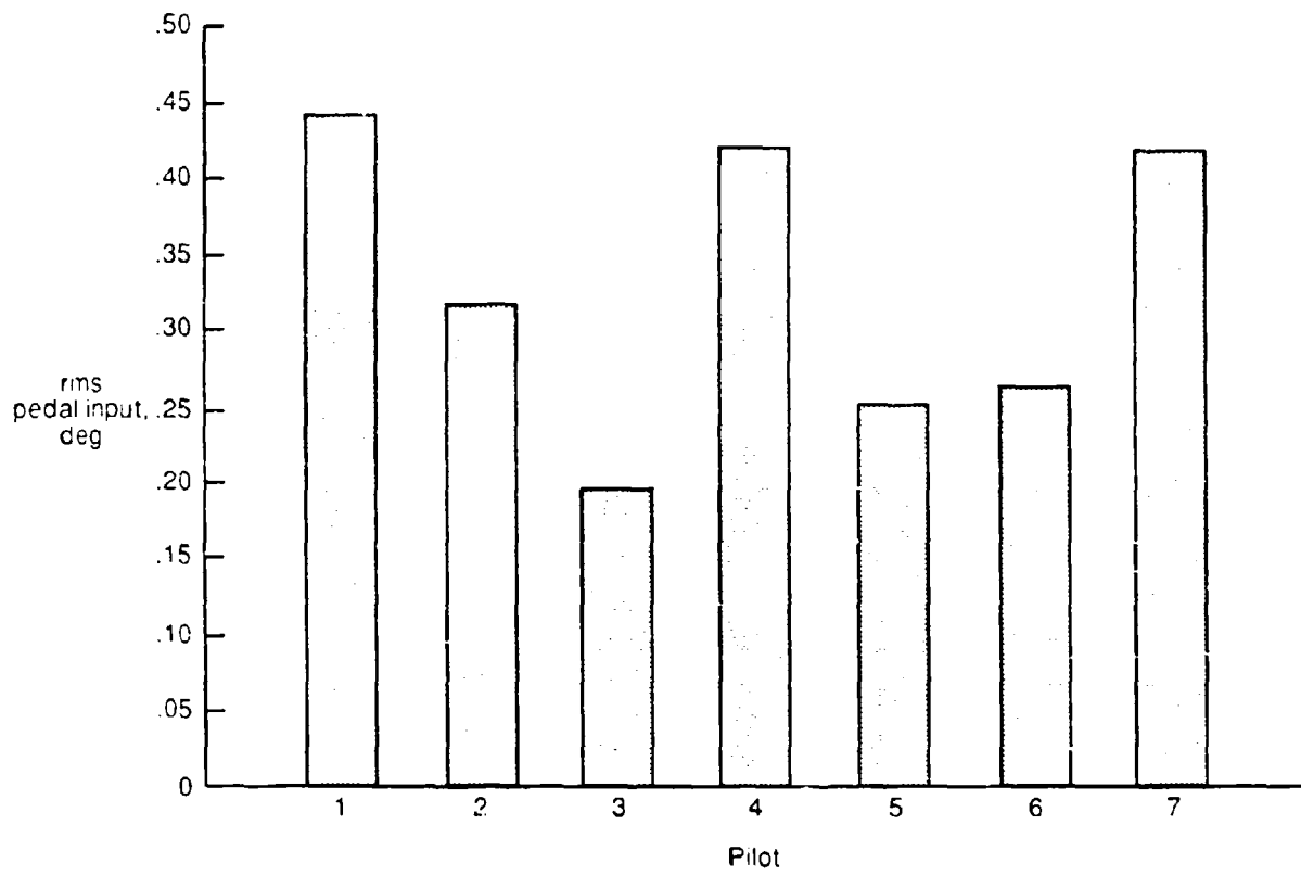
Figure 31. Mean rms pedal input for each pilot.
