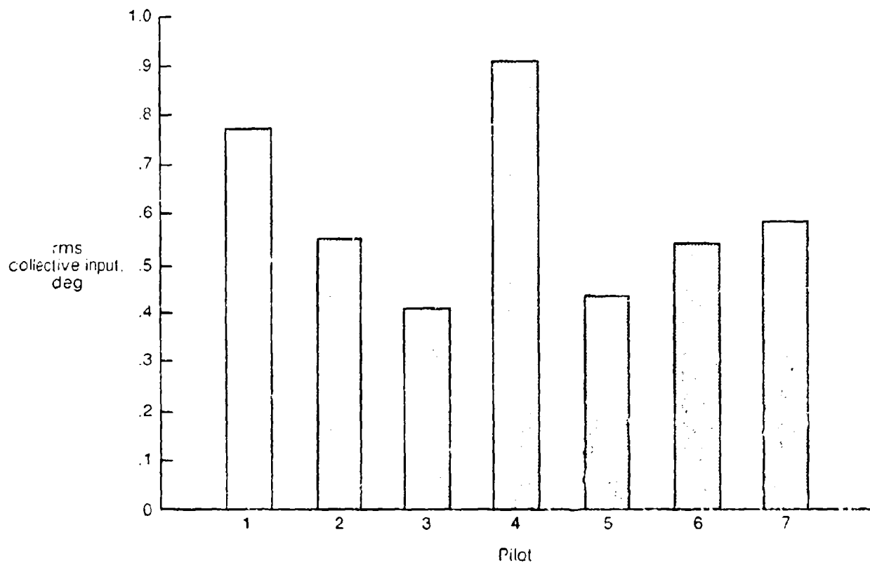
Figure 38. Mean rms collective input for each pilot.
