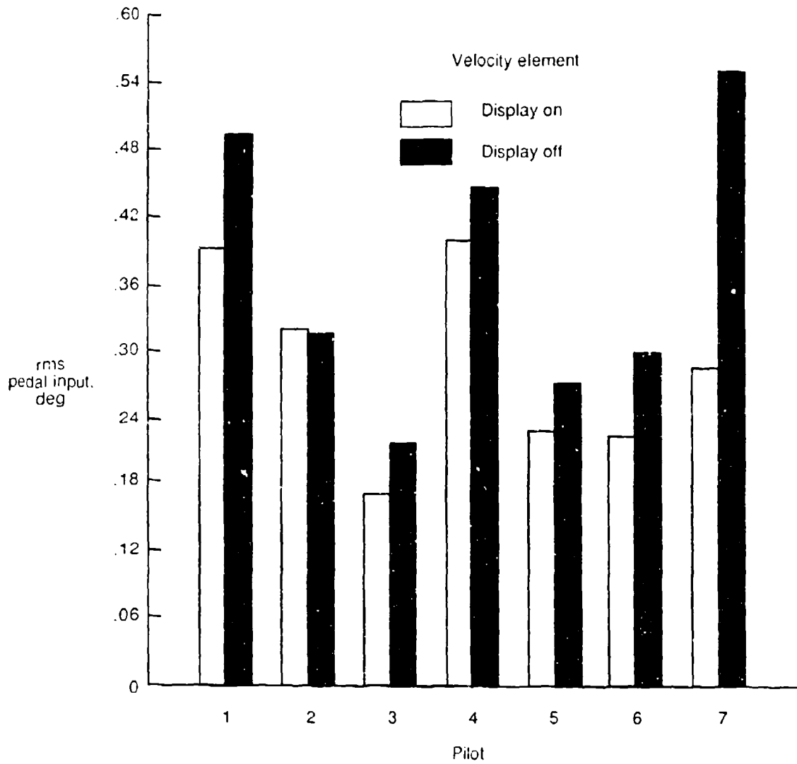
Figure 35. Mean rms pedal input for each pilot with velocity display element "on" and "off."
