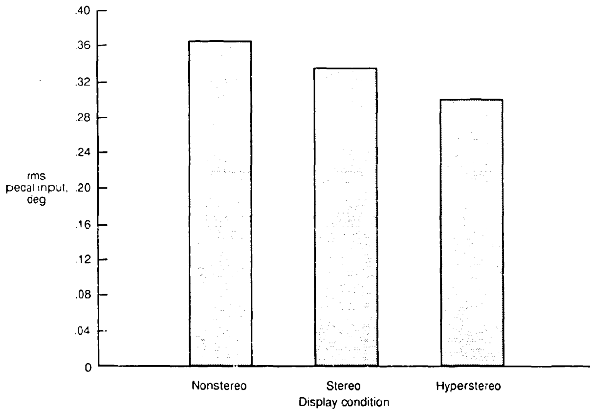
Figure 32. Mean rms pedal input for each display condition.
