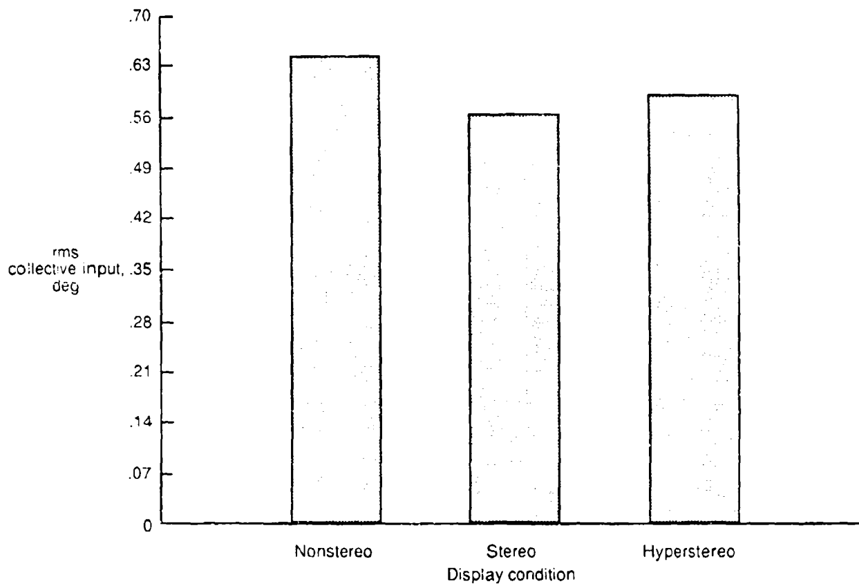
Figure 39. Mean rms collective input for each display condition.
