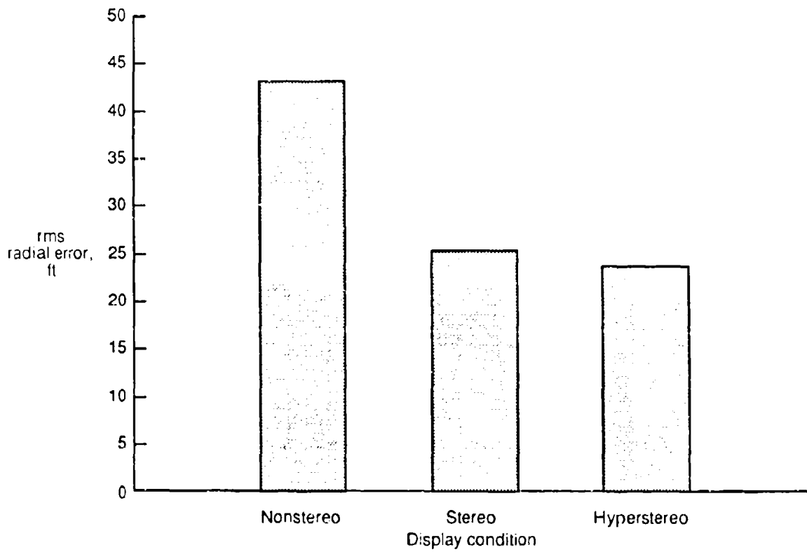
Figure 13. Mean rms radial error for each display condition (all pilots).
