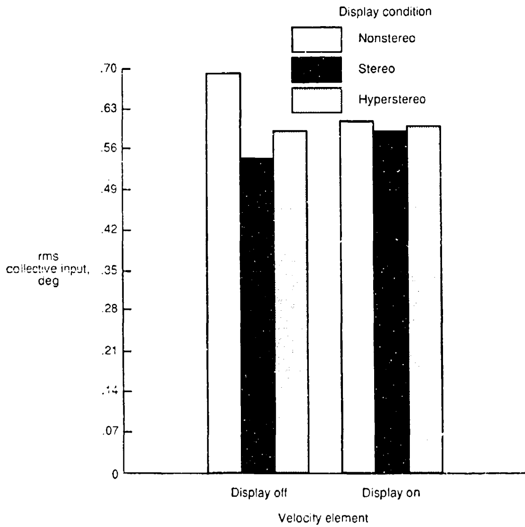
Figure 41. Mean rms collective input for each display condition with velocity display element "on" and "off."
