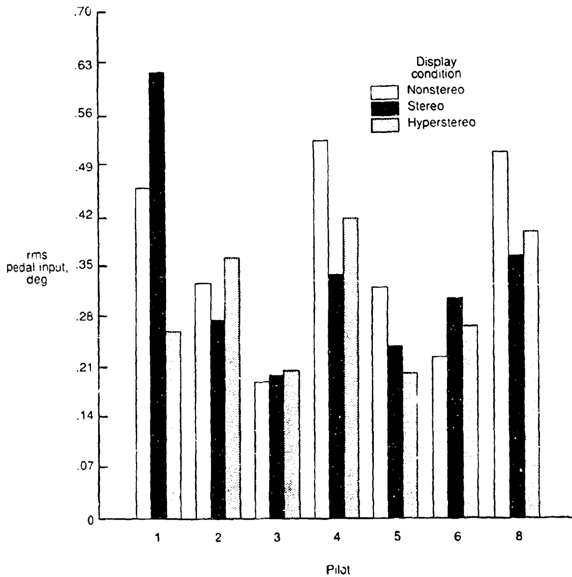
Figure 33. Mean rms pedal input for each pilot across display conditions.
