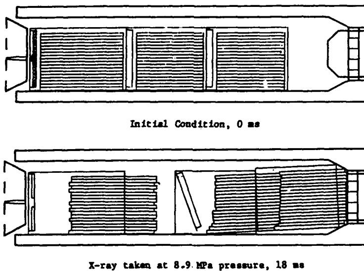
Figure 11. Schematic of X-ray, XM216 Propelling Charge, Zone 4, 63 °C, Round 41002
