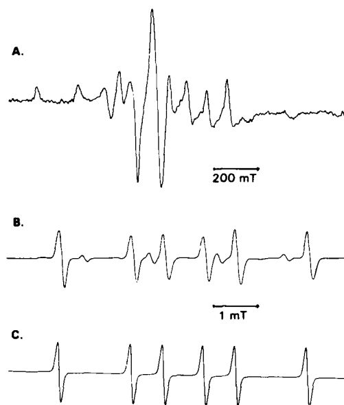
Fig. 2. (A) ESR spectrum of \text{VO}^{2+} ( 1 \times 10^{-3} M) bound to RNA ( 1 \times 10^{-3} M) in the presence of DMPO (0.1 M). (B) ESR spectrum of DMPO-hydroxyethyl adduct following reaction of mixture in (A) with \text{H}_2\text{O}_2 ( 1 \times 10^{-3} M) in the presence of ethanol (1.7 M). (C) Computer simulation of ESR spectrum in (B). Instrument receiver gain was set at: 2 \times 10^4 and 2.5 \times 10^3 for (A) and (B), respectively.
