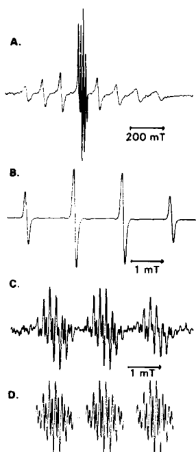
Fig. 1. (A) ESR spectrum of \text{VOSO}_4 ( 1 \times 10^{-3} M) following its reaction with \text{H}_2\text{O}_2 ( 1 \times 10^{-3} M) in the presence of DMPO (0.1 M). (B) DMPO-OH ESR spectrum observed in the center region of (A) after reducing the instrument microwave power, modulation amplitude and scan range. (C) ESR spectrum of the MNP-histidyl adduct from the reaction of \text{VOSO}_4 with \text{H}_2\text{O}_2 (same concentrations as in (A)) in the presence of histidine ( 1 \times 10^{-3} M) and MNP ( 2.5 \times 10^{-2} M). (D) Computer simulation of the ESR spectrum in (C). Instrument receiver gain was set at: 1.25 \times 10^4 , 2 \times 10^3 and 1.6 \times 10^5 for (A), (B) and (C), respectively. The time constant and scan time for (C) were 2 s and 30 min, respectively.
