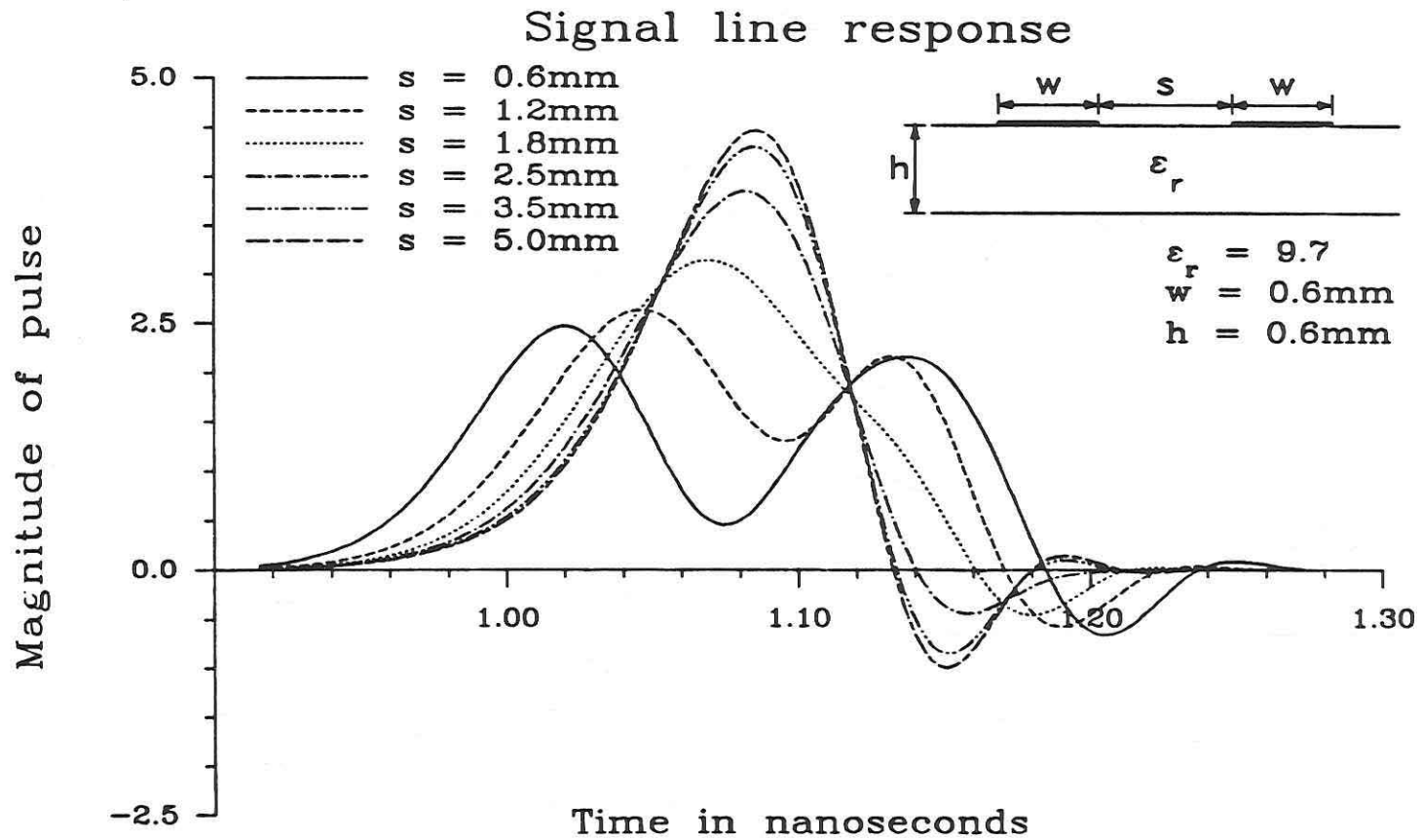
Fig. 4.23. Pulse distortion on coupled lines vs. spacing, signal line response l = 125\text{mm} , \tau = 30\text{ps} , alumina substrate.
