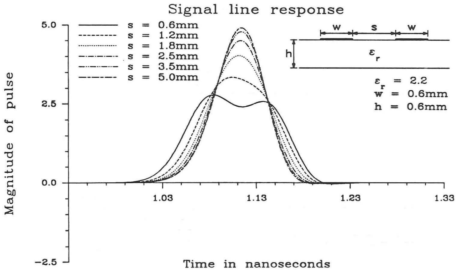
Fig. 4.19. Pulse distortion on coupled lines vs. spacing, signal line response l = 250\text{mm} , \tau = 30\text{ps} , RT/duroid 5880 substrate.
