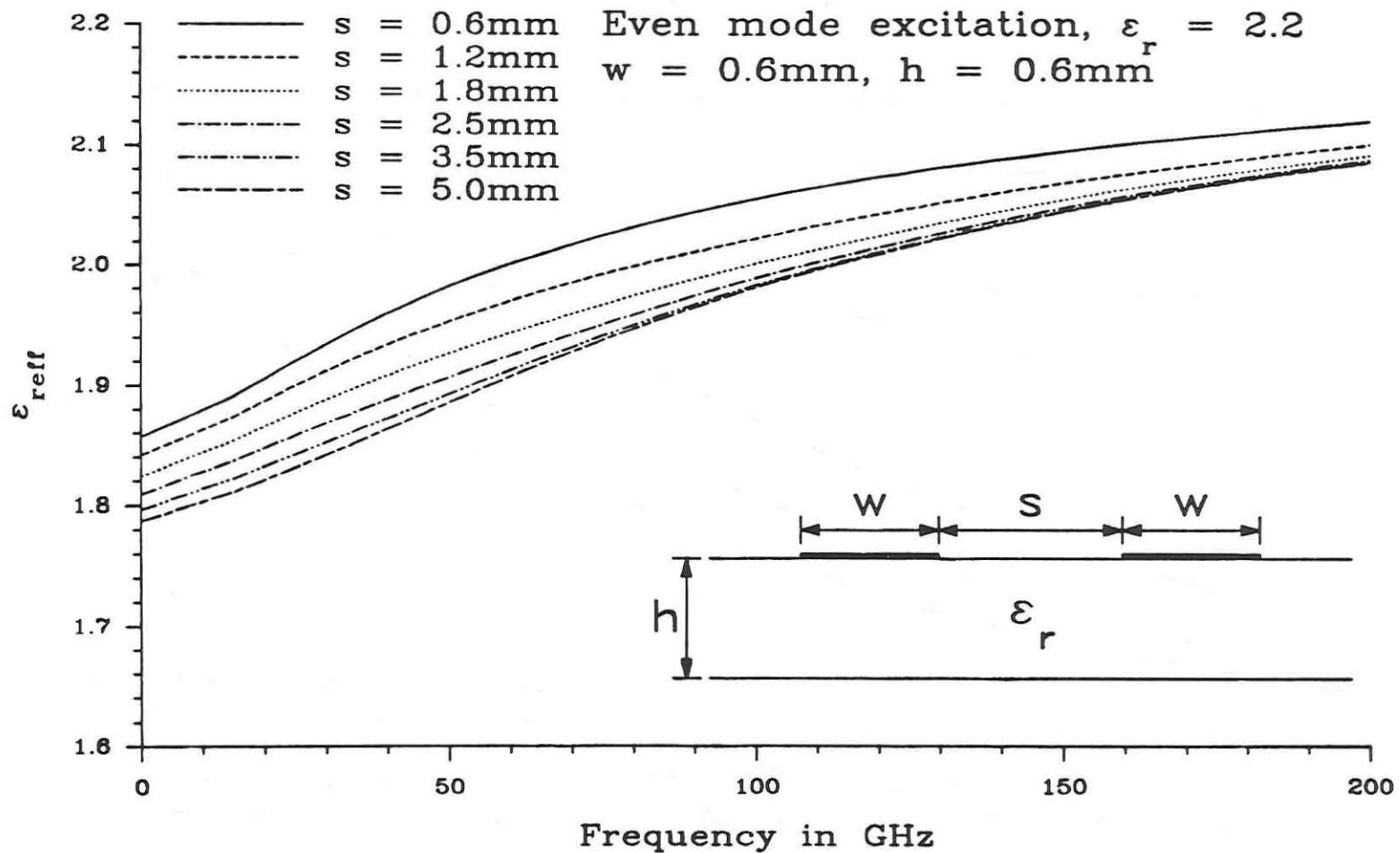
Fig. 4.1. \epsilon_{\text{reff}} vs. frequency for open symmetric coupled microstrips on RT/duroid 5880 substrate, even mode.
