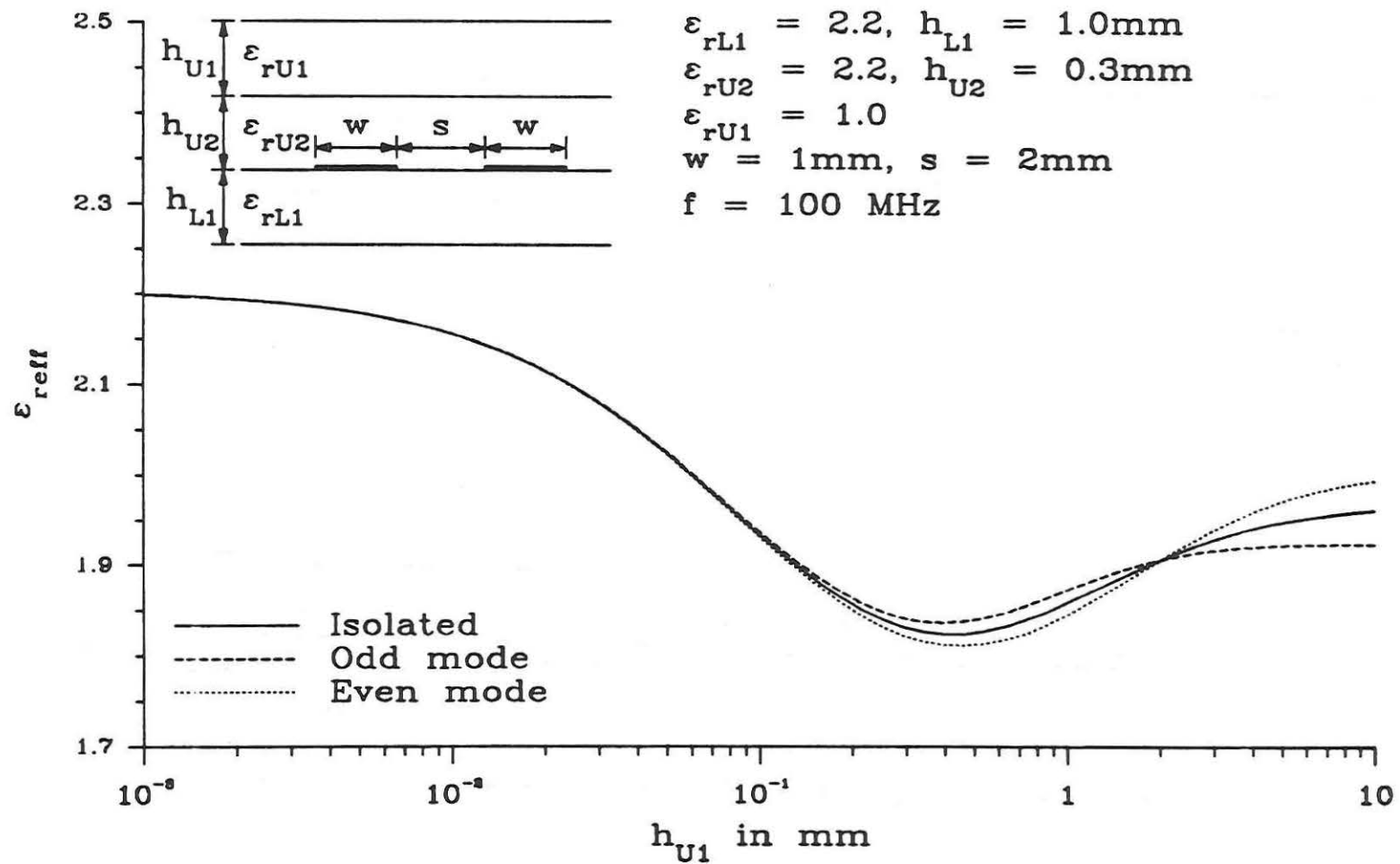
Fig. 4.35. \epsilon_{reff} vs. cover sheet height for multilayer symmetric coupled microstrips with RT/duroid 5880 superstrate and substrate.
