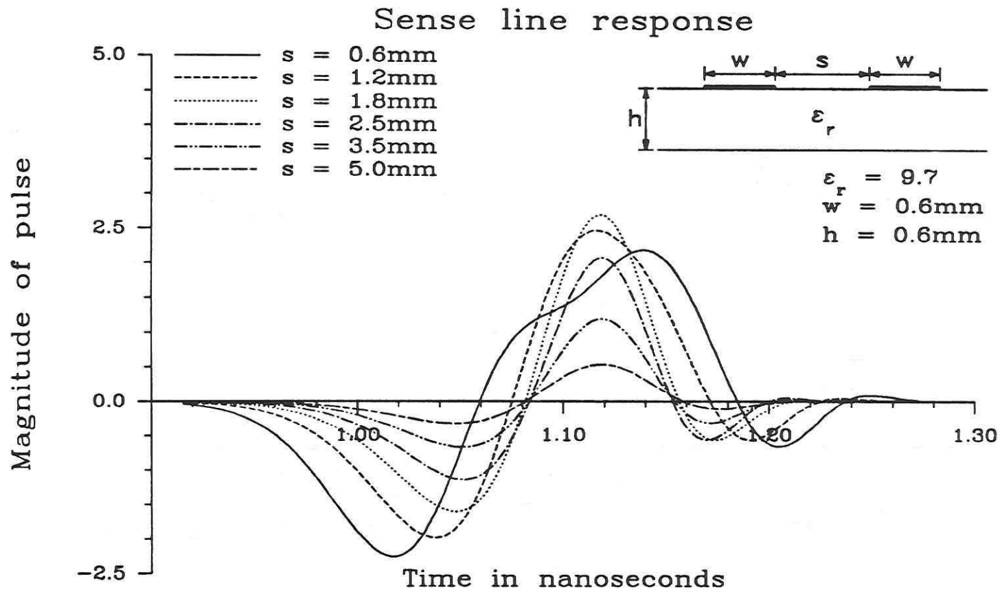
Fig. 4.24. Pulse distortion on coupled lines vs. spacing, sense line response l = 125\text{mm} , \tau = 30\text{ps} , alumina substrate.
