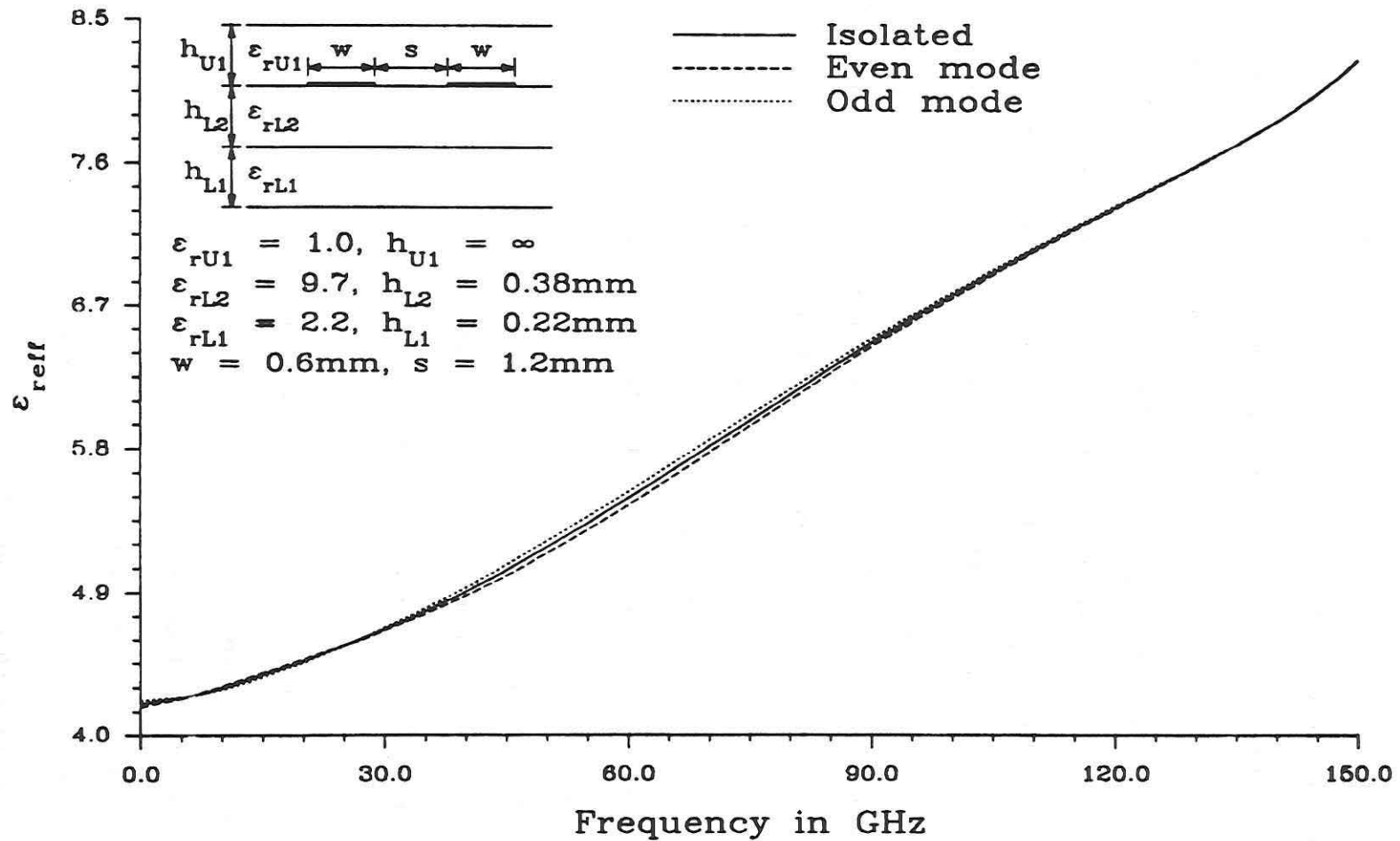
Fig. 4.49. \epsilon_{\text{reff}} vs. frequency for low coupling structure using alumina and RT/duriod 5880 substrates.
