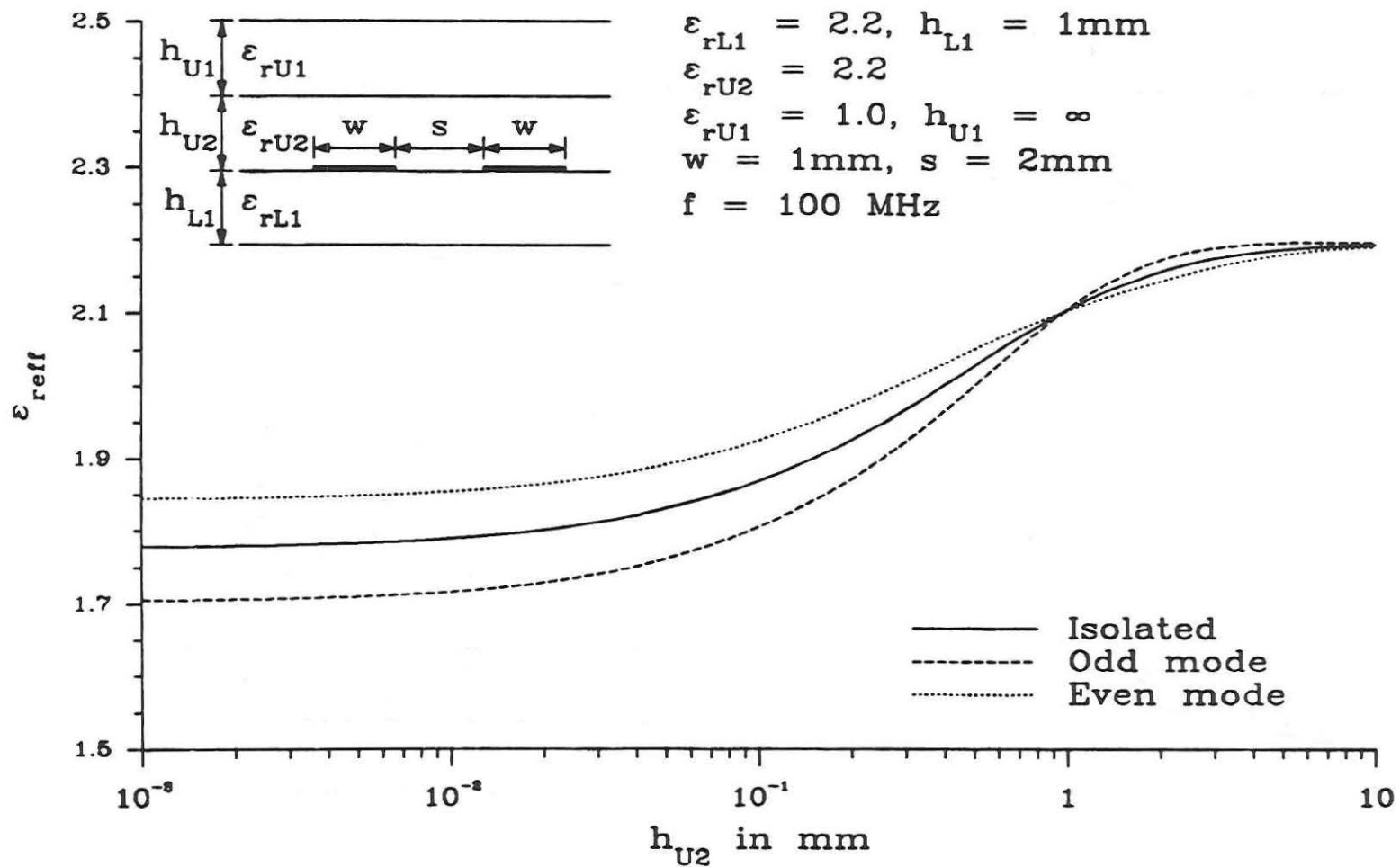
Fig. 4.31. \epsilon_{reff} vs. cover layer height for multilayer symmetric coupled microstrips with RT/duroid 5880 superstrate and substrate.
