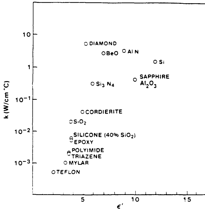
Figure 4-1. Thermal conductivity-dielectric constant relationship of dielectric layer and encapsulation materials.
