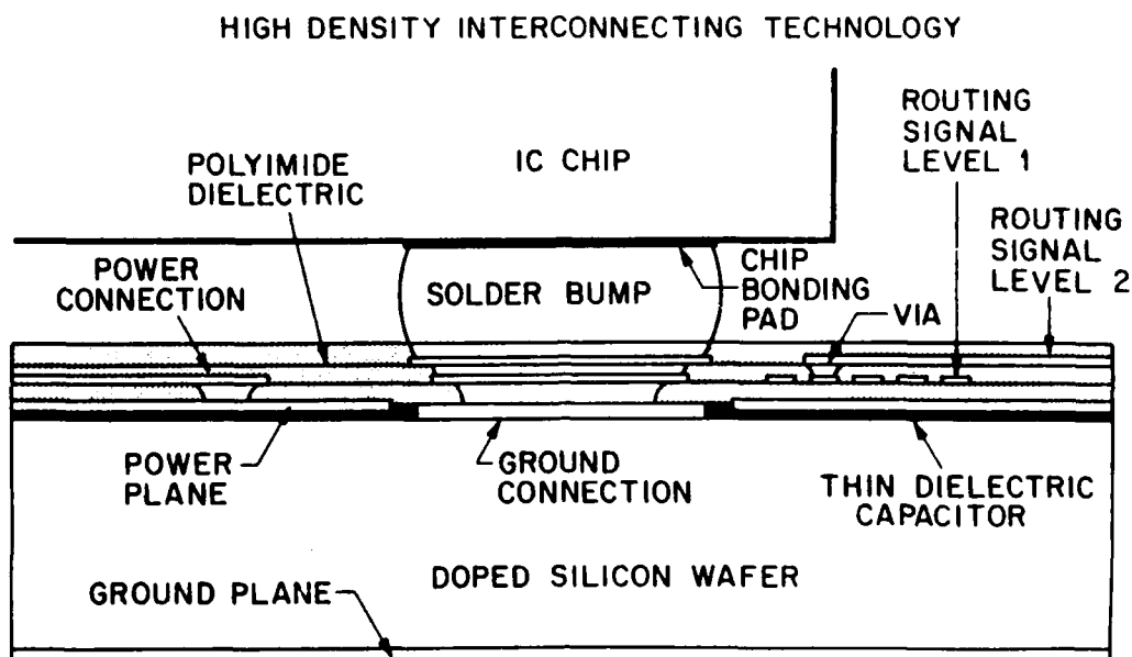
FIGURE 3-1 Cross-sectional view of AT&T AVP module.
