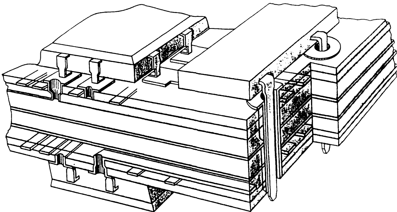
FIGURE 1-7 Printed wiring board circuit shown in cutaway to reveal inner connector layers and vias. A surface-mount device (left) and a through-hole device (right) are illustrated. Note that surface-mount devices can be mounted on both sides of the board (as shown) and do not consume valuable inner layer space with the through-hole.
