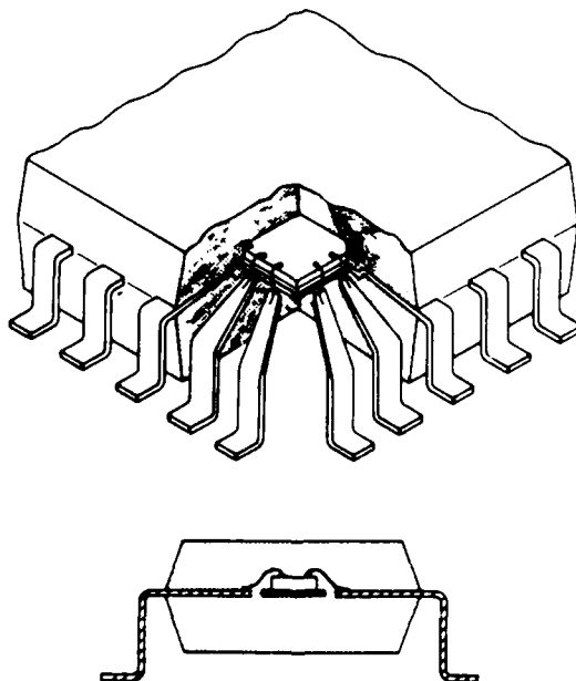
FIGURE 1-3 Molded plastic quad design or plastic leaded chip carrier (PLCC). The chip is die-bonded to the paddle, which is connected to one or more ground leads. Signal, power, ground, and timing leads are connected by wire bonding pads. (A TAB inner lead frame can be used for this purpose.)
