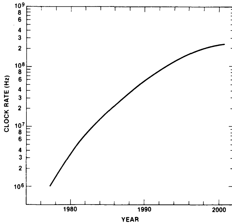
Figure C-4 Microprocessor clock rate: history and forecast.
