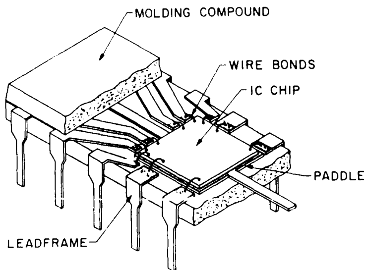
FIGURE 1-1 Cutaway view of a plastic DIP.
