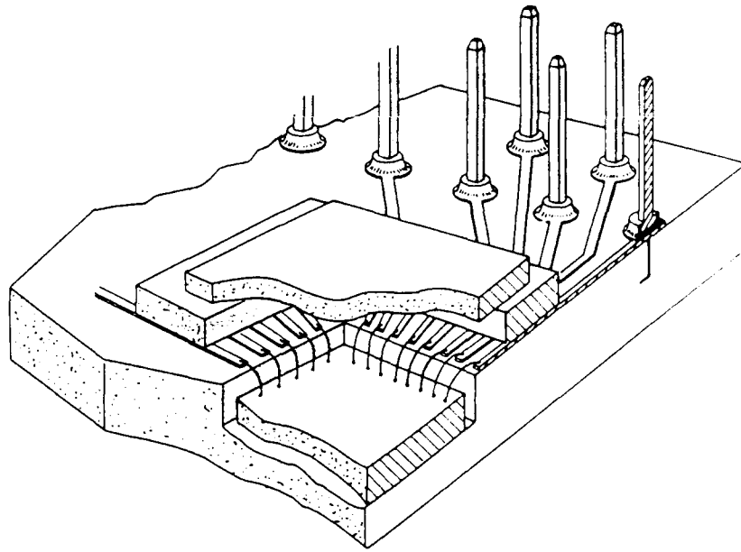
FIGURE 1-4 Cutaway of a PGA. The chip is die-bonded in the ceramic cavity and wire-bonded to the conductor fan-out, which is plated onto the ceramic. The outer end of each fanout finger is terminated onto a brazen pin, which is inserted into a through-hole on the PWB. This package can then be sealed hermetically with a lid (ceramic or metal). Similar packages with surface-mount leads are also employed. The device is shown inverted, and in use the active side of the chip would face the PWB (face down). The pins can be made to exit the ceramic on the opposite side (face up). The face-down option shown offers a favorable surface for heat-sink attachment.
