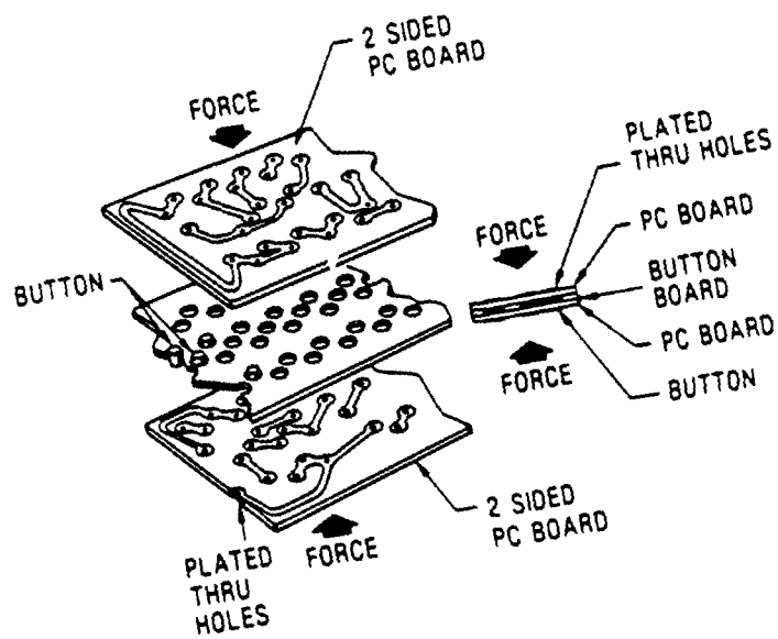
Figure D-1 Circuit assembly employing button board technology for face-to-face interconnection of modules. (Courtesy of TRW)
