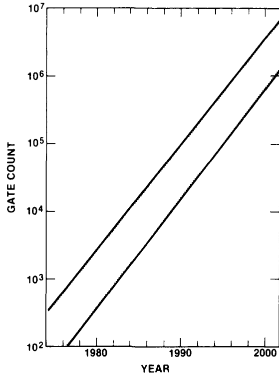
Figure C-3 Microprocessor gate count: history and forecast.
