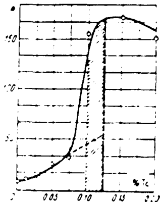
Fig. 1. Dependence of number of grains n , which fall on 1 \text{ cm}^2 of area of large section, from % additive, tantalum; shaded region corresponds to beginning of precipitation of crystals of compound TaAl.
