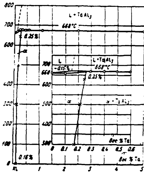
Fig. 8. Constitution diagram aluminum-tantalum (within it is represented angle of diagram on increased scale): o - data of thermal analysis, x - data of X-ray diffraction analysis. Key: (1). Weight % Ta.
