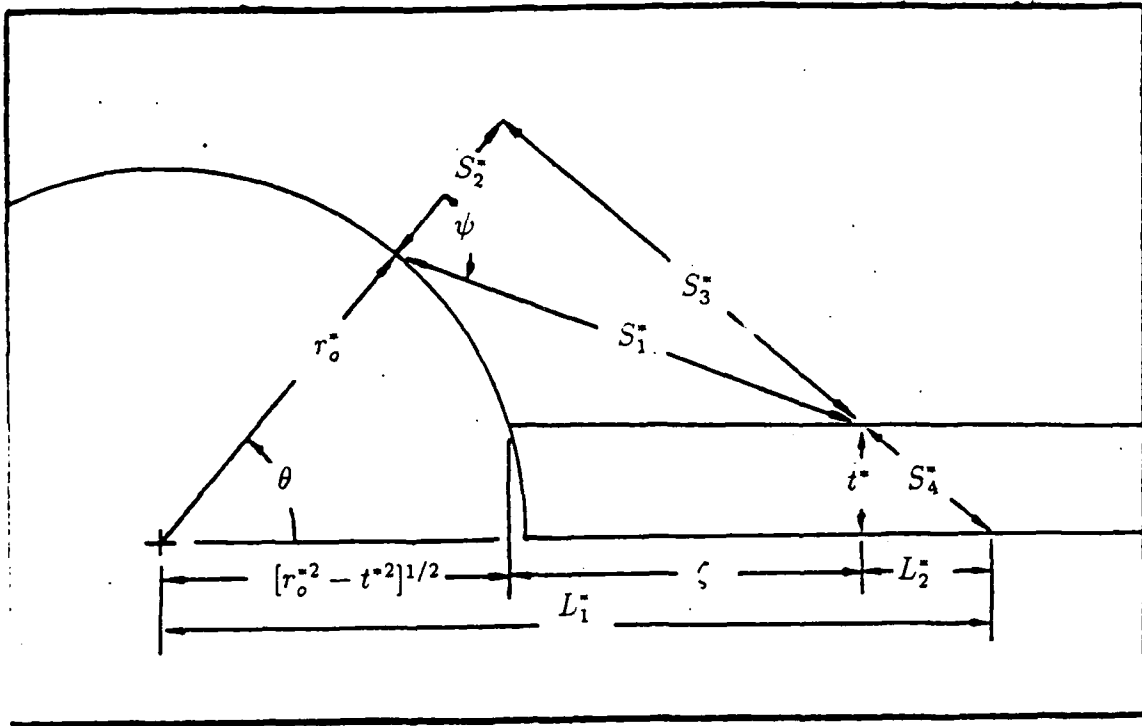
Figure B.1. Geometry Used in Fin-to-Heatpipe View Factor Determination
