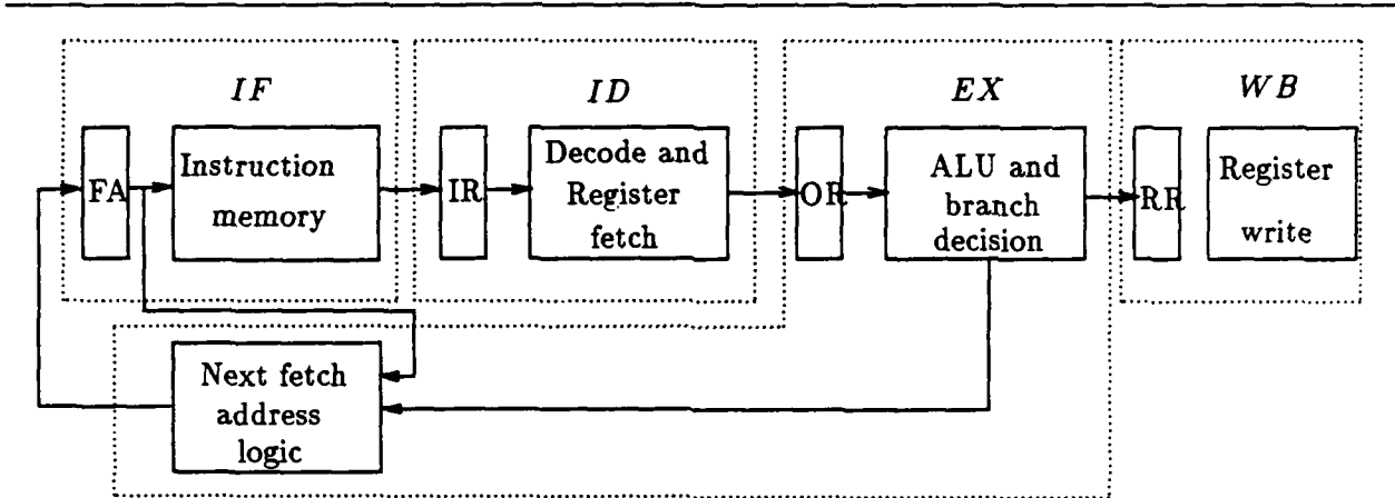
Figure 3: A block diagram and a simplified view of a pipelined processor. FA, IR, OR, RR are pipeline registers Fetch Address , Instruction Register , Operand Register , and Result Register .
