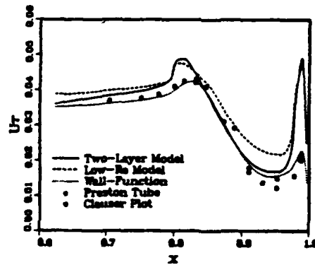
Fig.VI-33. Friction Velocity Distribution for Afterbody-5 Given in Ref.[56]
