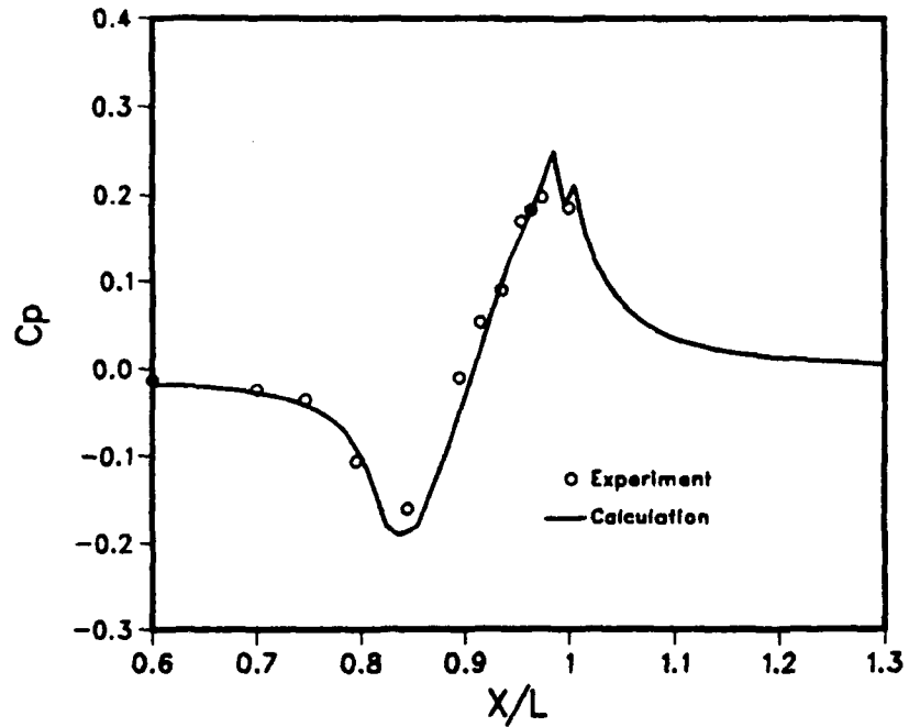
Fig.VII-5. Surface Pressure Distribution ( Afterbody-2 )
