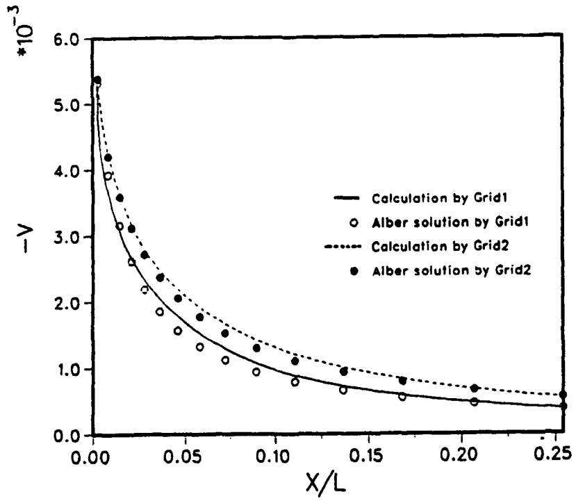
Fig.IV-11. Near-Wake Normal Velocity Distributions
