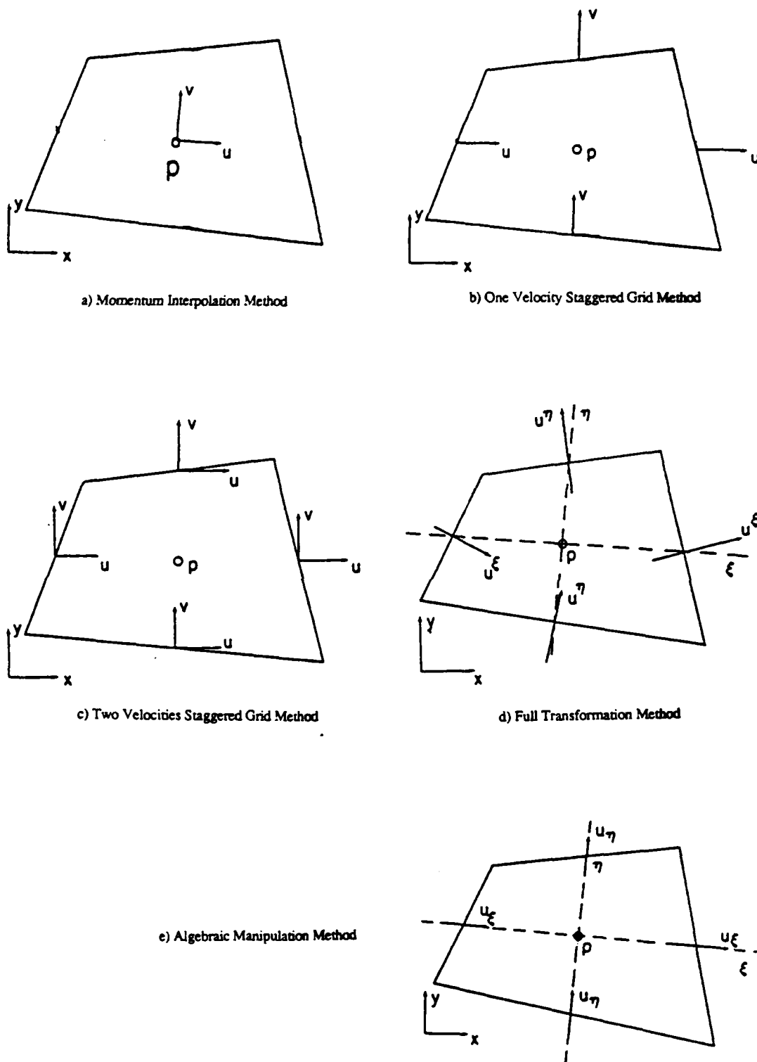
Fig.I-1. Grid Configurations.
