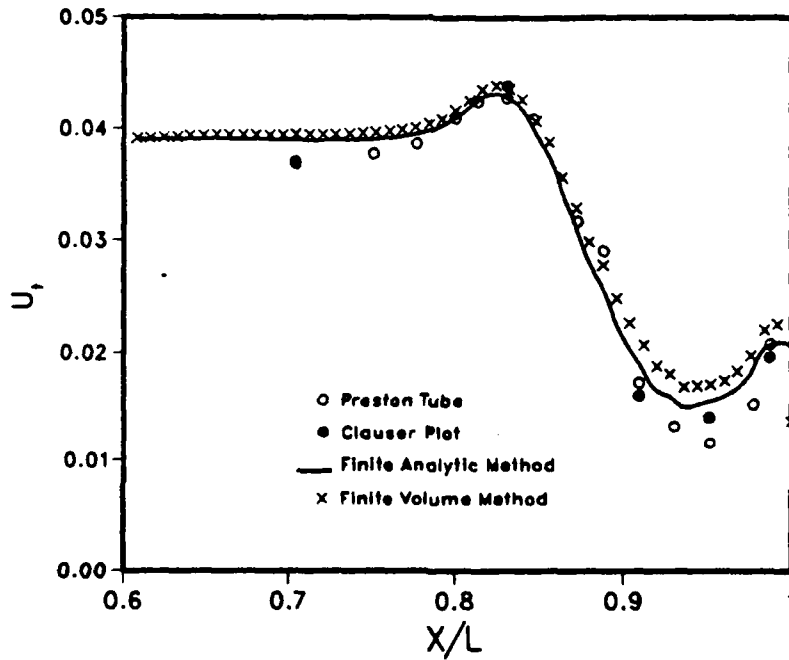
Fig.VI-14. Friction Velocity Distribution ( Afterbody-5 )
