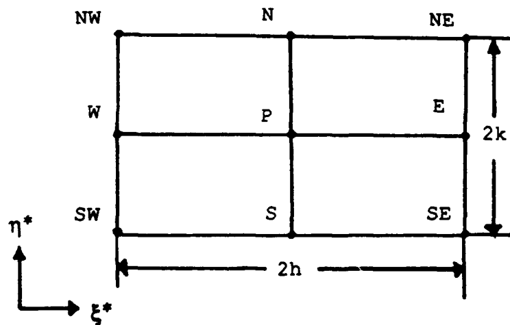
Fig.II-7. A Local Element for Finite Analytic Method in Boundary-Fitted Coordinate System
