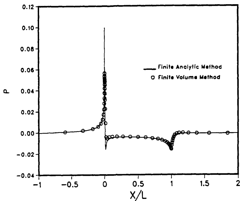
Fig.V-1. Pressure Distribution ( Laminar Flow )
