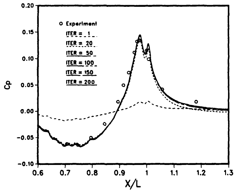
Fig. VI-4. Pressure Convergence History ( Finite Volume Method )
