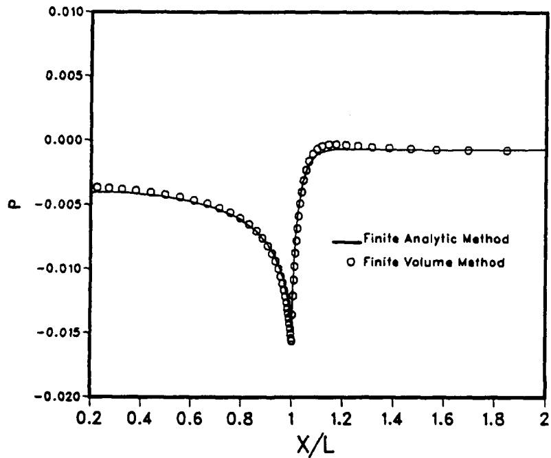
Fig.V-2. Pressure Distribution near the Trailing Edge ( Laminar Flow )
