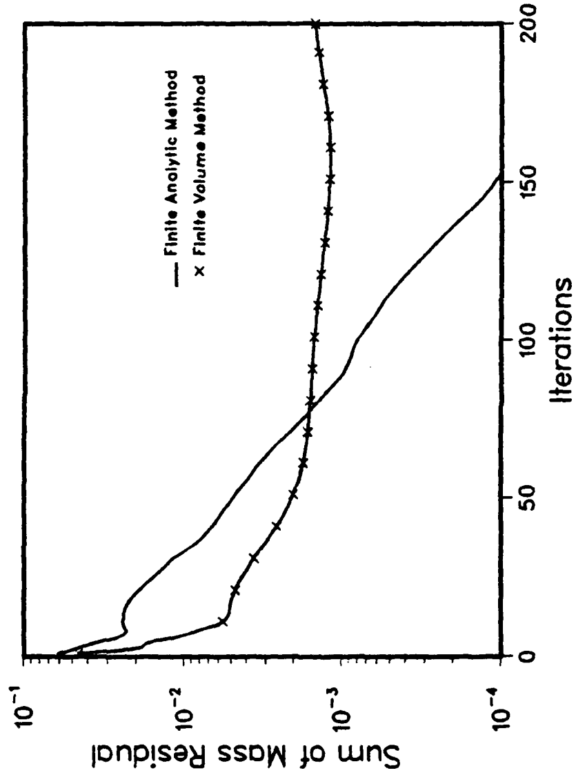
Fig. VI-2. Convergence History
