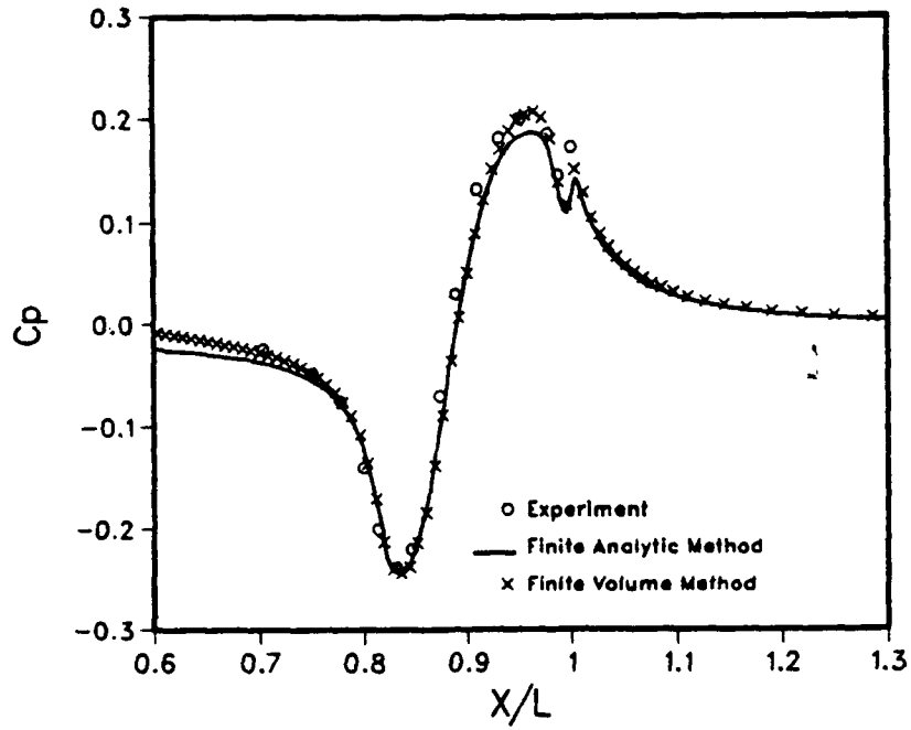
Fig.VI-11. Surface Pressure Distribution ( Afterbody-5 )
