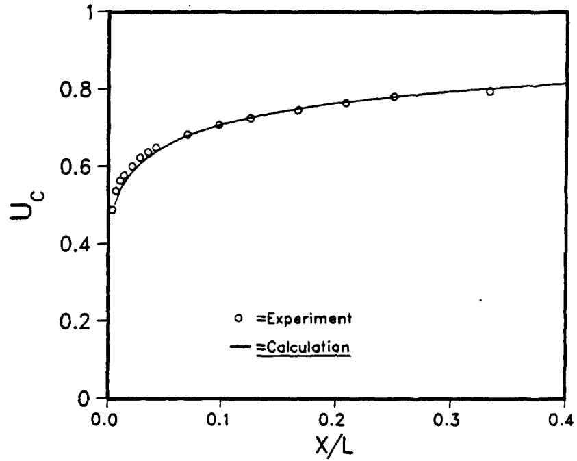
Fig. IV-6. Wake Centerline Velocity Distribution
