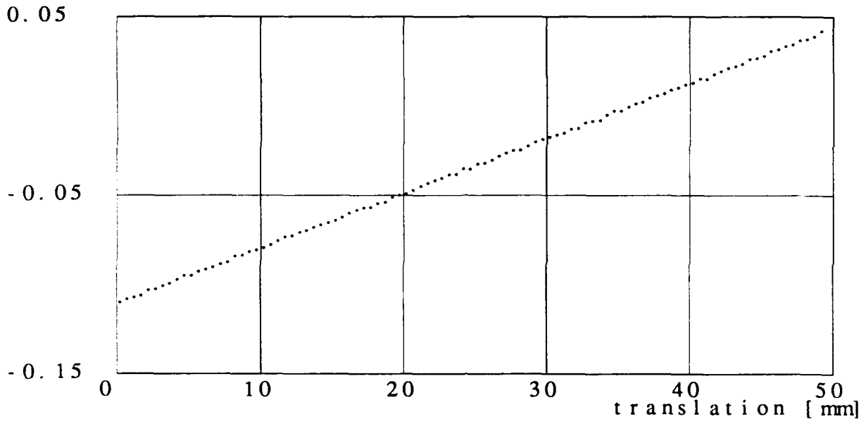
Figure 7: Photodiode resolution
