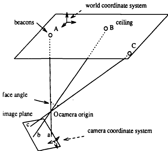
Figure 2: Church's algorithm
