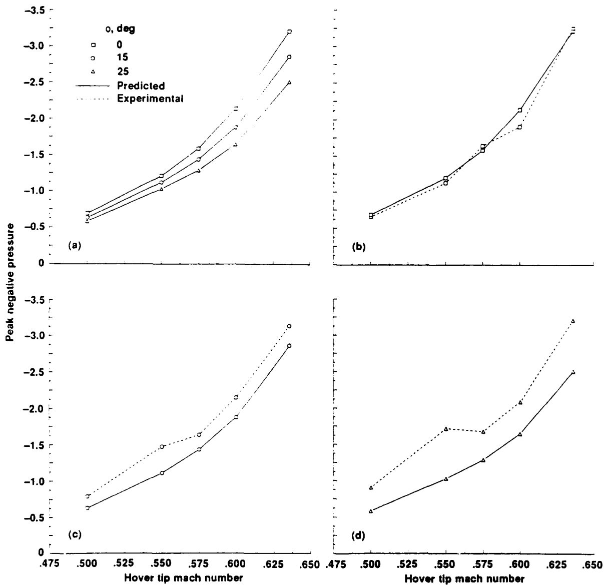
Figure 3. Plots of peak negative acoustic pressure versus mach number. (a) Depicts predicted trends. (b) Shows comparisons for inplane microphones, \phi = 0 . (c) Shows comparisons for microphones at \phi = 15^\circ below the tip path plane. (d) Shows comparisons for microphones at \phi = 25^\circ below the tip path plane.
