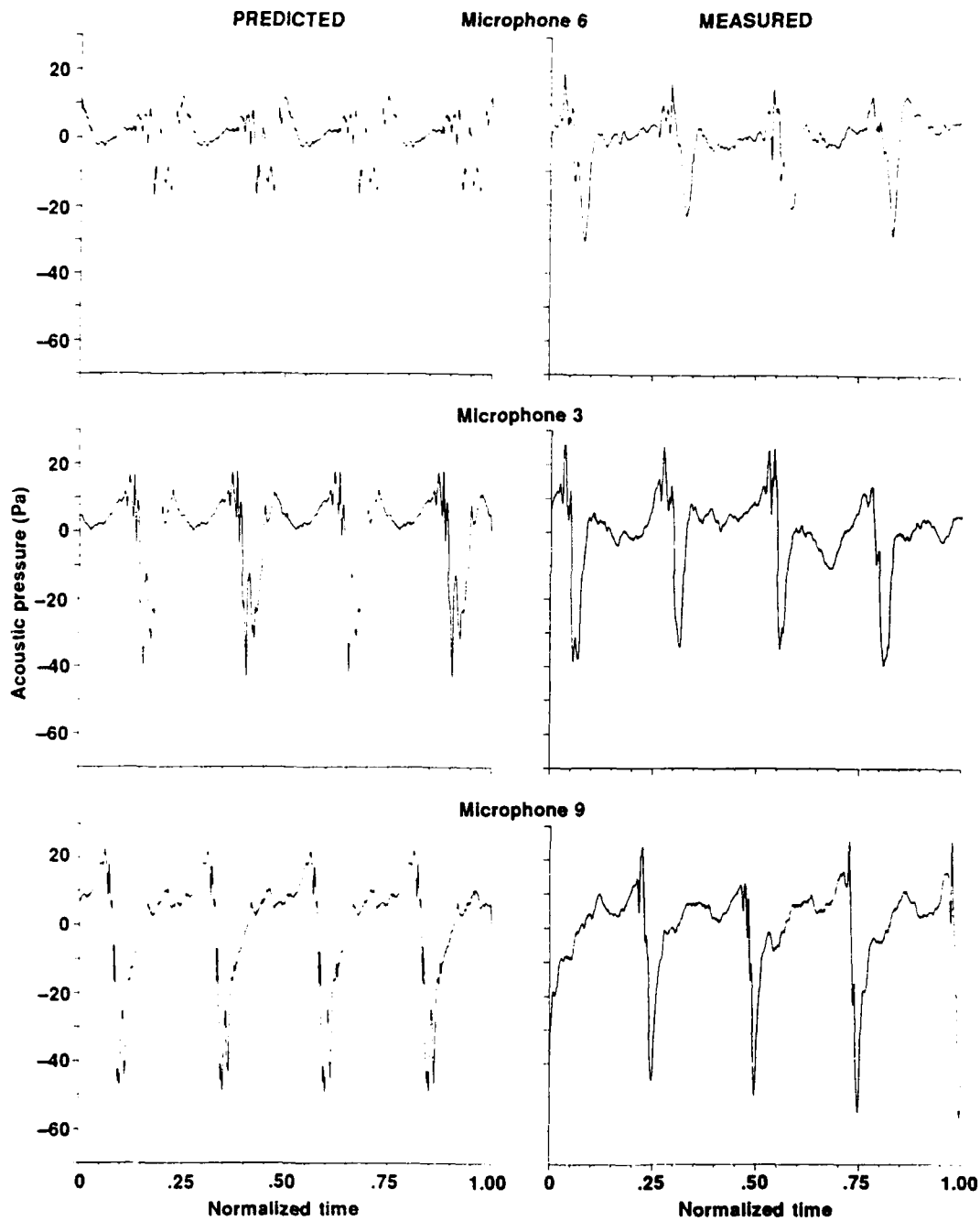
Figure 4b. Plots of acoustic pressure time histories for microphones 25° below the tip path plane. The flight conditions are \mu = 0.356 , CT/\alpha = 0.07 , and shaft tilt = 5.55°
