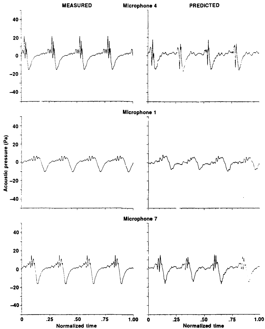
Figure 5a. Plots of acoustic pressure time histories for microphones in the tip path plane. The flight conditions are \mu = 0.225 , CT/\alpha = 0.07 , and shaft tilt = 4.38^\circ .
