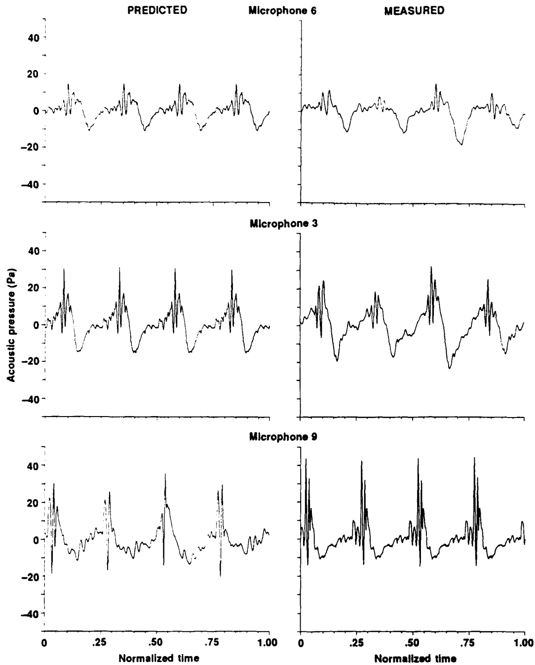
Figure 5b. Plots of acoustic pressure time histories for microphones 25° below the tip path plane. The flight conditions are \mu = 0.225 , CT/\alpha = 0.07 , and shaft tilt = 4.38°.
