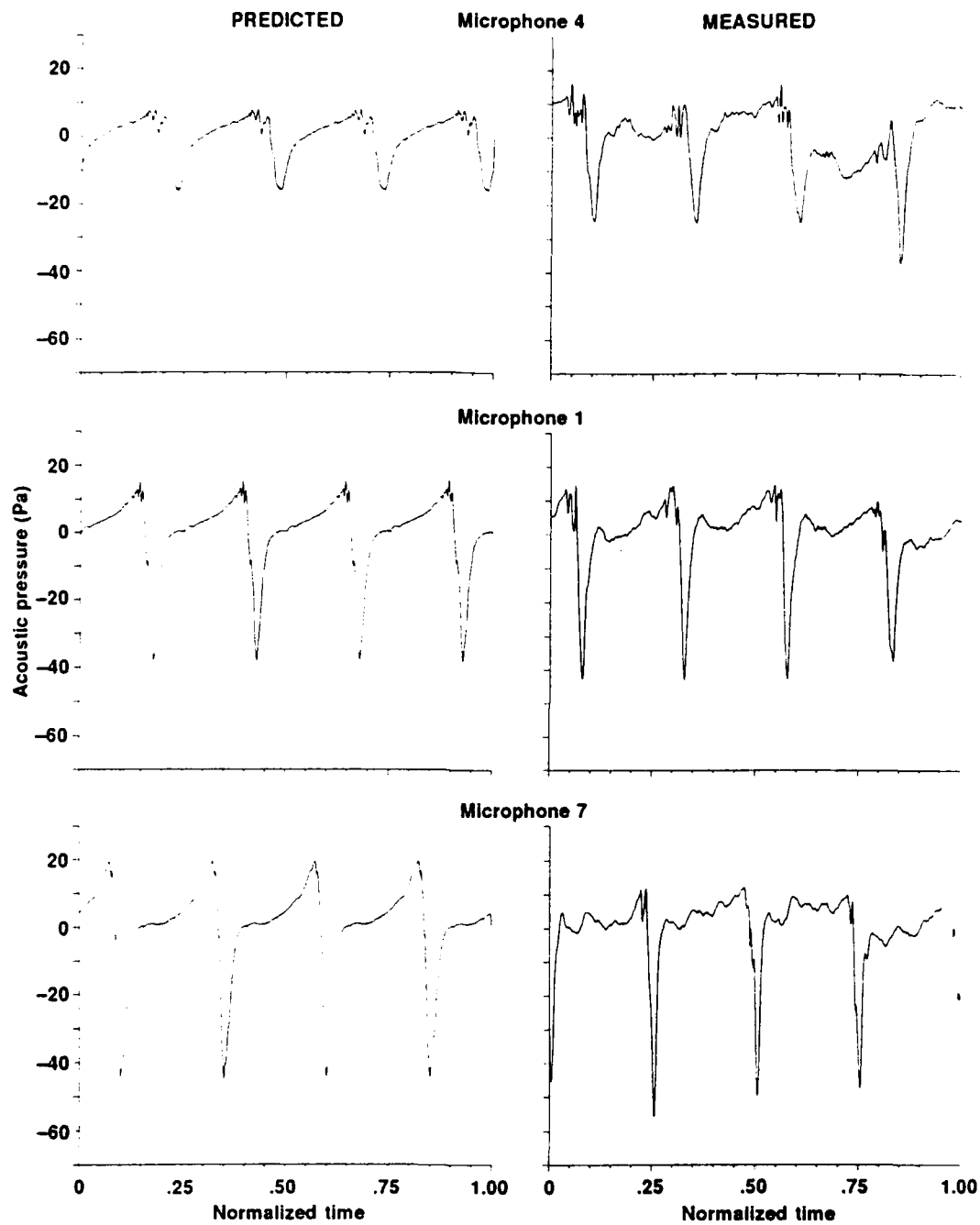
Figure 4a. Plots of acoustic pressure time histories for microphones in the tip path plane. The flight conditions are \mu = 0.356 , CT/\alpha = 0.07 , and shaft tilt = -5.55^\circ .
