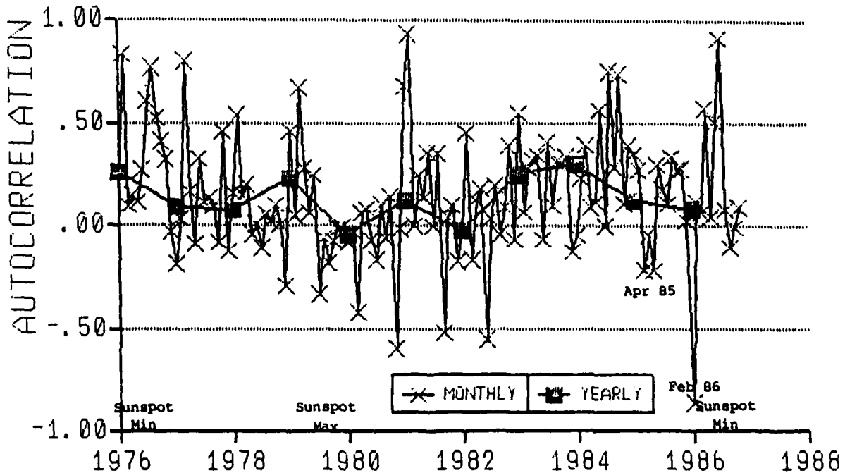
Figure 2-11. Monthly and yearly plots of 27-day lag autocorrelation coefficients.
