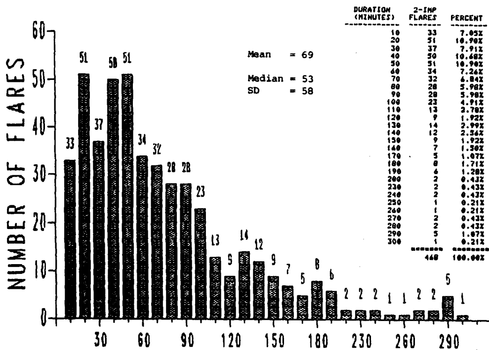
Figure 1-17. Number of "2-importance" flares categorized by duration in 10 minute intervals (1-10, 11-20, 21-30, etc.). Inset table gives duration, number of flares, and percent of total. Mean, median, and standard deviation (SD) are also shown.
