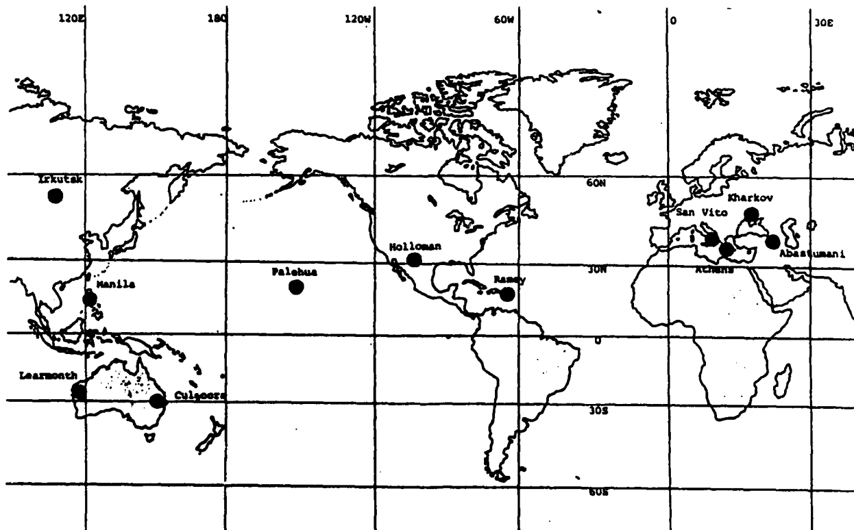
Figure 1-1. Location of optical observatories in the database for Solar Cycle 21.
