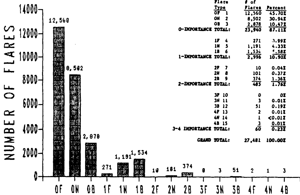
Figure 1-5. Total number of flare reports for each flare type. This figure gives flare type distribution for the entire 11-year POR. The inset table gives a number for each flare type and the percent of the total.
