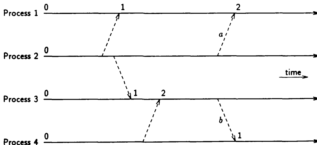
Figure 1 The system history partial order
