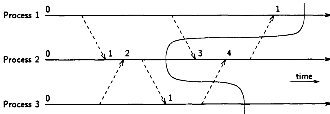
Figure 2 An inconsistent system state
