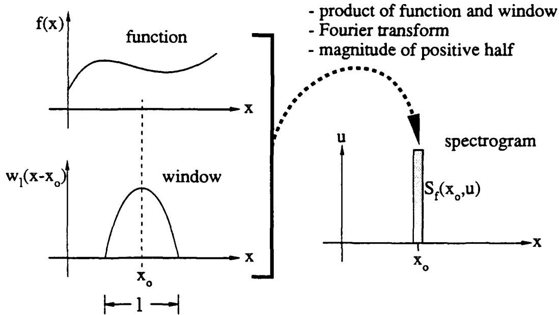
Figure 5: Computing the spectrogram
