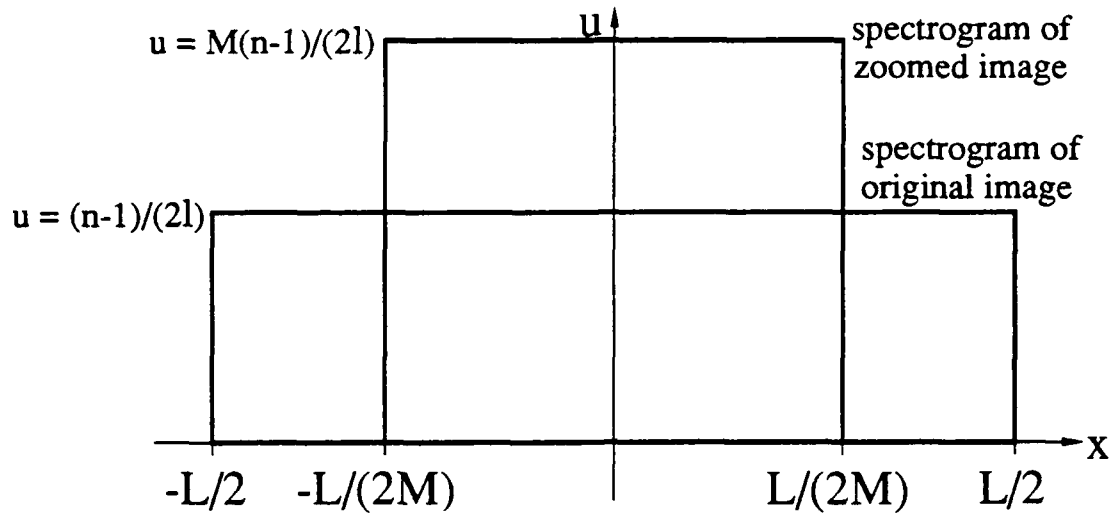
Figure 24: Effect of zooming on spectrogram dimensions
