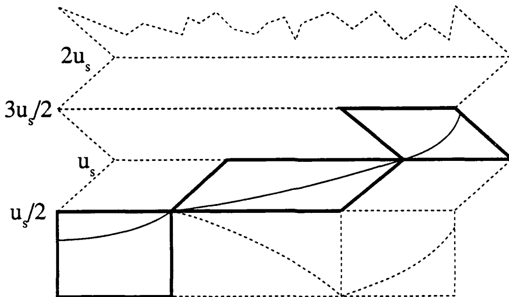
Figure 21: Folding the ideal spectrogram to show aliasing
