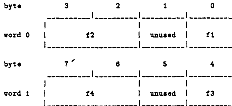
Figure 4. Pragma Pack Ignored
