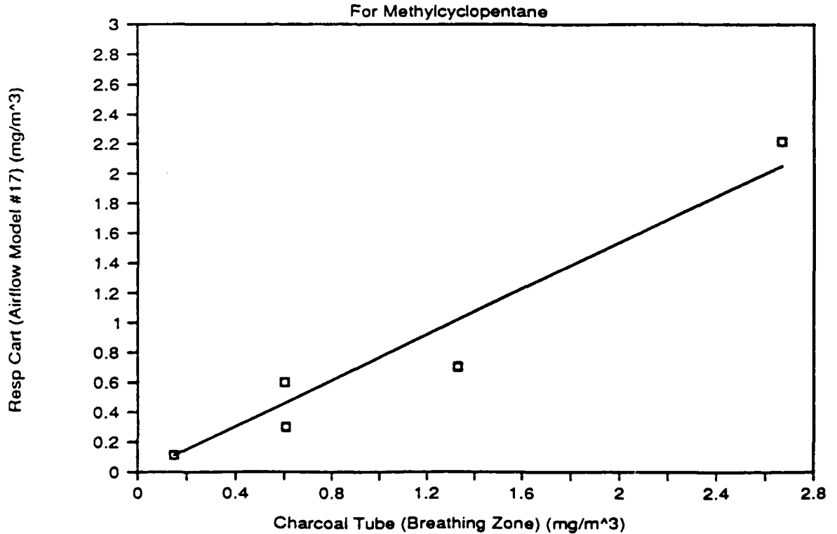
Figure 14: Organic Vapor Sample Results
