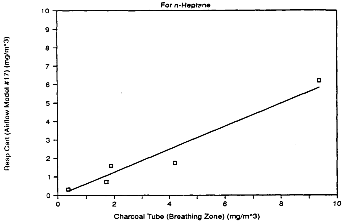
Figure 15: Organic Vapor Sample Results
