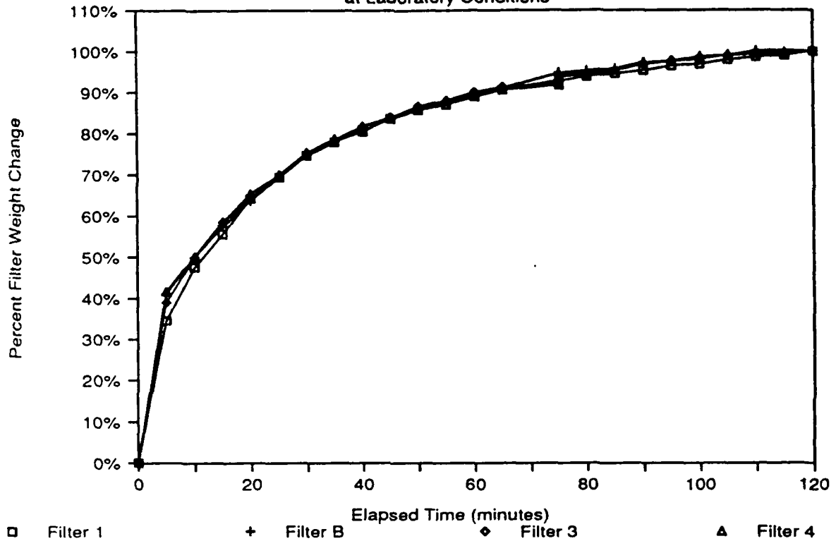
Figure 1: % Filter Wt Change vs. Time
