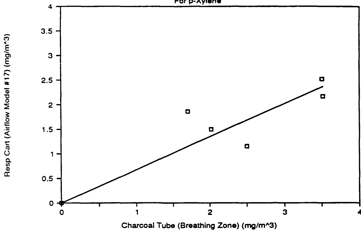
Figure 17: Organic Vapor Sample Results
