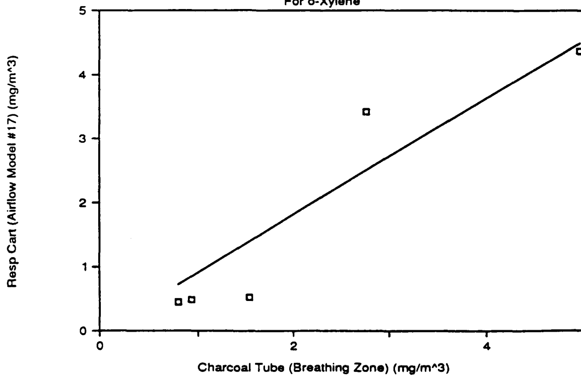
Figure 18: Organic Vapor Sample Results
