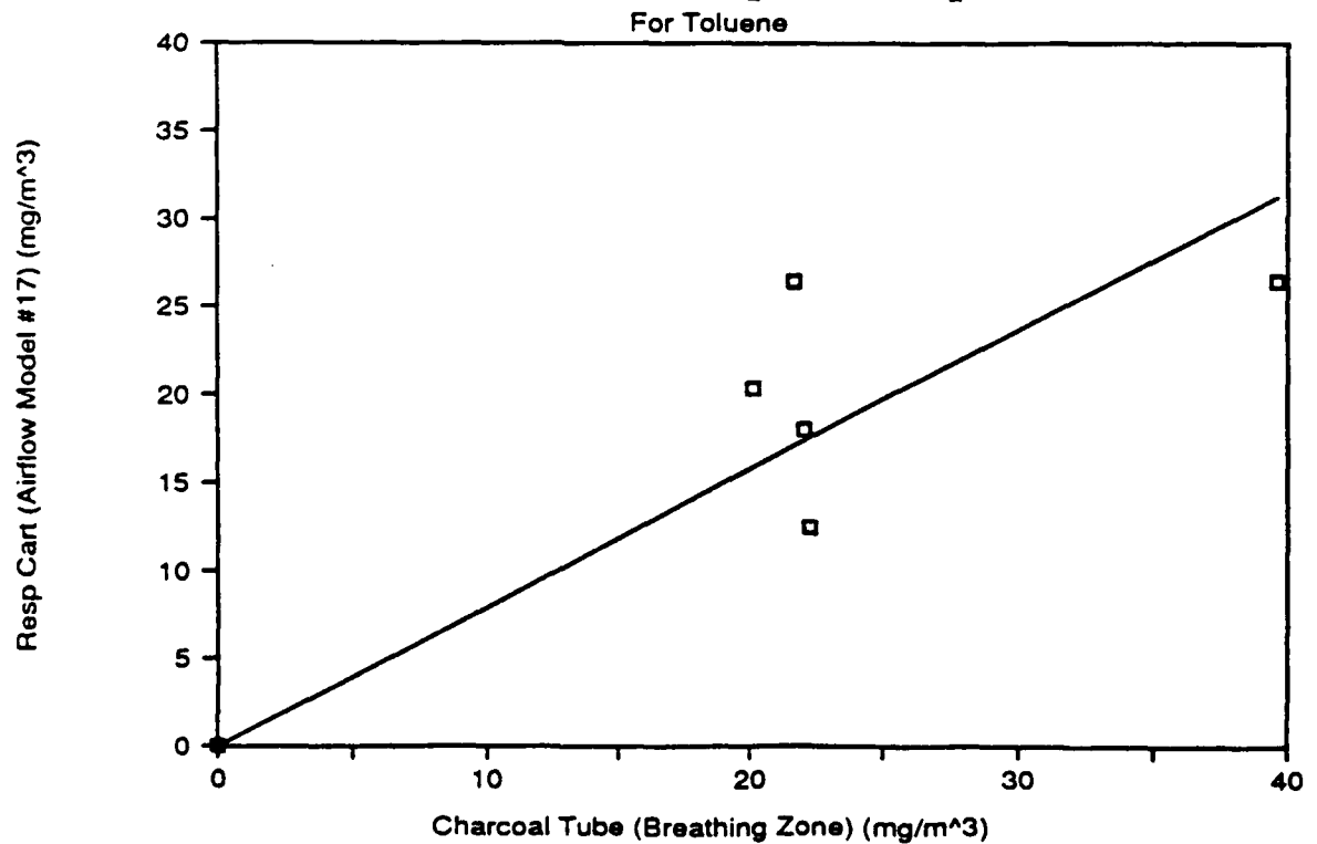
Figure 16: Organic Vapor Sample Results
