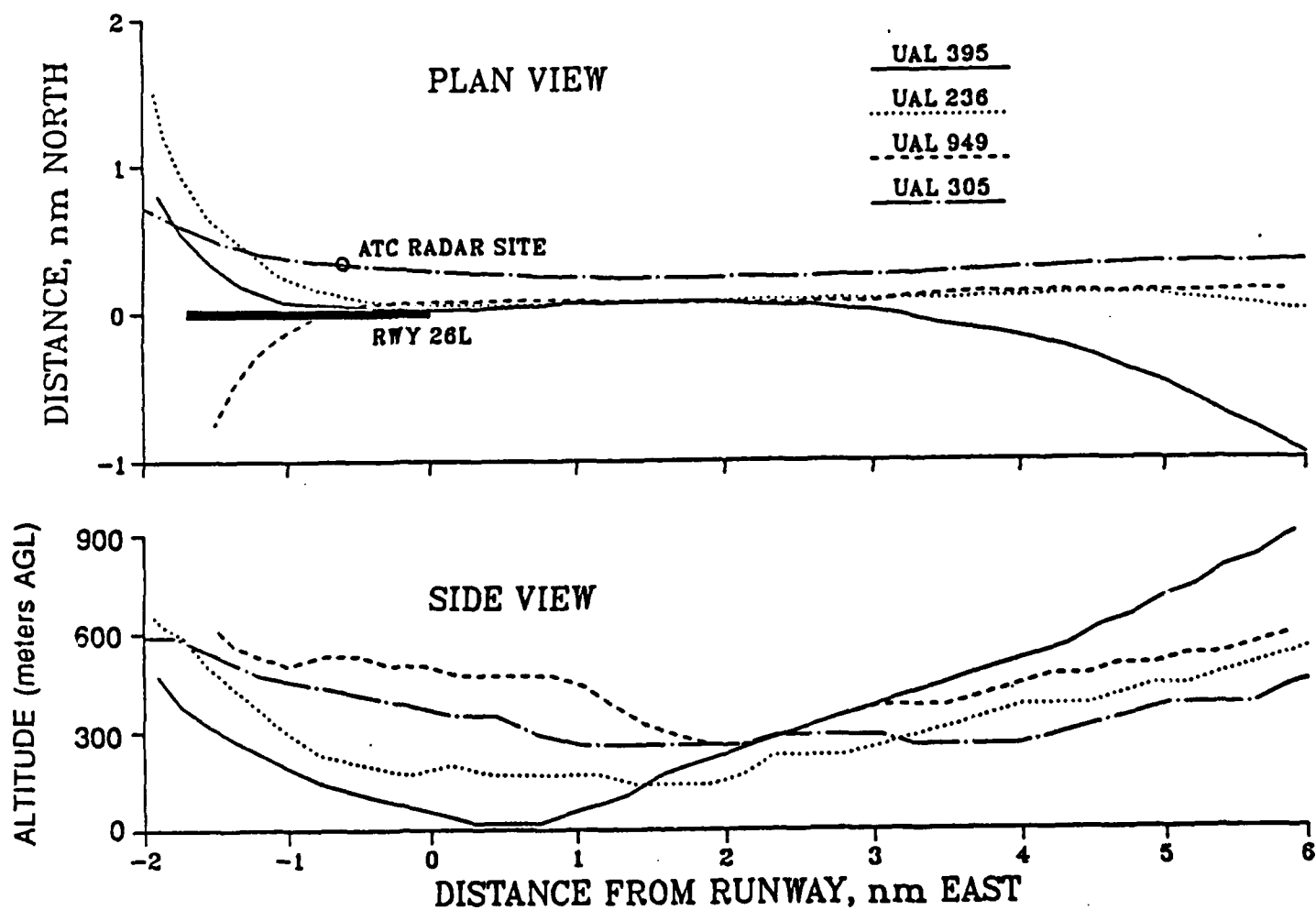
Fig. 20. Aircraft positions relative to the runway (from Wingrove and Coppenbarger 1989).
