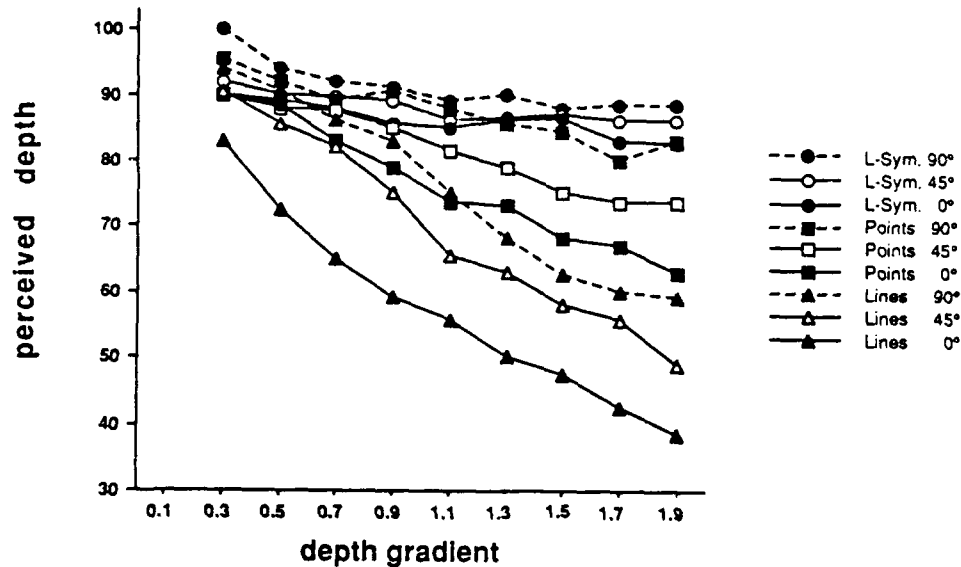
Figure 7: Perceived depth in percent of displayed depth as a function of depth gradient for points, lines and large symbols in horizontal (0 deg), oblique (45 deg) and vertical orientation (90 deg). Each data item represents the mean of nine different disparities (3-27 arc min) tested with 10 subjects. The standard errors of the means are in the order of the symbol size.
