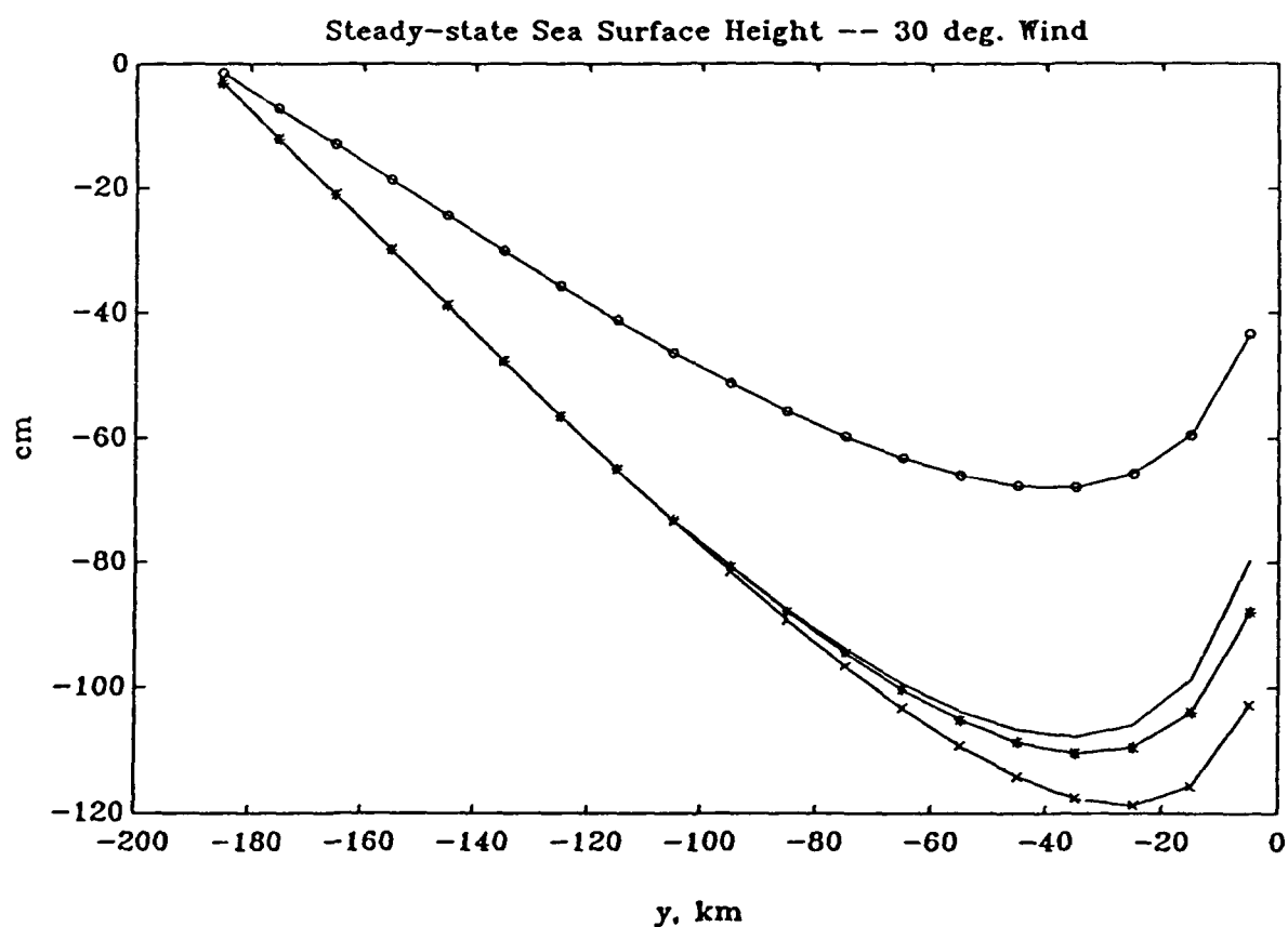
Figure 3-37: Steady-state surface profile for a wind angle of 30°. Curves are for the 2½-D model (—), traditional model with r = r_{\min} (x—x), traditional model with r = r_{\max} (o—o) and traditional model with r = r(y) (*—*).
