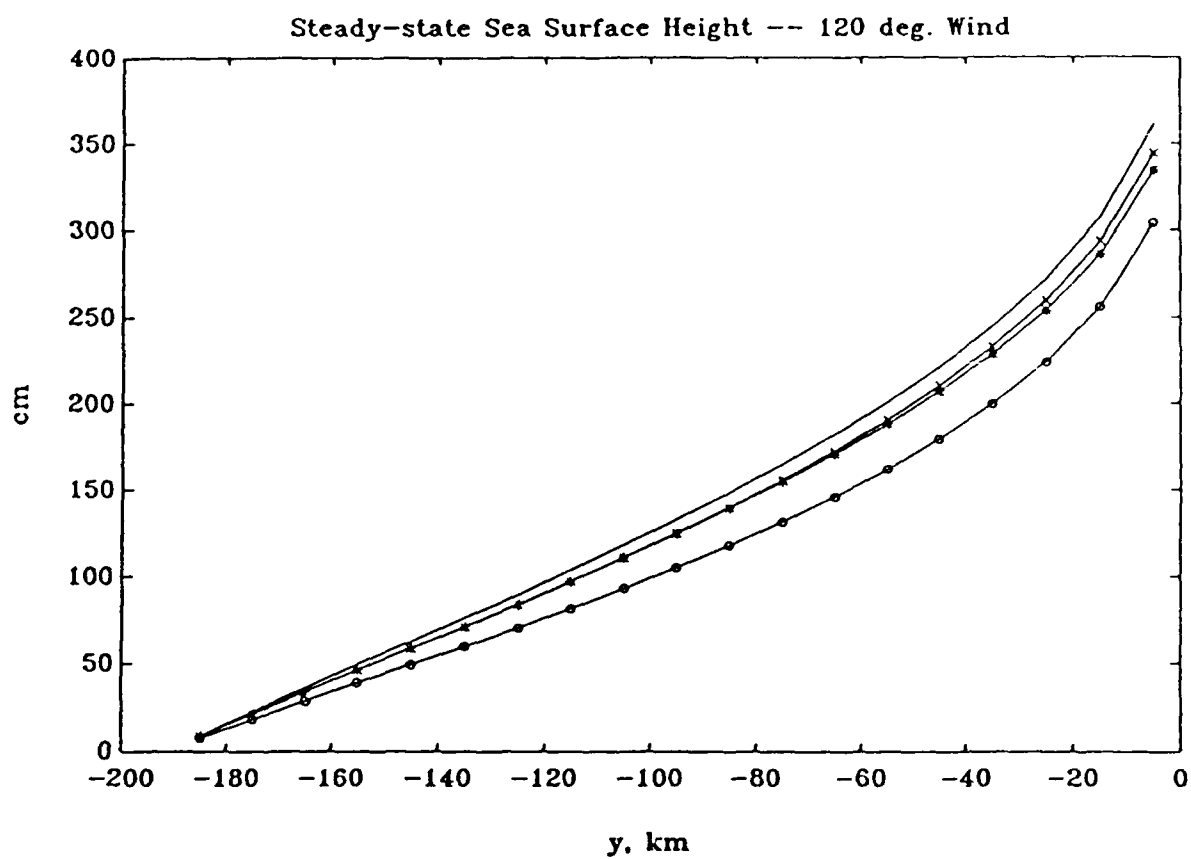
Figure 3-39: Steady-state surface profile for a wind angle of 120^\circ . Curves are for the 2\frac{1}{2} -D model (—), traditional model with r = r_{\min} (x—x), traditional model with r = r_{\max} (o—o) and traditional model with r = r(y) (+—+).
