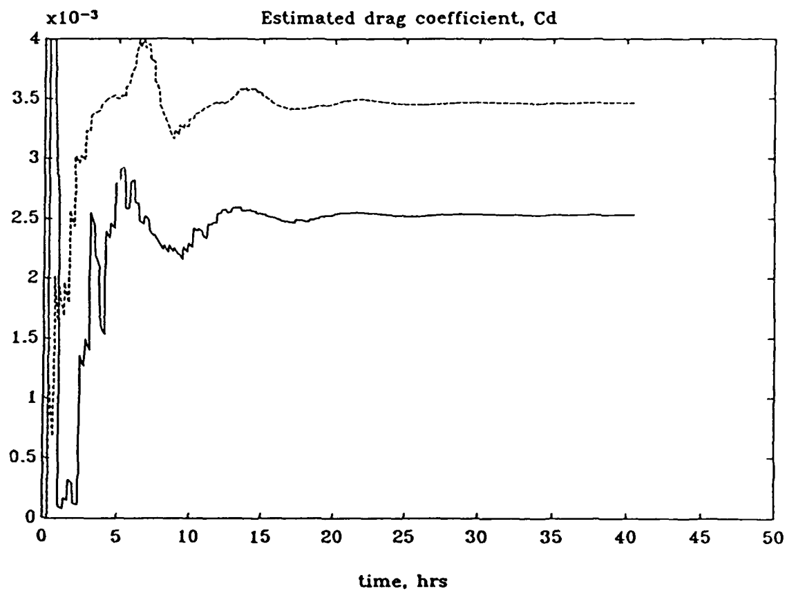
Figure 3-33: Time series of estimated drag coefficient at the offshore (solid line) and onshore (dashed line) points. The spike in the offshore point signal is truncated at .004 although its actual maximum is C_d \approx .023 .
