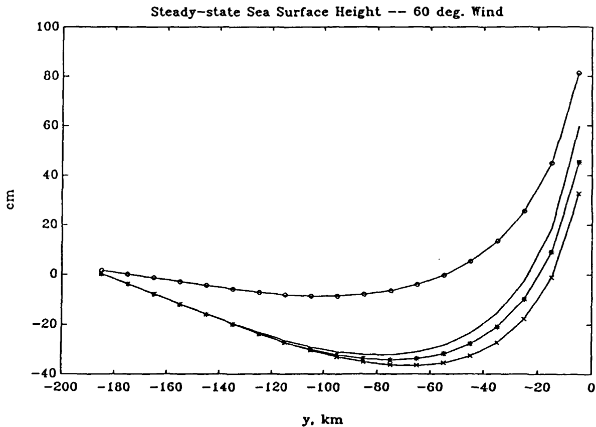
Figure 3-38: Steady-state surface profile for a wind angle of 60^\circ . Curves are for the 2\frac{1}{2} -D model (—), traditional model with r = r_{\min} (x—x), traditional model with r = r_{\max} (o—o) and traditional model with r = r(y) (*—*).
