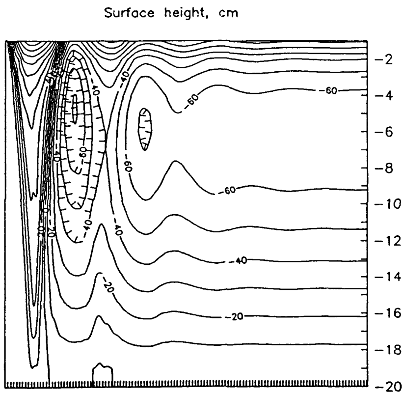
Figure 3-26: Contour plot of sea surface height on the y - t plane. Tic marks are at intervals of 5\Delta t and \Delta x on the horizontal and vertical axes, respectively. The time axis ranges from 0 to 40 hrs.
