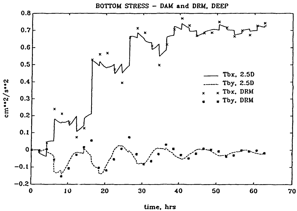
Figure 3-16: Time series of deep case kinematic bottom stress components \tau_{bx}/\rho, \tau_{by}/\rho from the DAM (continuous curves) and from the DRM (symbols).
