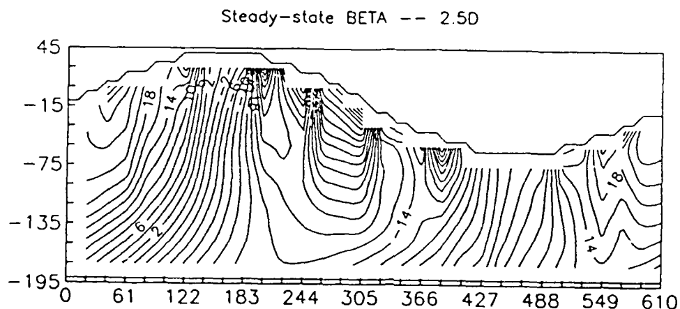
Figure 3-50: Contour plot of \beta at steady-state. Contour interval is 2^\circ .
