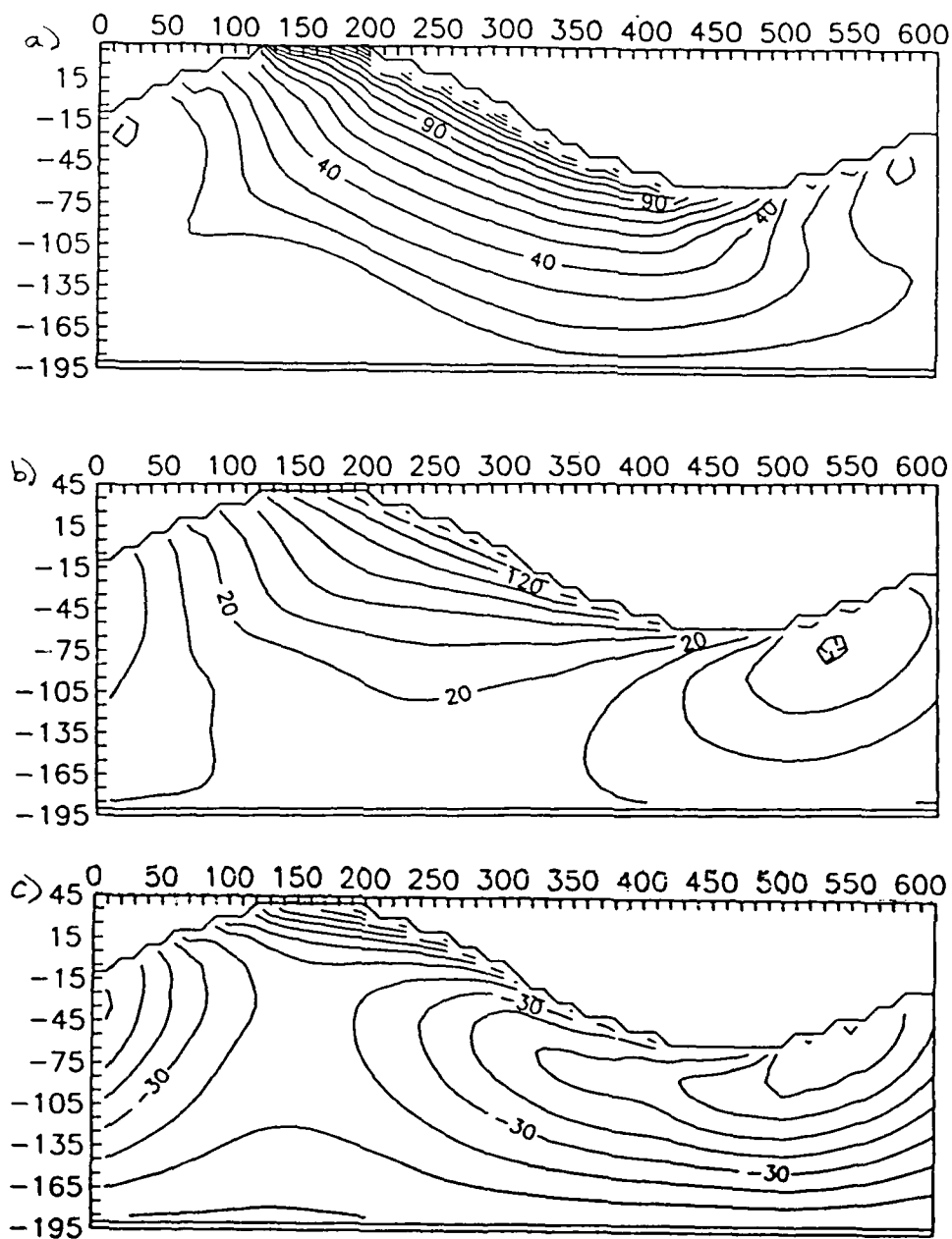
Figure 3-42: Contours of surface elevation at a) 2.4, b) 4.8 and c) 7.2 hrs.
