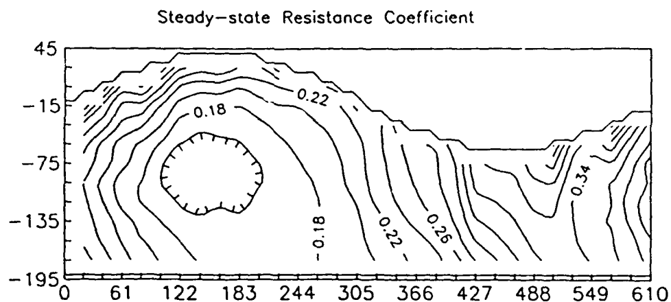
Figure 3-52: Steady-state resistance coefficient.
