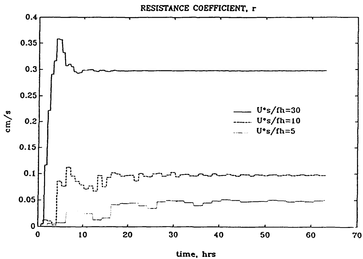
Figure 3-17: Time series of resistance coefficient at the offshore point.
