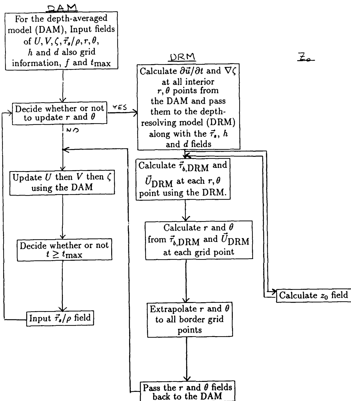
Figure 2-8: Schematic of the full 2\frac{1}{2} -D model.
