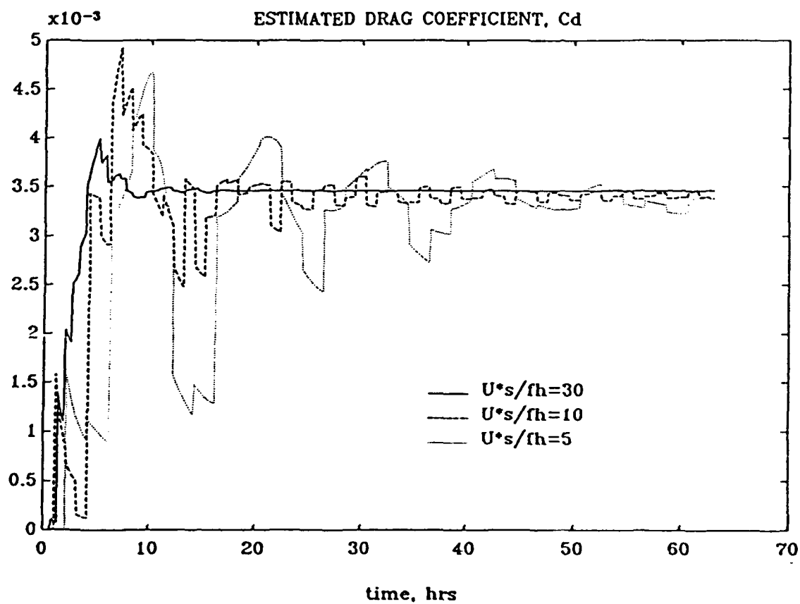
Figure 3-18: Time series of estimated drag coefficient at the offshore point.
