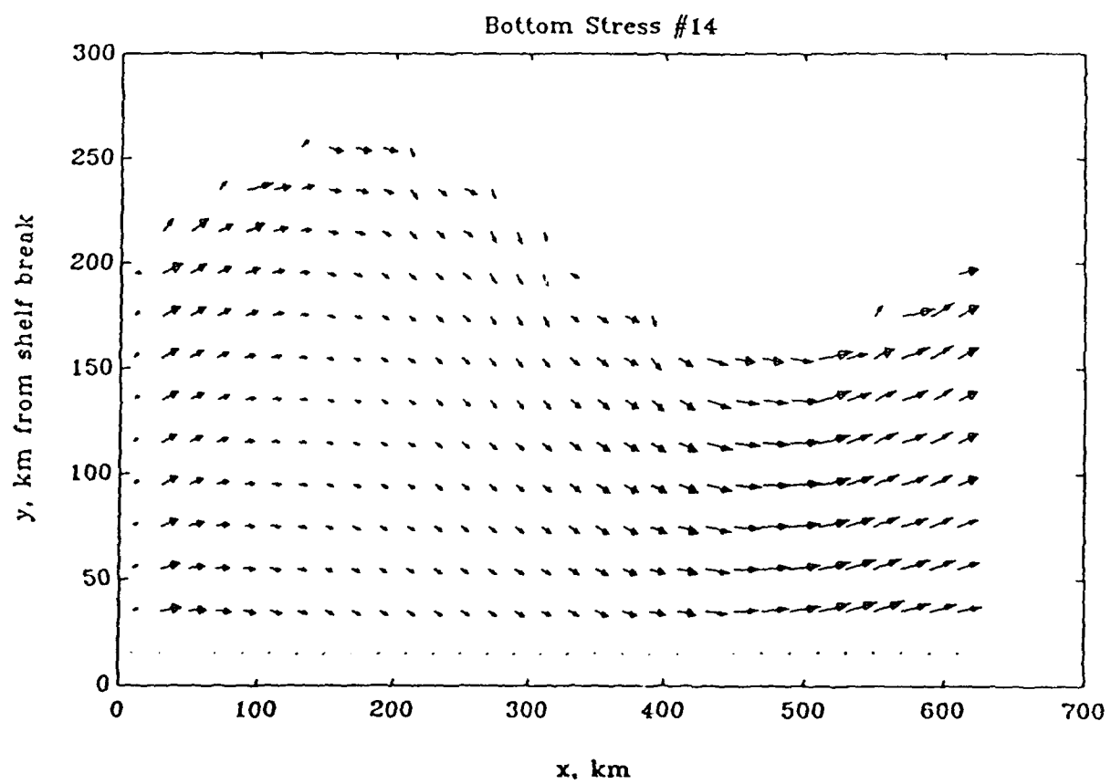
Figure 3-51: Steady-state kinematic bottom stress field. Scale: 1 cm = 60 \text{ cm}^2/\text{s}^2 .
