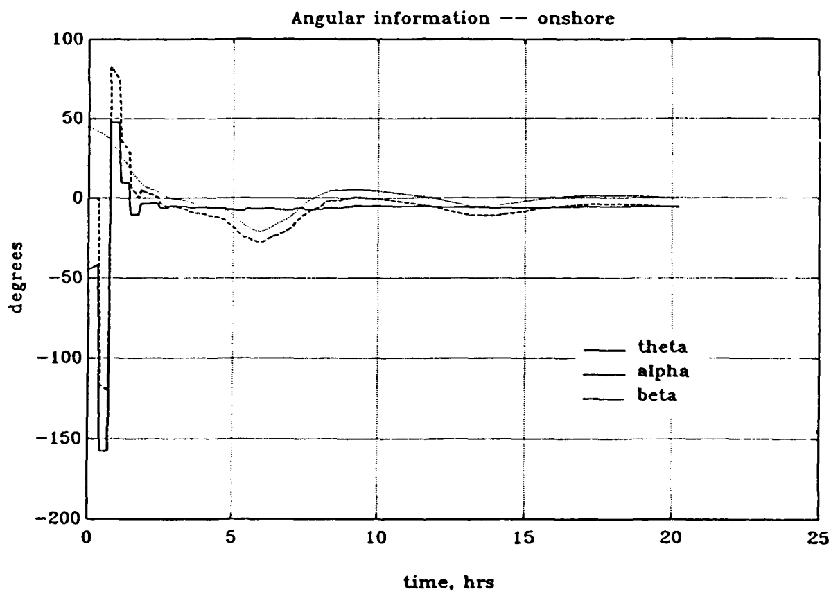
Figure 3-34: Time series of angular information at the onshore point.
