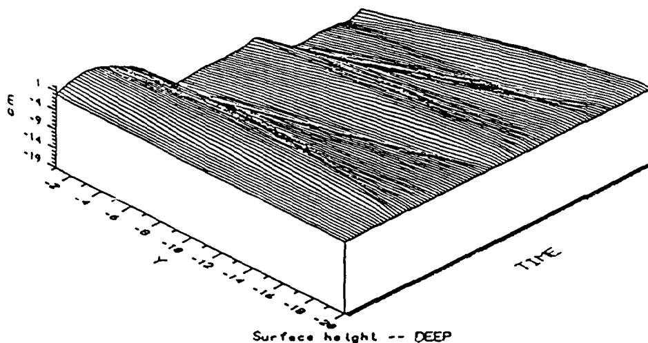
Figure 3-8: 3-D plot of sea surface height in y-t space for the deep case. Tic mark spacing is \Delta t on the time axis and \Delta x on the y axis.
