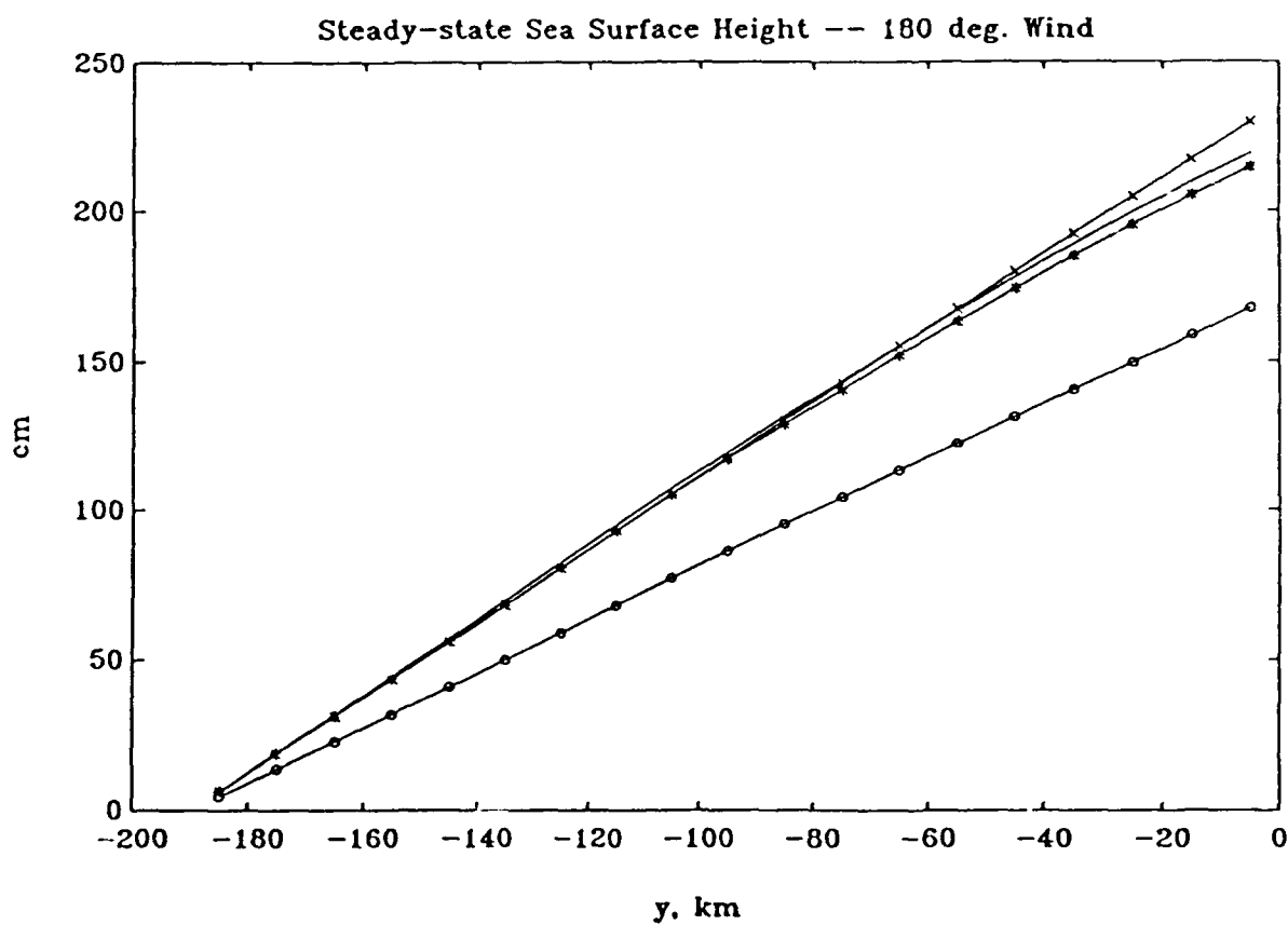
Figure 3-41: Steady-state surface profile for a wind angle of 180^\circ . Curves are for the 2\frac{1}{2} -D model (—), traditional model with r = r_{\min} (x—x), traditional model with r = r_{\max} (o—o) and traditional model with r = r(y) (*—*).
