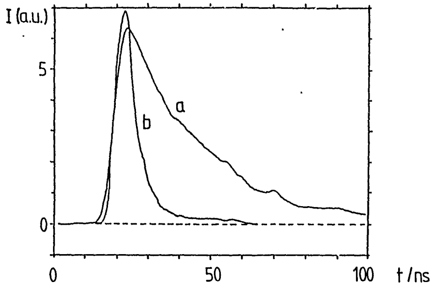
Fig. 1 Time - resolved H atom fluorescence signals; curve a from discharge-flow reactor at 2 mbar, curve b from H_2/O_2 - flame at 95 mbar
