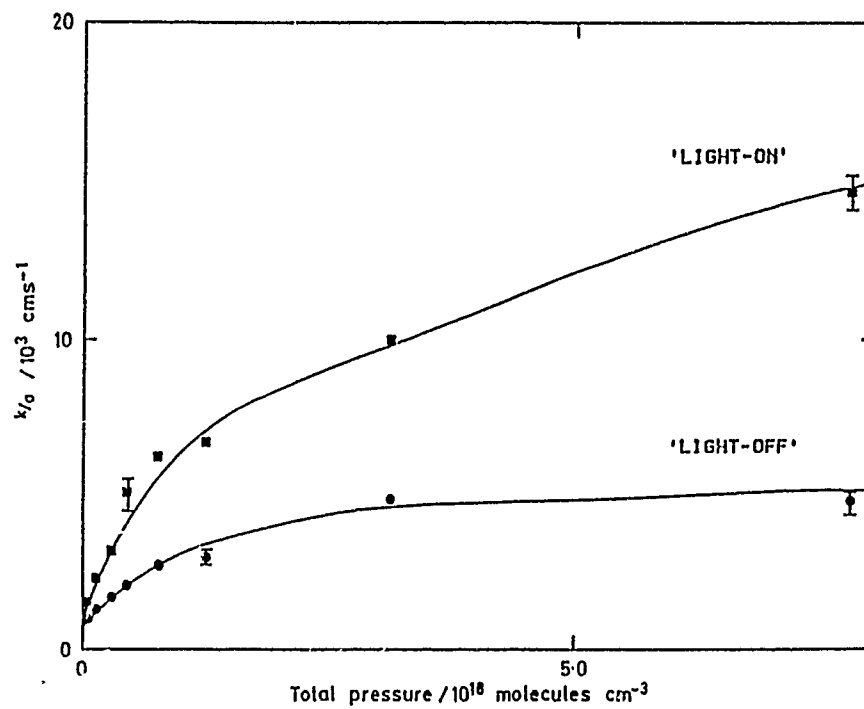
FIGURE 1 - PRESSURE DEPENDENCE OF THE OBSERVED BINOMOLECULAR RATE CONSTANTS AT 308K
