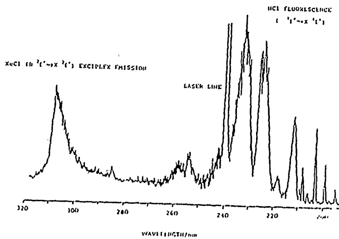
Figure 1(c) Dispersed fluorescence showing XeCl(B 2 2,1 - X 2 2,1 ) exciplex chemiluminescence.
