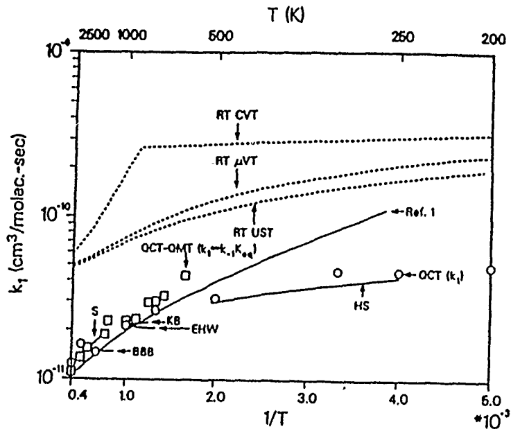
Figure 2. Arrhenius plot of k_1,0 + OH \xrightarrow{k_1,1} O_2 + H . Variational transition state theory results are from Raj and Truhlar (RT). Trajectory results are from J. A. Miller, J. Chem. Phys. 74, 5120 (1981), (marked Ref. 1 on the figure) and from this work. Experimental results are from Smith and Howard (HS), Schott (S), Brabbs, Belles and Brokaw (BBB), Eberius, Hoyermann and Wagner (EHW), and Kurzius and Boudart (KB).
