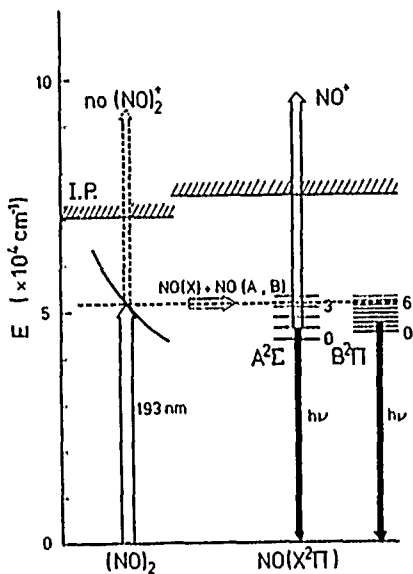
Fig. 1 A schematic representation of the mechanism of the photolysis of the NO dimer
