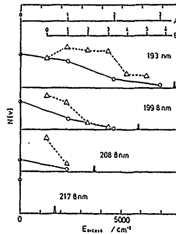
Fig. 4 The electronic and vibrational energy partitioning. O: A state, Δ: B state.
