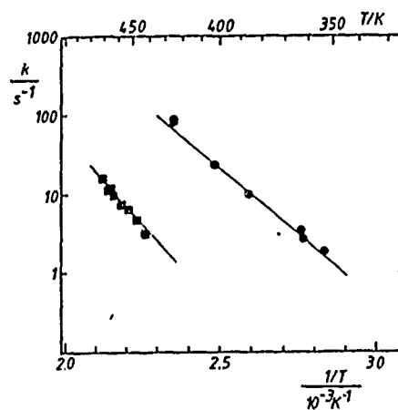
Figure 2: Arrhenius plots of the rate constants for the unimolecular decay of the adducts imidazole-OH (●) and thiophene-OH (■) back to the reactants.
