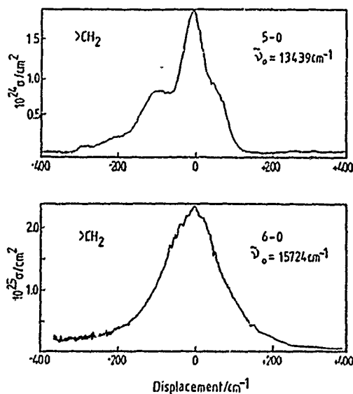
Fig. 2. Laser photoacoustic spectra of gas phase cyclobutene in the region of the \nu=5 and 6 methylenic C-H stretch overtones.
