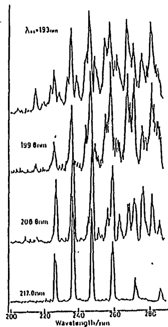
Fig. 2 The emission spectra observed by the photolysis of (NO)_2 at several wavelengths.
