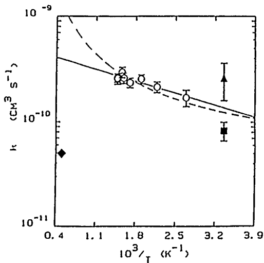
Fig. 2 Arrhenius plot for \text{CH}_2 + \text{H} \rightarrow \text{CH} + \text{H}_2 : \circ this work, \blacksquare Grebe and Homann (Ref. 2), \blacktriangle Bohland and Temps (Ref. 3), \blacklozenge Lohr and Roth (Ref. 4). Solid line is Arrhenius fit, broken line is transition-state theory calculation fit.
