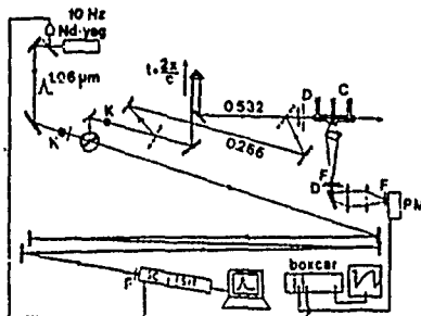
fig. 1 - Experimental Setup
