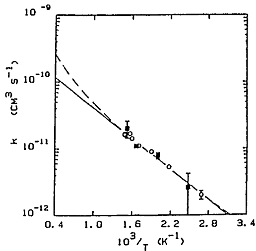
Fig. 1 Arrhenius plot for \text{CH} + \text{H}_2 \rightarrow \text{CH}_2 + \text{H} : \circ this work, \blacksquare Berman and Lin (Ref. 1). Solid line is Arrhenius fit, broken line is transition-state theory calculation fit.
