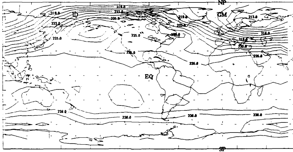
Figure 2.16a: MSU Channel 3 Brightness Temperature (K) (8-31 Jan 87)
