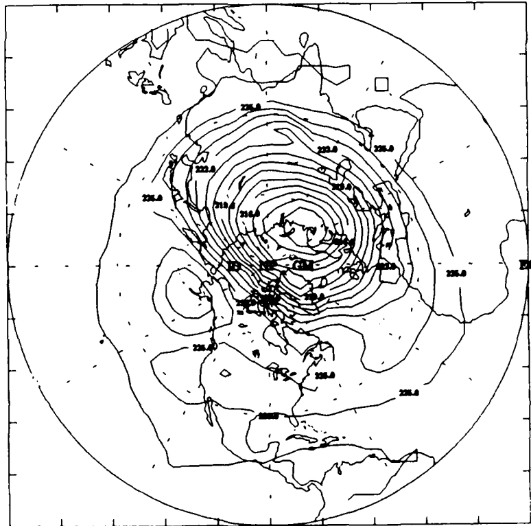
Figure 2.16b: MSU Channel 3 Brightness Temperature (K) Northern Hemisphere (8-31 Jan 87)
