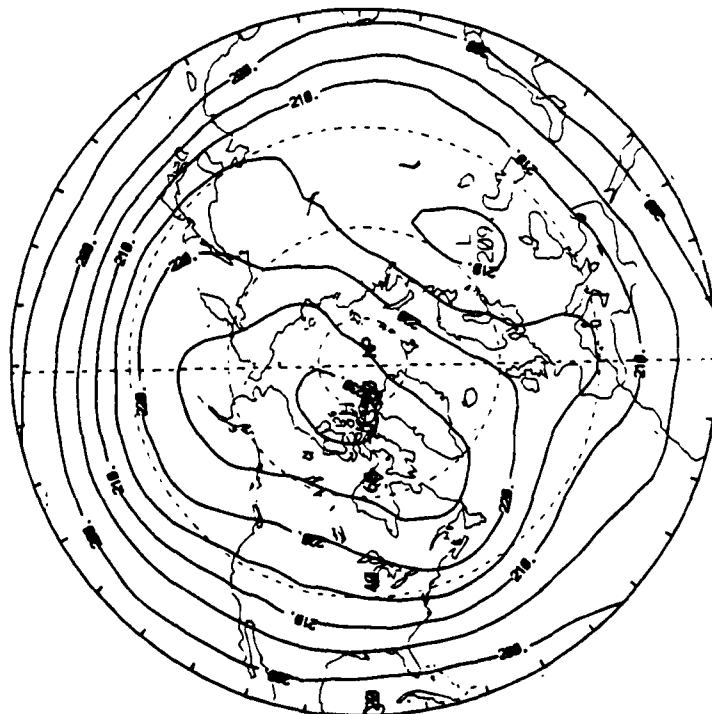
Figure 4.4: Comparison between MSU Channel 4 and ECMWF 100 mb. A) MSU Channel 4, 1-18 Feb 87, Contour Interval 2 K. B) ECMWF 100 mb Temperature Field, 1-18 Feb 87, Contour Interval 5K.
