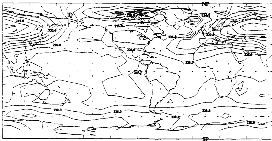
Figure 2.17a: MSU Channel 3 Brightness Temperature (K) (1-18 Feb 87)
