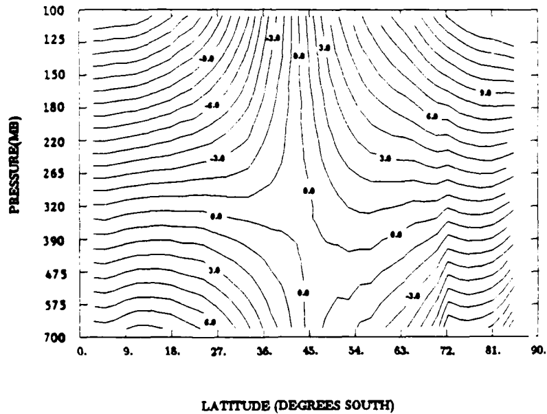
Figure 4.9: MSU Temperature Anomaly Fields for 8-31 Jan 87 along A) 165° East (NH), B) 165° East (SH), C) 110° West (NH), D) 110° West (SH), E) 75° West (NH), F) 75° West (SH). Anomaly fields are determined using CH2=700 mb, CH3=300 mb, and CH4=100mb and run from 2.5 - 87.5° latitude.
