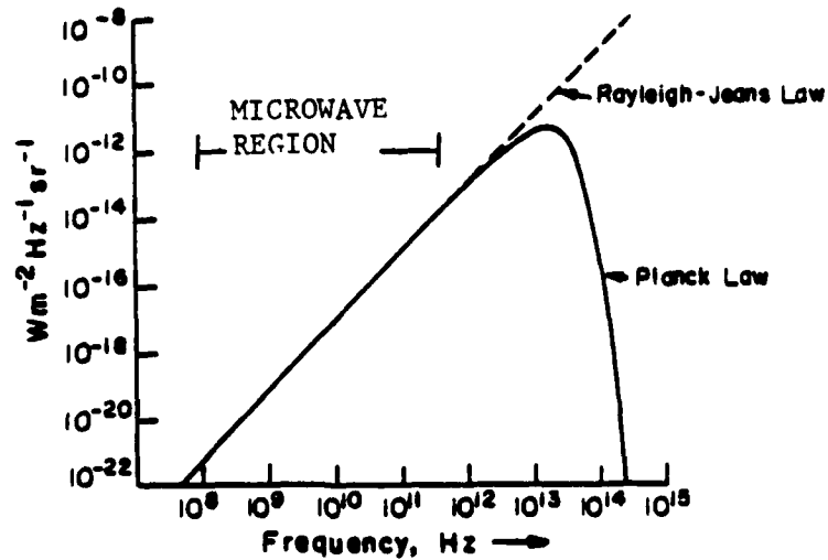
Figure 2.1: Comparison of Planck's law with Rayleigh-Jean's Law at T = 300 K (From Tsang et al., 1985).
