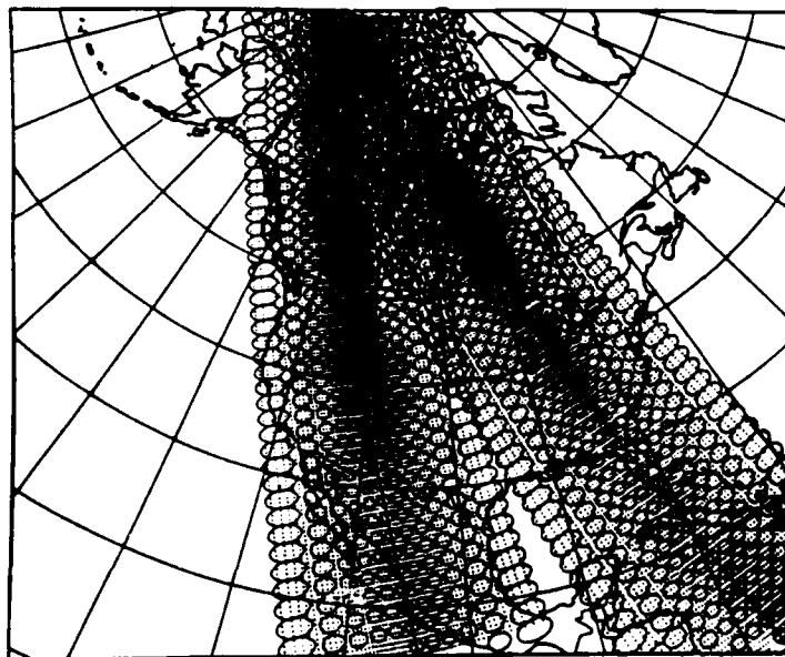
Figure 2.10: MSU Scan Pattern Two Consecutive Orbits. (Smith et. al., 1979) shown along with HIRS scan pattern (small dots).
