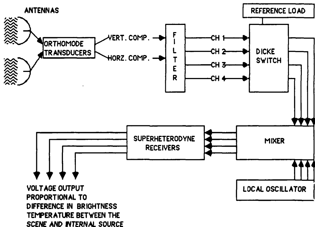
Figure 2.11: The MSU Radiometer Subsystem (Adapted from Njoku, 1982).
