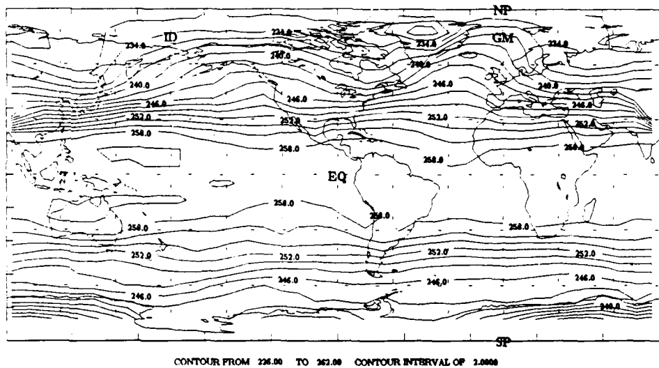
Figure 2.14a: MSU Channel 2 Brightness Temperature (K) (8-31 Jan 87)
