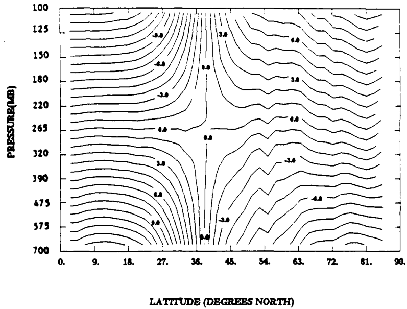
Figure 4.7a: Brightness Temperature Anomaly Field derived from MSU data for Northern Hemisphere along 165°E longitude (contour interval = 1°K)
