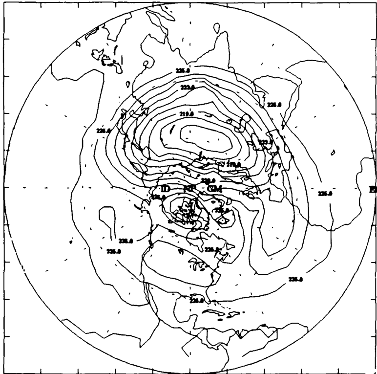
Figure 2.17b: MSU Channel 3 Brightness Temperature (K) Northern Hemisphere (1-18 Feb 87)
