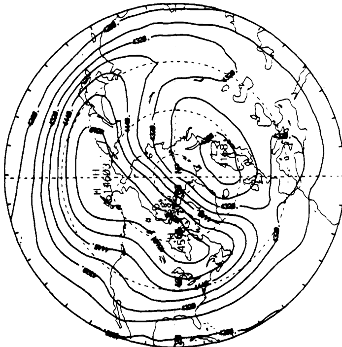
Figure 4.17: Comparison between MSU Channel 4 and ECMWF Thickness. A) MSU Channel 4, 8-31 Jan 87, Contour Interval 2 K. B) ECMWF 200-100 Geopotential Thickness Field, 8-31 Jan 87, NH, Contour Interval 60m.
