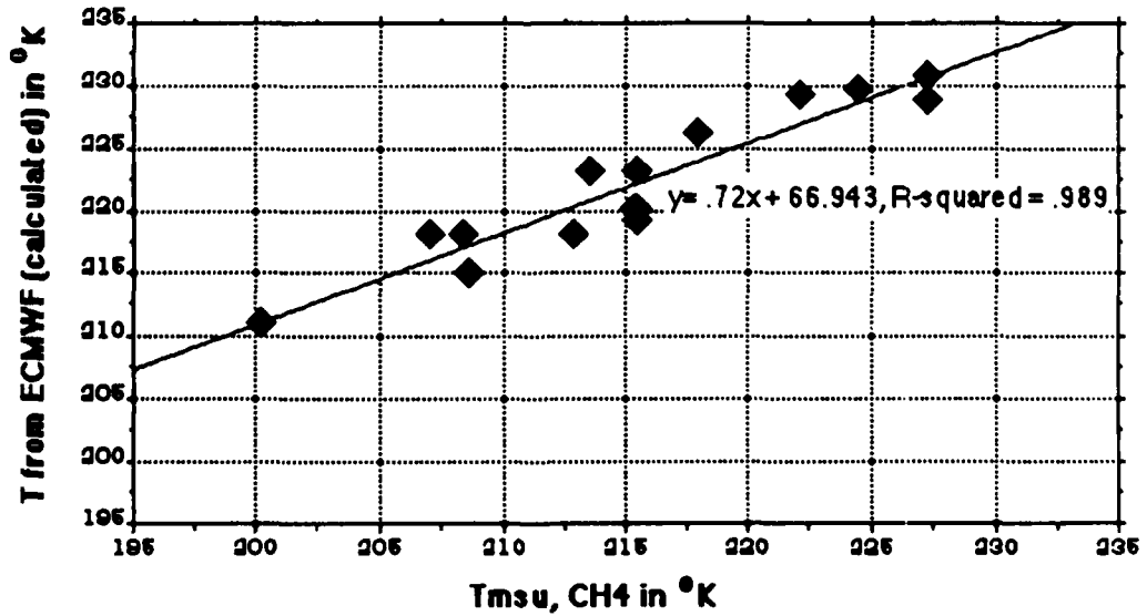
Figure 4.20: Comparison between MSU and calculated Temperature
