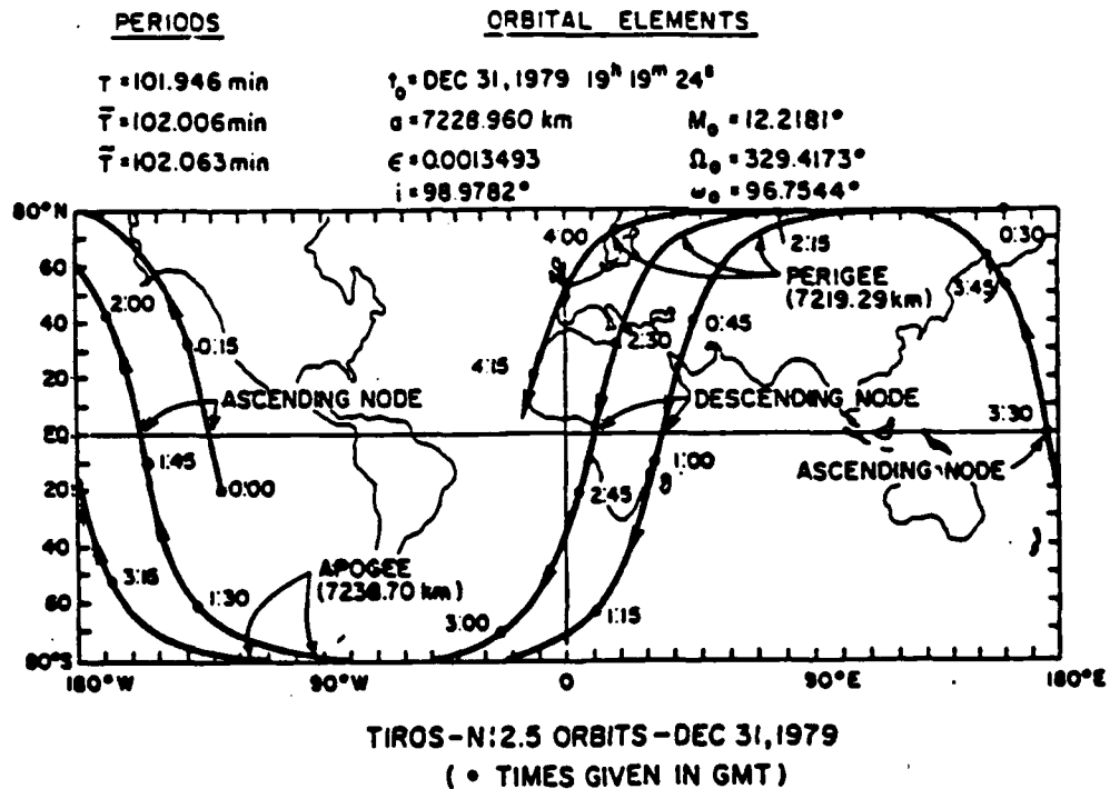
Figure 2.6: The Ground Track of a Sun-synchronous Satellite
