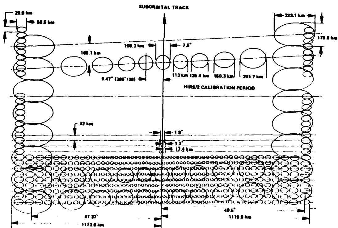
Figure 2.8: MSU Scan Line pattern (large oblate circles) projected on Earth, coverage pattern is shown in relation to the High Resolution Infrared Radiation Sounder (HIRS/2) instrument (smaller circles). (Schwalb, 1978)
