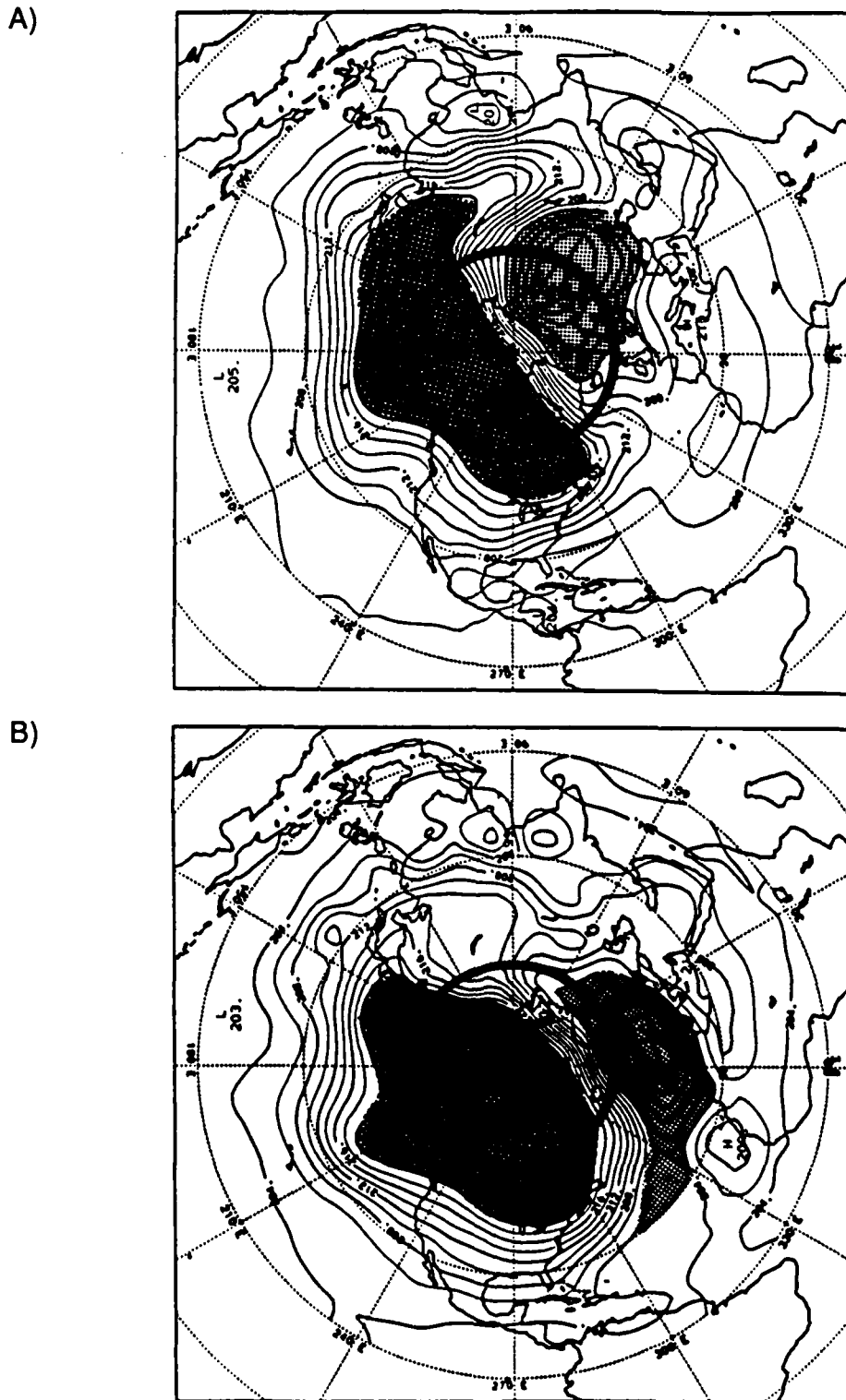
Figure 4.30: NMC 50 mb Temperature (K) Field for A) 12Z Jan 20 1987, and B) 12Z Jan 25 1987 with regions colder than 204 K shaded and regions warmer than 220 K hatched; and NMC 50 mb Geopotential Height (GPM) Field for C) 12Z Jan 20 1987, and D) 12Z Jan 25 1987.
