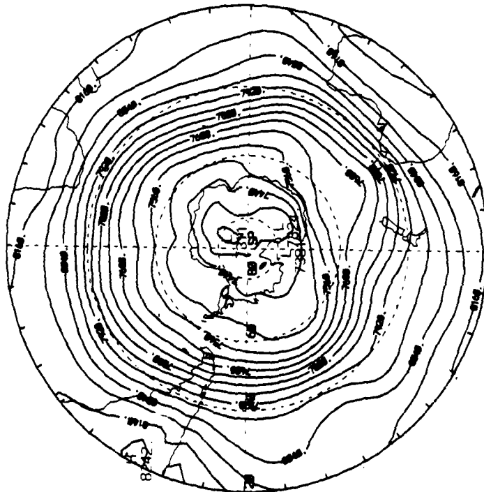
Figure 4.14: Comparison between MSU Channel 2 and ECMWF Thickness.
