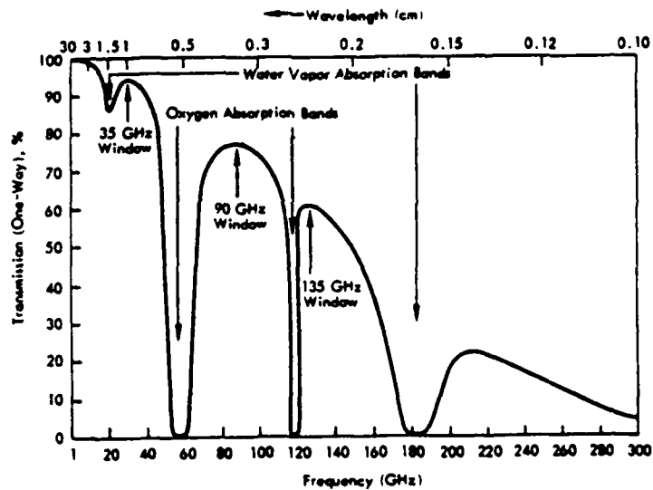
Figure 2.3: Percent Transmission through the Earth's Atmosphere, along the vertical, under clear sky conditions (Ulaby, 1981)
