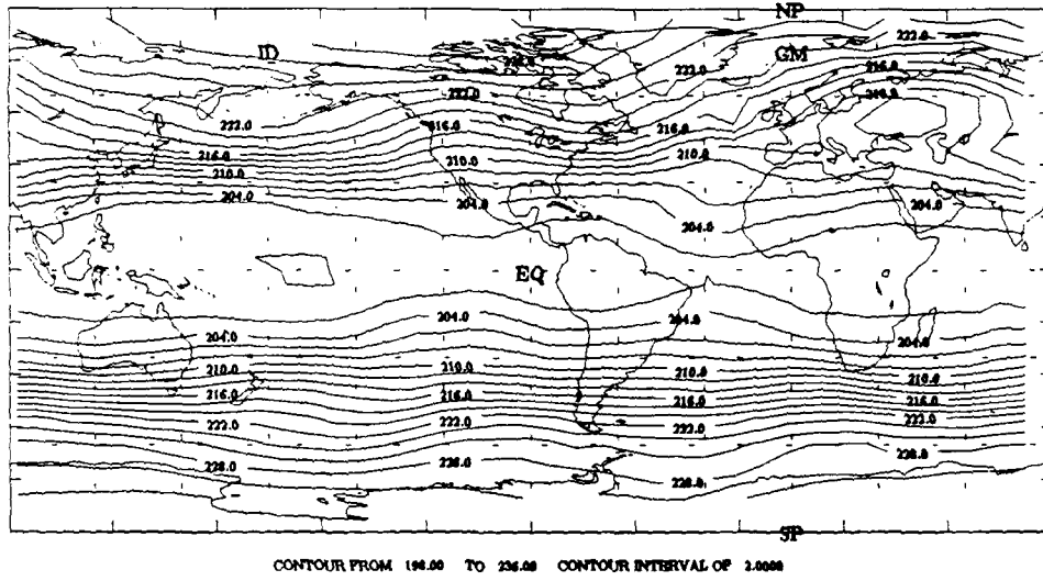
Figure 2.19a: MSU Channel 4 Brightness Temperature (K) (1-18 Feb 87)
