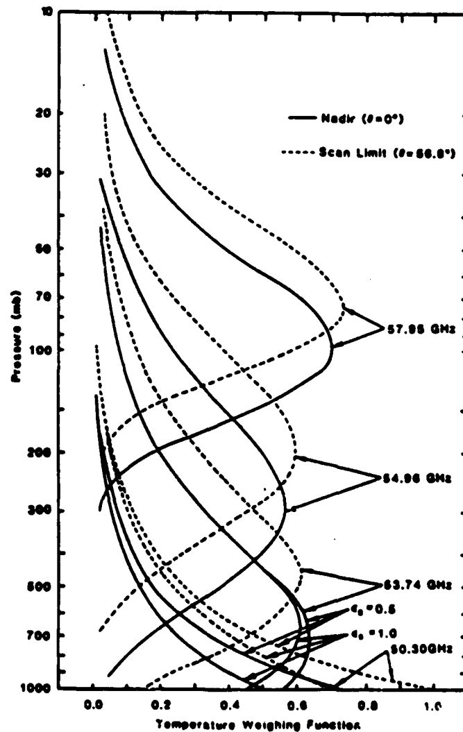
Figure 2.4: MSU Weighting Function at nadir and scan limit positions (From Grody, 1983).
