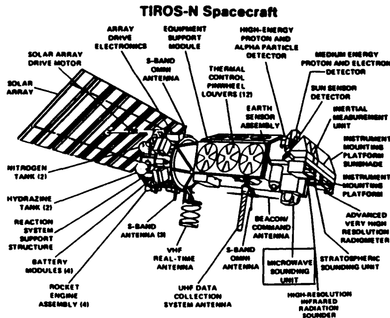
Figure 2.5: The TIROS-N Series Spacecraft (After Schwalb, 1978)
