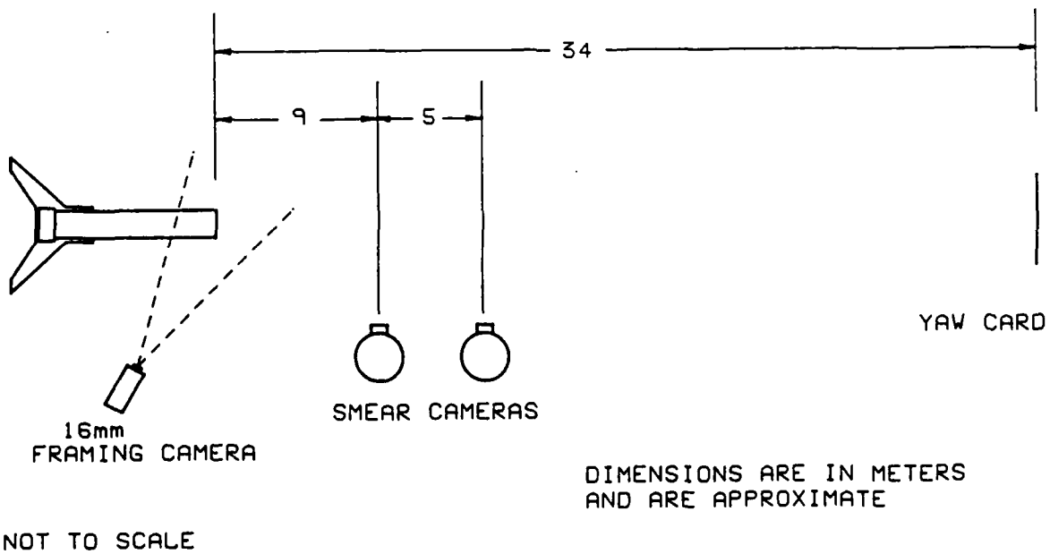
Figure 5. Test set-up.
