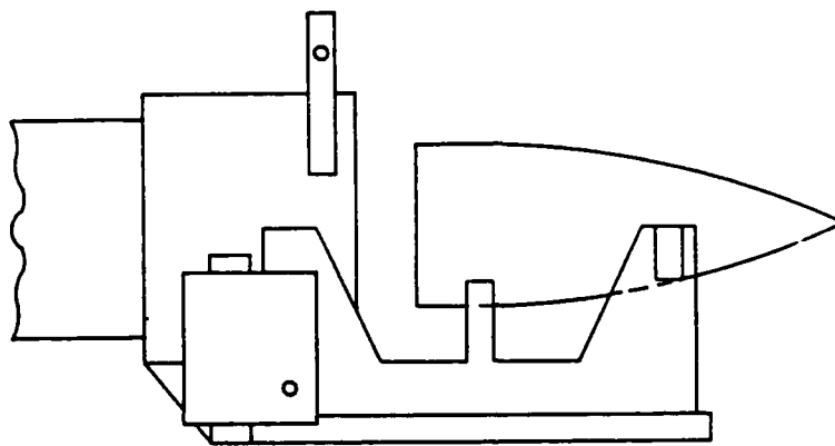
CORRECTLY FUNCTIONING YAW INDUCER PART 2 REMAINS ATTACHED TO PART 1 DURING RECOIL
