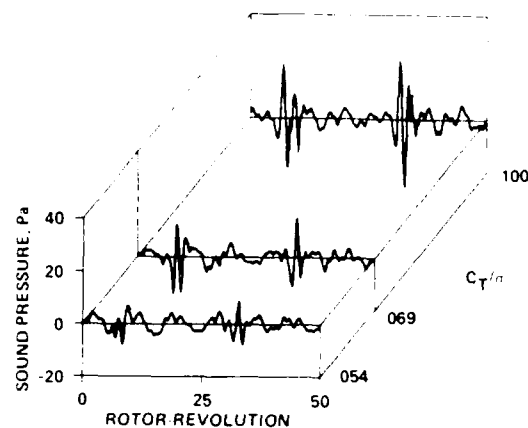
Figure 15. BVI waveform comparisons for microphone 3 at \mu=0.198 .
