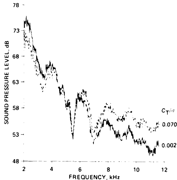
Figure 25. Power spectrum for overhead microphone, number 20, at two thrust values.
