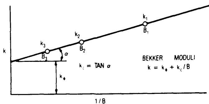
Figure 2.2-3. Sinkage moduli diagram (after Hvorslev, 1970).
