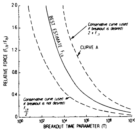
Figure 2.3-5. Normalized long-term breakout force as a function of breakout time parameter (after Rocker, 1985) [ F_{LB} = long-term breakout force carried by the sediment ( F ); F_{lb} = immediate breakout force carried by the sediment ( F )].
