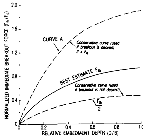
Figure 2.3-3. Normalized immediate breakout force as a function of relative embedment depth (after Rocker, 1985) [ F_{lb} = immediate breakout force carried by the sediment ( F ); F_q = bearing capacity of the sediment under a vertical downward load ( F )].
