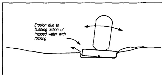
Figure 1.1-5. Sinkage/embedment of footing while rocking subject to oscillatory lateral force.
