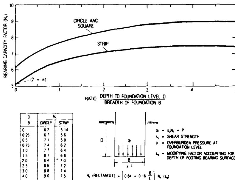
Figure 2.2-6. Bearing-capacity factors for foundations in clay ( \phi = 0 ) (after Skempton, 1951).
