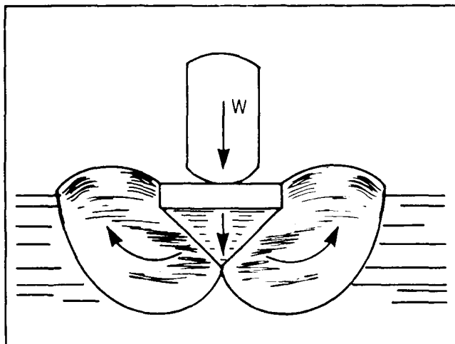
Figure 1.1-1. Bearing capacity or sinkage failure of footing on cohesive sediment, vertical noneccentric loading. W = submerged weight of structure.
