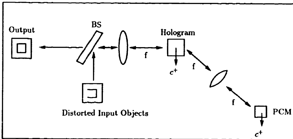
Figure 1. Single Iteration Holographic Associative Memory
