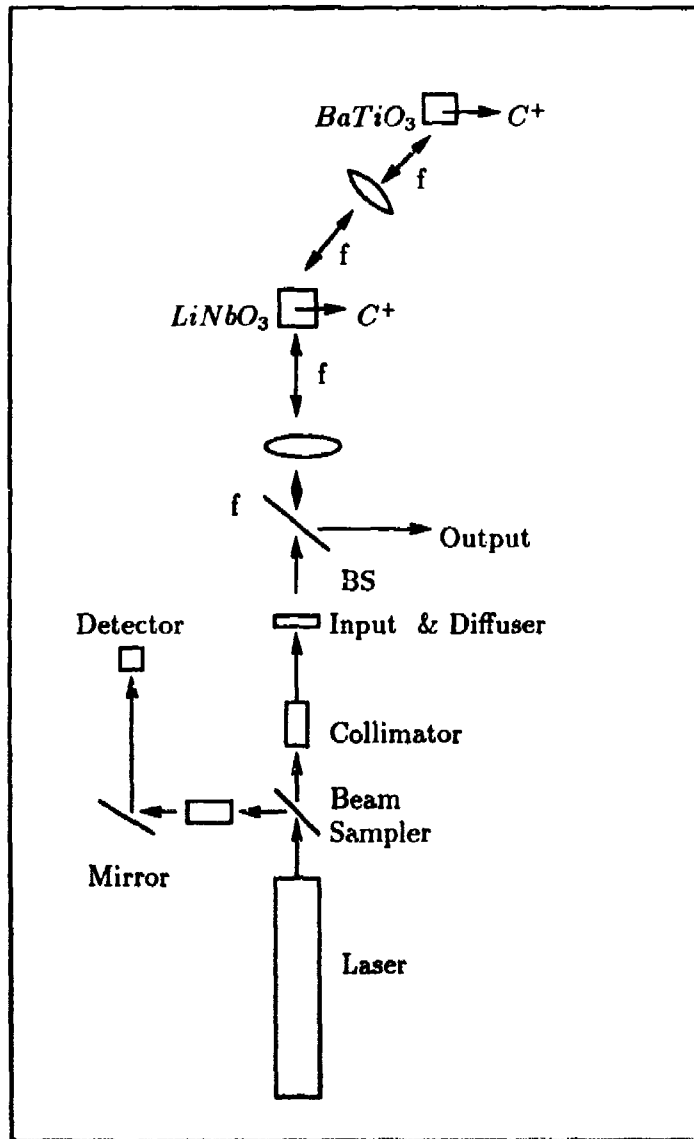
Figure 2. The Holographic Associative Memory
