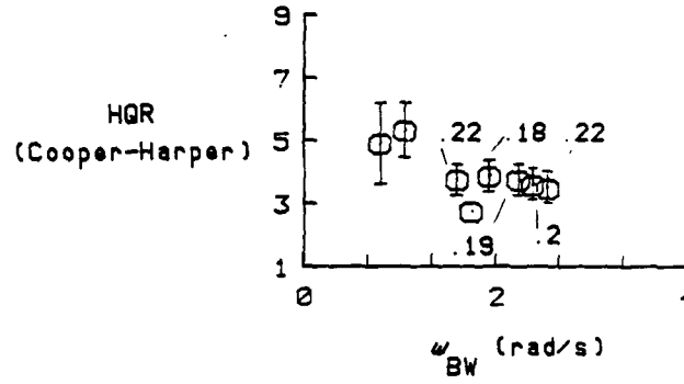
Fig 17 Variation in pilot rating with phase-limited bandwidth
