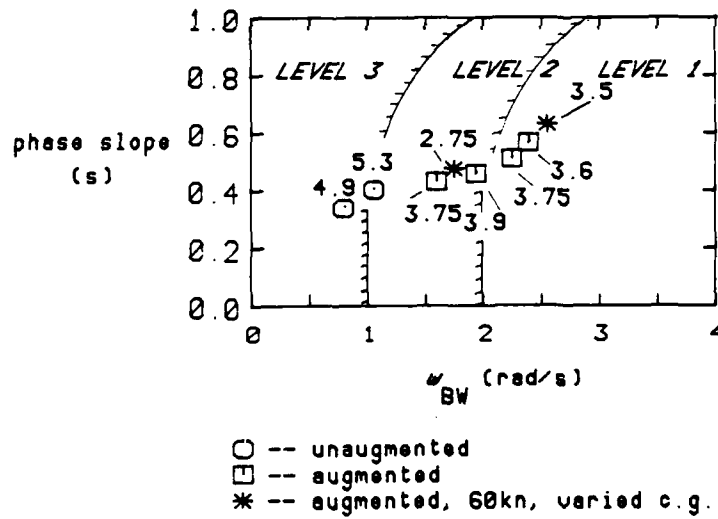
Fig 24 Correlation of Puma characterisation in terms of phase slope and bandwidth
