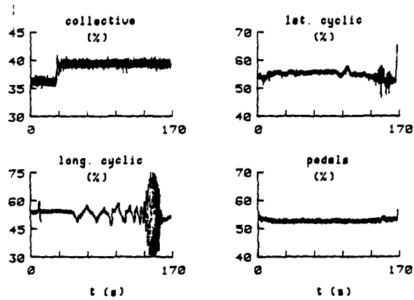
Fig 6 Control input time histories, augmentation engaged, 20 kn
