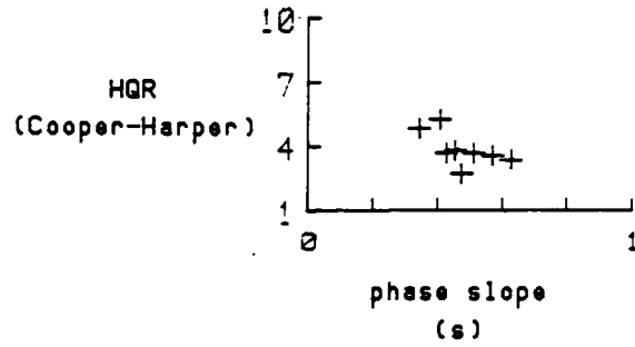
Fig 25 Variation in pilot rating with phase slope
