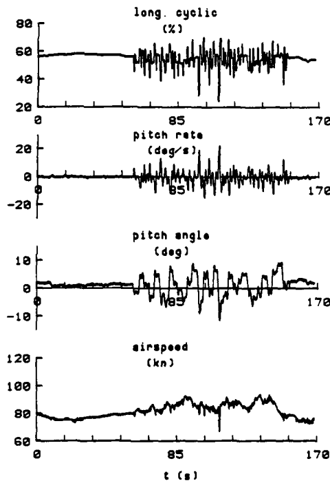
Fig 12 Time histories of control input and response during tracking Pilot P1, augmentation engaged, 80 kn
