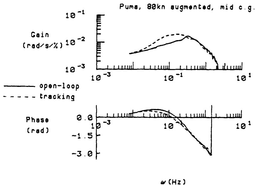
Fig 20 Comparison of open and closed-loop (tracking) pitch rate to longitudinal cyclic frequency responses Pilot P1
