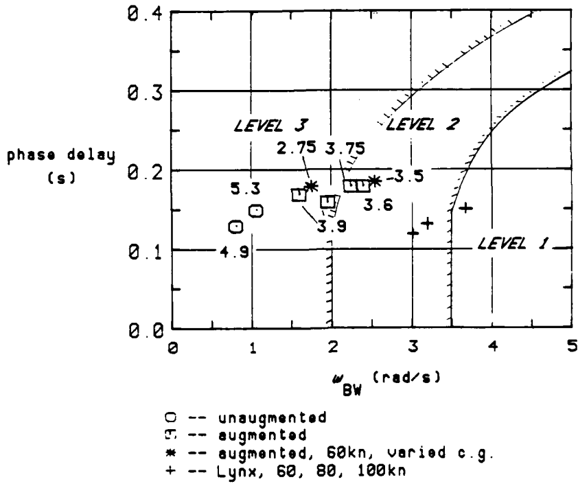
Fig 26 Puma and Lynx pitch axis dynamics characterised by phase delay and phase-limited bandwidth - latest (Ref 5) form for air-air combat
