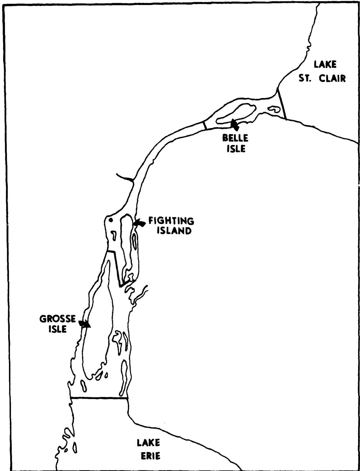
Figure 22. Aerial subdivisions of Detroit River used to compare aerial and ground surveys.
