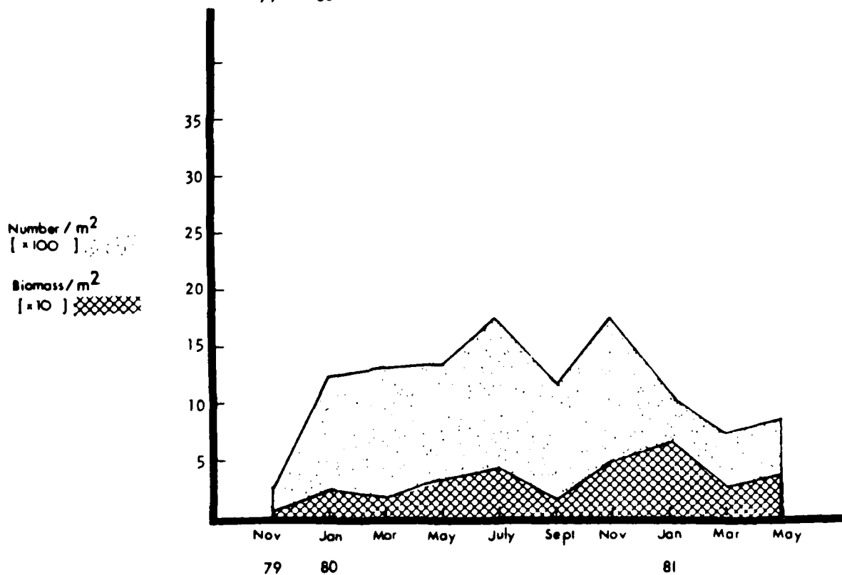
Figure 27. Oligochaete densities at 2m for 10 sampling periods, 1979-1981.
