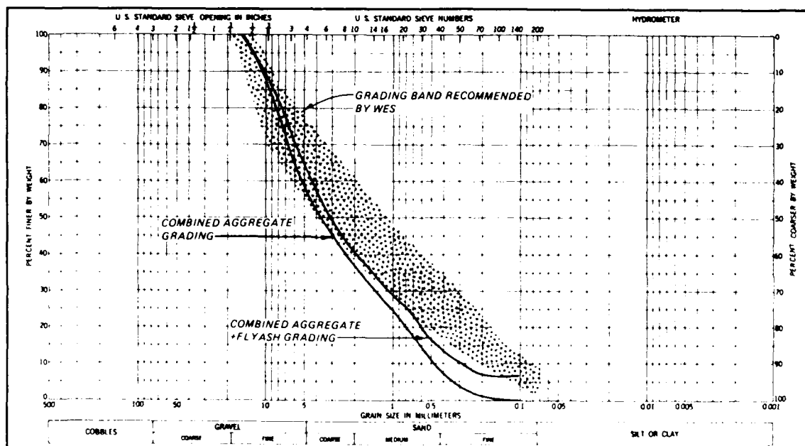
Figure 2. RCC Aggregate Grading
