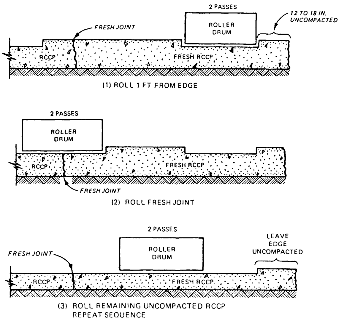
Figure 5. Roller Pattern: Fresh Joint Construction (from Pittman 1986)
