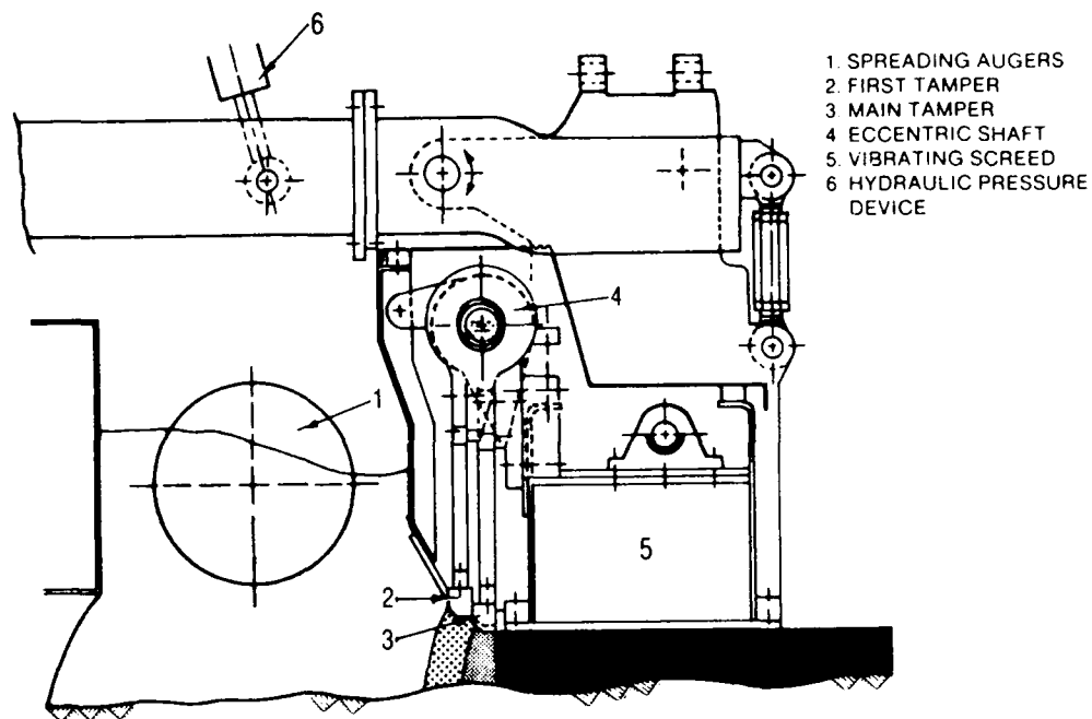
"ABG PAVER FINISHER TITAN 420"
