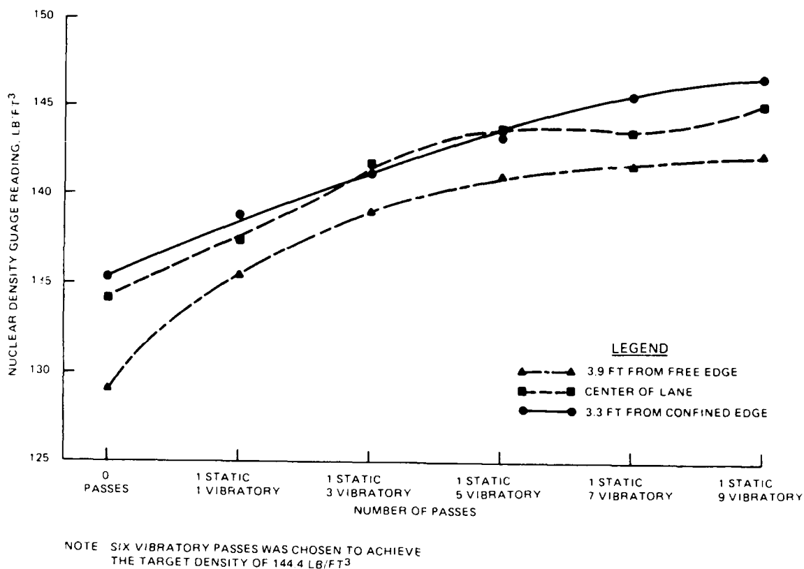
Figure 11. Roller Passes Versus RCC Density
