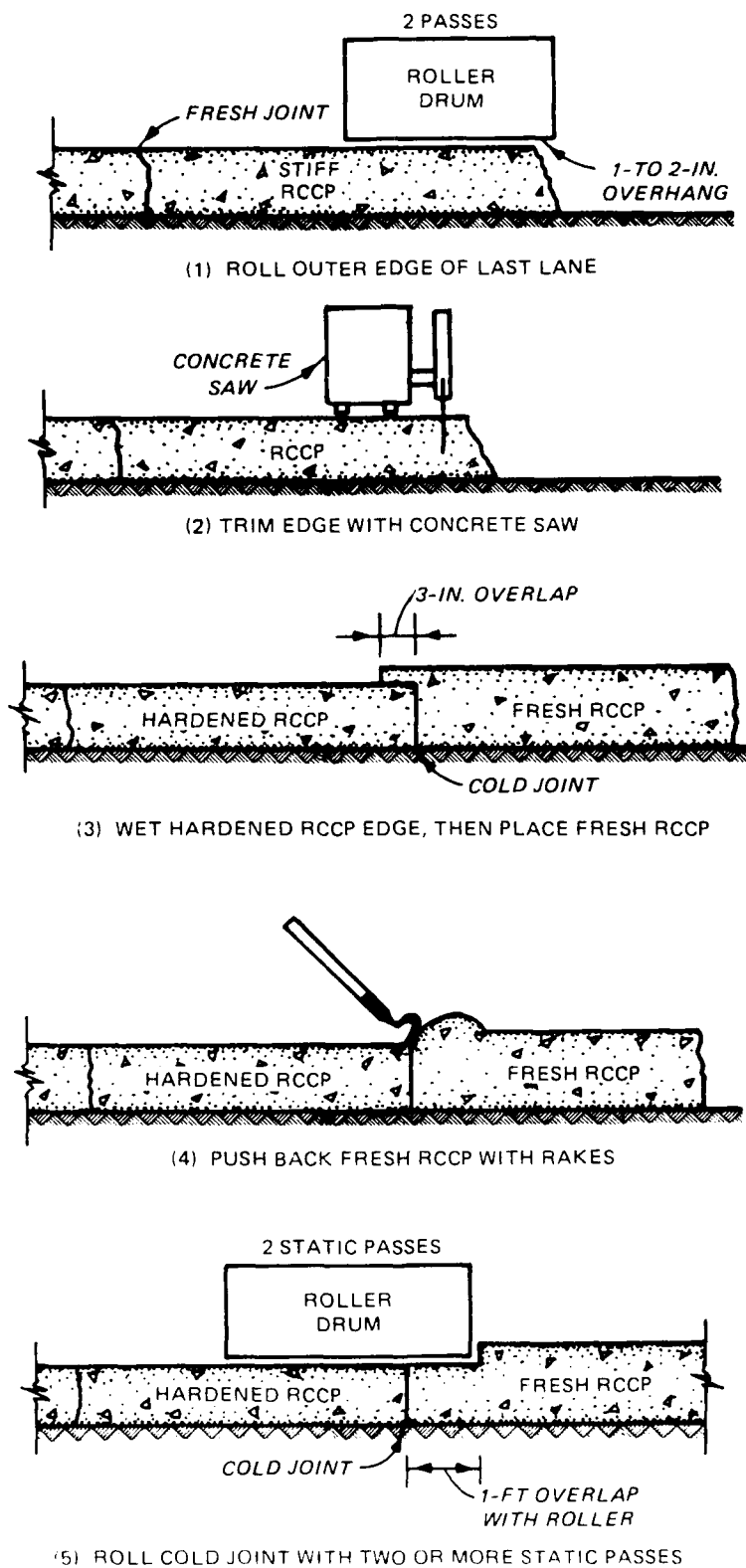
Figure 6. Roller Pattern: Cold Joint Construction (from Pittman 1986)
