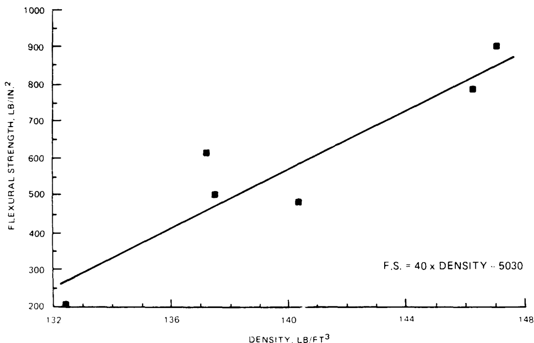
Figure 15. 28-Day Flexural Strength Versus Density
