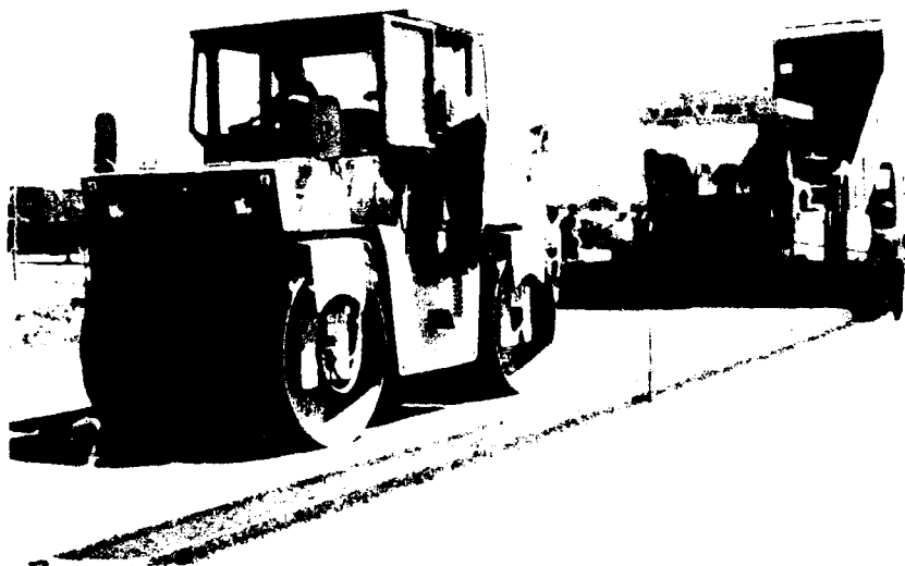
Photo 34. The 10-ton vibratory roller followed immediately behind the paver for primary compaction
