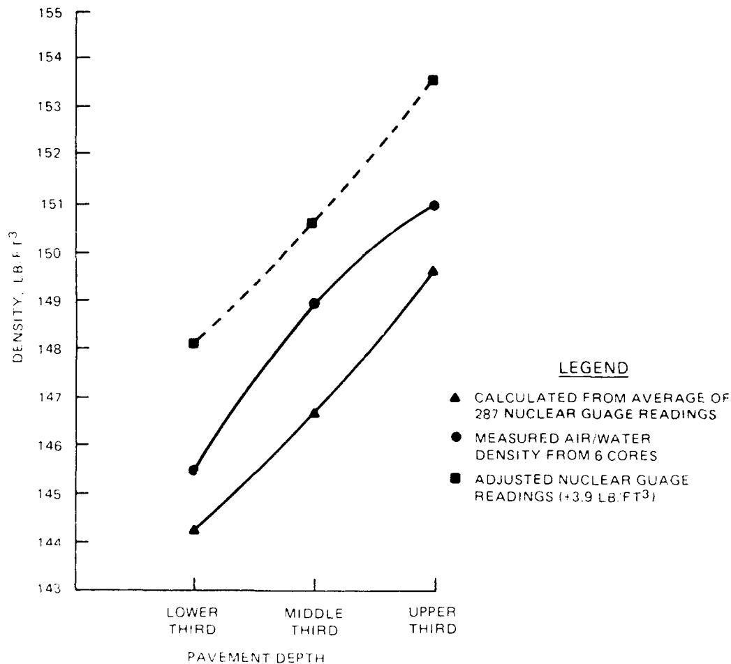
Figure 18. RCC Density Versus Pavement Depth
