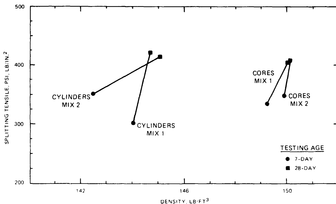
Figure 12. Splitting Tensile Strength Versus Density
