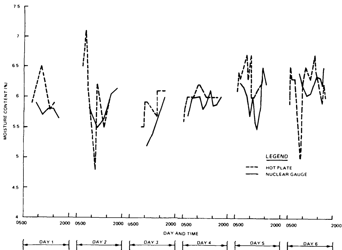
Figure 19. Variation of RCC Moisture Content With Time
