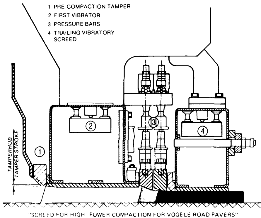
"SCREED FOR HIGH POWER COMPACTION FOR VÖGELE ROAD PAVERS"
