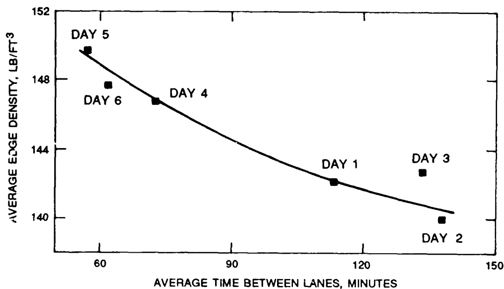
Figure 16. Effect of Delayed Compaction on Joint Density
