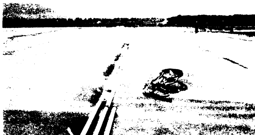
Photo 43. At the end of the day, an irrigation-type sprinkler system was set up to moist cure the RCC for seven days
