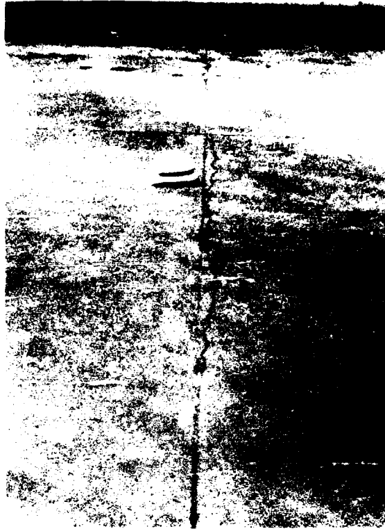
Photo 59. This crack formed ahead of the saw during cutting, indicating that the sawing occurred too late
