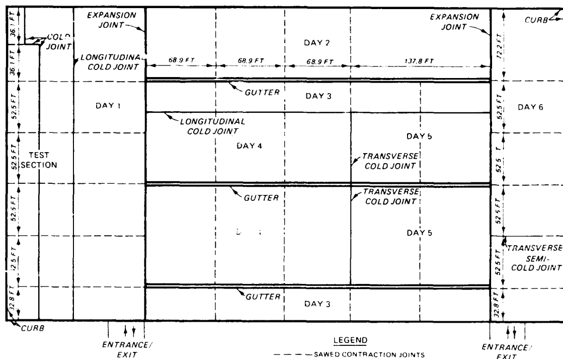
Figure 7. Location of Cold and Contraction Joints
