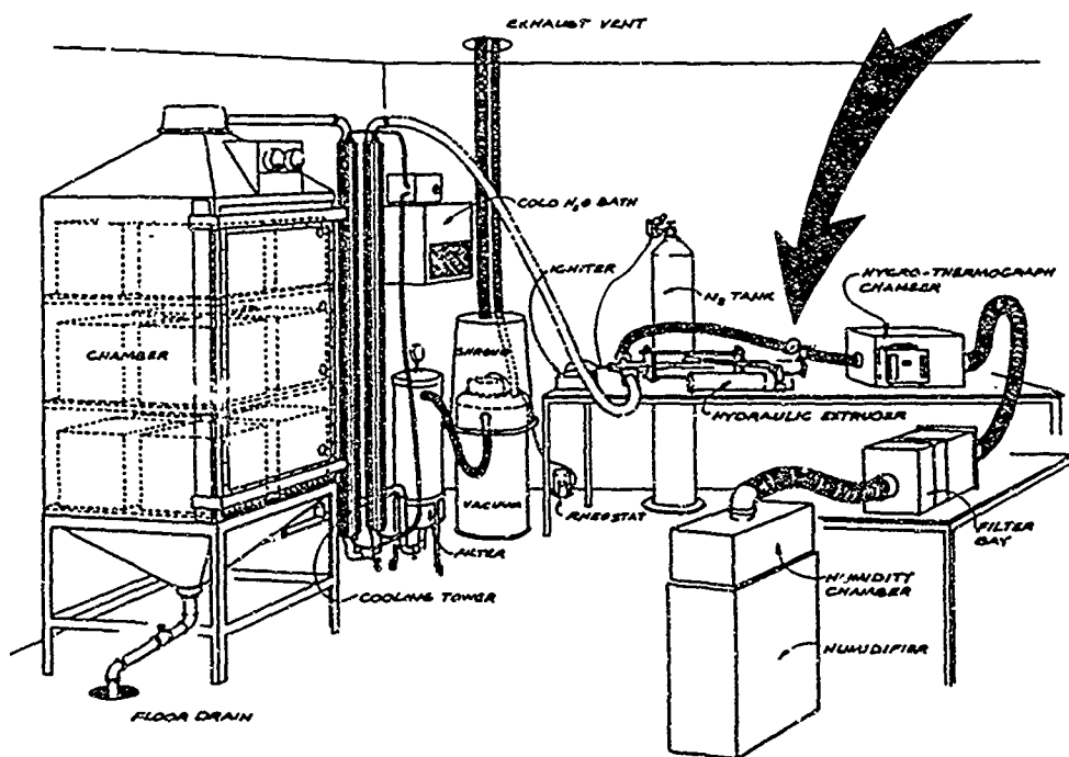
Figure 2. Technical illustration of the Modified RP/BR Extruder and Inhalation Chamber System. (Note.--Components of the System are scaled relative to the perspective, i.e., 2.54 cm equals 0.6 m, but the location of some components has been drawn to improve the visual display.) The insert shows a schematic diagram of the RP/BR extruder/generator subsystem--the equipment used to automatically extrude the softened RP/BR product into the glass burn chamber where it is ignited to generate aerosol in the intake airstream (from Holmberg, Moneyhun and Gayle, 1985).
