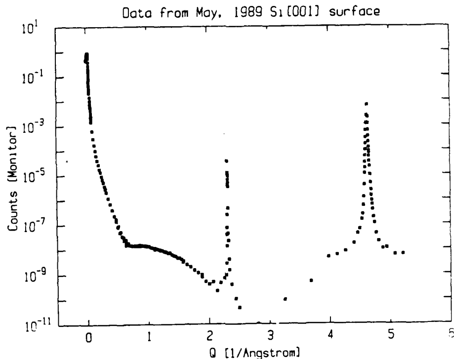
Figure 1.2. X-ray specular reflectivity from the [001] face of a Si crystal coated with approximately 7 Å SiO 2 . The peak near Q \approx 4.6 \text{ \AA}^{-1} corresponds to the [004] Bragg reflection. The sharper peak at Q \approx 2.3 \text{ \AA}^{-1} arises from multiple scattering such as the [111] and [\bar{1}\bar{1}\bar{1}] and is sensitive to rotation of the sample around the [001] direction.
