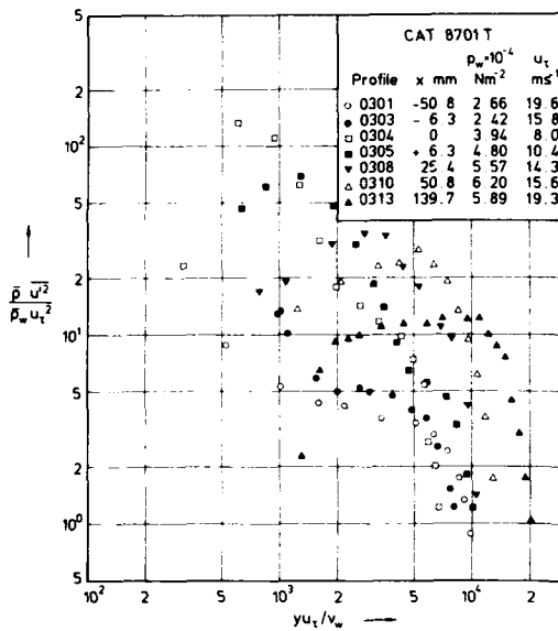
Fig. 11.2.24 Distributions of the Reynolds normal stress in a compressible boundary layer along a compression corner ( 16^\circ ). ( T_w/T_r \approx 1.10 , origin not defined, c_f from Preston tube). Muck et al. (1987).
