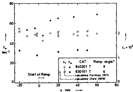
Fig. 10.3.6 Skin friction and c f -distributions in compressible boundary layers along two compression corners (Deblève 1983, Ardonceau 1984). 2.3 > M 0 > 1.8, 5500 > Re δ 2 > 2300.
