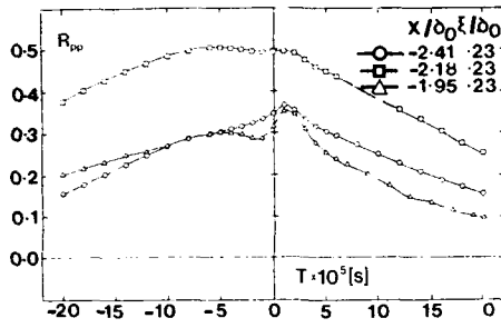
Figure 11: Longitudinal space-time correlations in intermittent region: compression ramp at Mach 3
