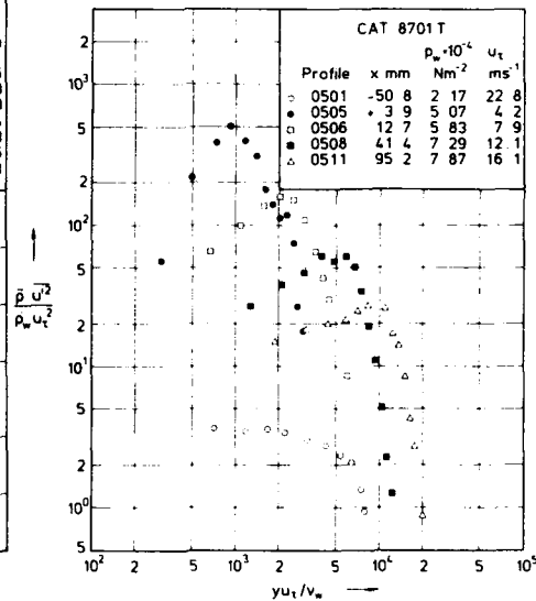
Fig. 11.2.25 Distributions of the Reynolds normal stress in a compressible boundary layer along a compression corner ( 20^\circ ). ( T_w/T_r \approx 1.10 , origin not defined, c_f from Preston tube). Muck et al. (1987).
