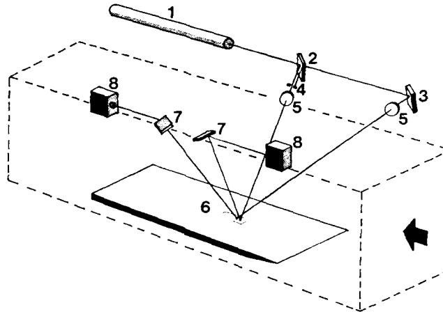
Fig. 1 Diagram of LISF meter: 1 - He-Ne laser, 2 - 50/50 beamsplitter, 3 - planar mirror, 4 - stop, 5 - focusing lens, 6 - flat plate, 7 - planar mirror, 8 - housing for 6328 Angstrom filter, photodiode, and amplifier.
