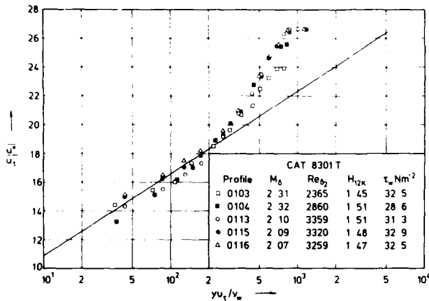
Fig. 10.3.1 Law of the wall for a compressible boundary layer along a compression surface ( 6^\circ ) (adiabatic wall, origin not defined, c_f from correlation of Chew (1978)). Debiève (1983).
