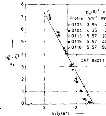
Fig. 10.3.2 Outer law for a compressible boundary layer along a compression surface ( 6^\circ ). Debiève (1983).
