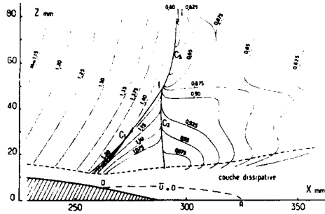
Fig. 10.4.1 Mach-number field of a quasi-normal shock/boundary-layer interaction as deduced from an interferogram. Détery et al. (CAT8002T), copied from author's Fig. 5.
