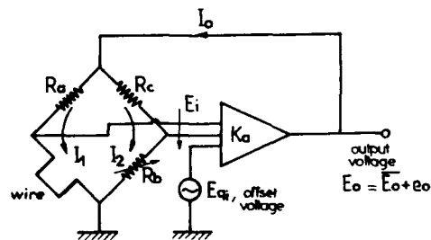
Figure 2. Constant temperature circuit.
