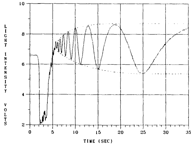
Fig. 2 Typical LISF fringe record ( M = 2.98 , \nu = 500 centistokes).
