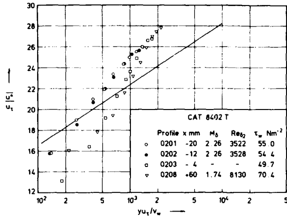
Fig. 10.3.4 Law of the wall for a compressible boundary layer along a compression corner (13°), (adiabatic wall, origin not defined, c f from Fernholz (1971)). Ardonceau (1984).
