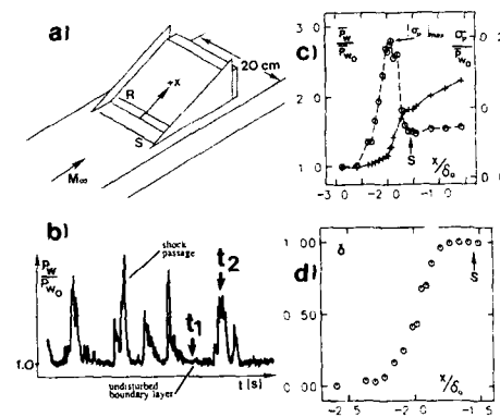
Figure 5: Mach 3 compression ramp flow (a) flow features (b) pressure signal upstream of "S" (c) distribution of mean pressure and rms of pressure fluctuations (d) intermittency
