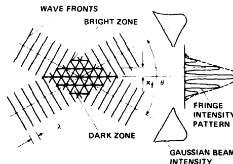
Figure 2. Depiction of fringe formation at beam crossover.
