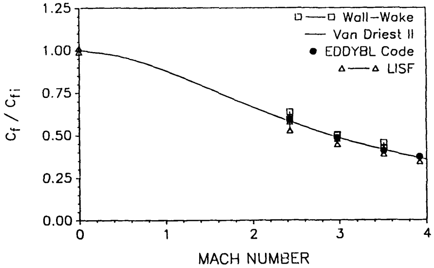
Fig. 6 LISF calibration plot of c_f / c_{fi} vs. Mach number.
