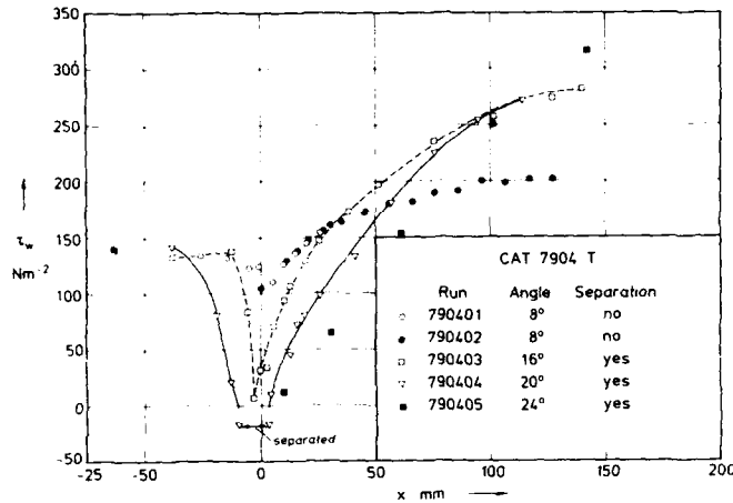
Fig. 10.3.7 Skin friction distributions for compressible boundary layers along 4 compression corners ( c_f from Preston tube): Settles (1979). (Lines are for clarification only).
