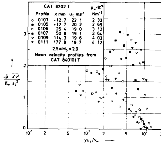
Fig. 11.3.2 Distributions of the Reynolds shear stress in a compressible boundary layer along a concave compression surface with a recovery section. ( T_w/T_r \approx 1.10 , origin not defined, c_f from Preston tube.) Jayaram et al. (1987).
