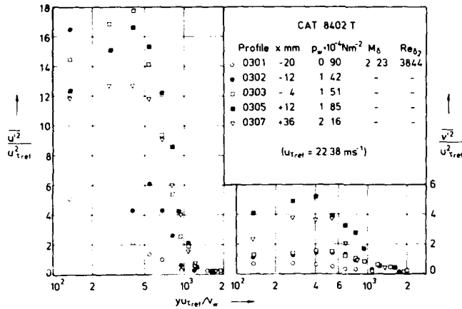
Fig. 11.2.21 Distributions of the specific Reynolds normal stress in a compressible boundary layer along a compression corner (18°), (adiabatic wall, origin not defined). Ardonceau (1984).
