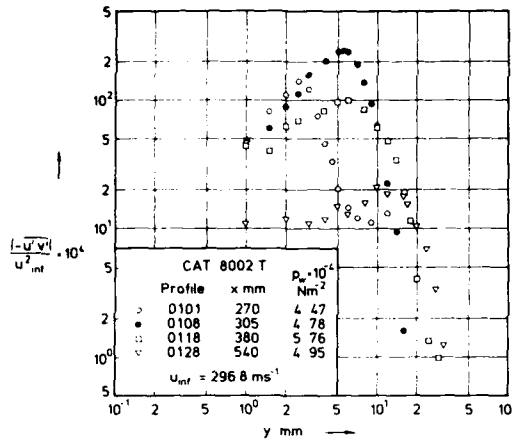
Fig. 11.3.10 Distributions of the specific Reynolds shear stress in a compressible boundary layer with a shock interaction (adiabatic wall, origin not defined). Déleury et al. (1980).
