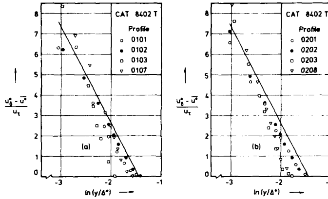
Fig. 10.3.5 Outer law for a compressible boundary layer along a compression corner (8° and 13°). Ardonceau (1984).
