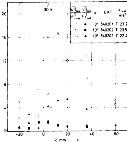
Fig. 11.2.22 Development of the maxima of specific Reynolds normal stresses in compressible boundary layers along 3 compression corners. Ardonceau (1984).
