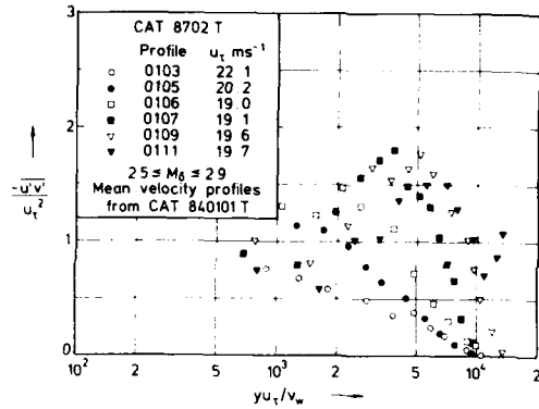
Fig. 11.3.3 Distributions of the specific Reynolds shear stress in a compressible boundary layer along a concave compression surface with a recovery section. ( T_w/T_r \approx 1.10 , origin not defined, c_f from Preston tube.) Jayaram et al. (1987).
