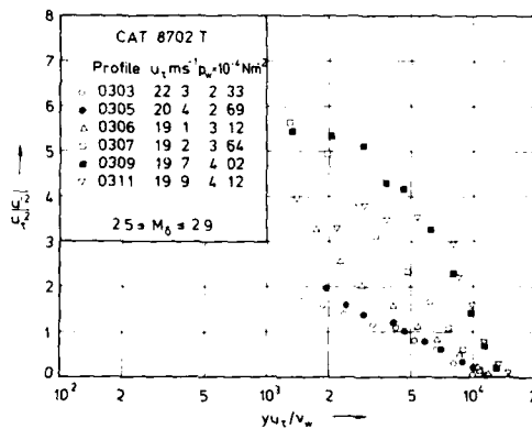
Fig. 11.2.12 Distributions of the specific Reynolds normal stress in a compressible boundary layer along a concave compression surface with a recovery section ( T_w/T_r \approx 1.10 , origin not defined, c_f from Preston tube). Jayaram et al. (1987).
