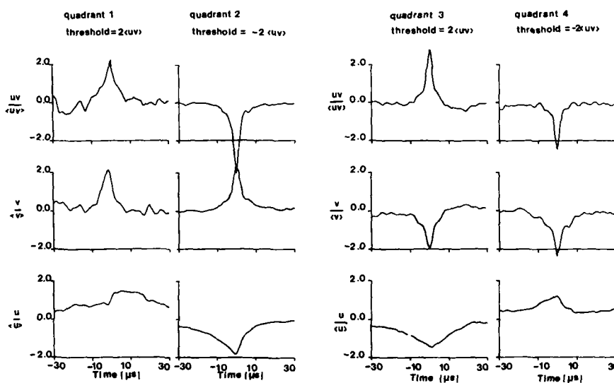
Figure 15. Ensemble-averaged events based on threshold detection applied to u'v' signal at y/\delta = 0.65 : Quadrants I ( u+ , v+ ); II ( u- , v+ ); III ( u- , v- ); IV ( u+ , v- ). (Fernando et al. 1987)
