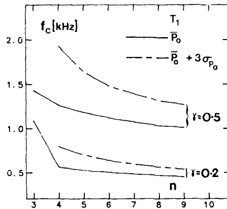
Figure 10: Sensitivity of shock zero crossing frequency to threshold settings
