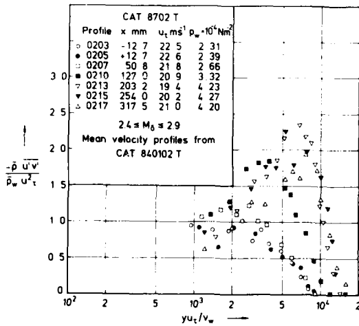
Fig. 11.3.4 Distributions of the Reynolds shear stress in a compressible boundary layer along a concave compression surface with a recovery section. ( T_w/T_r \approx 1.10 , origin not defined, c_f from Preston tube.) Jayaram et al. (1987).
