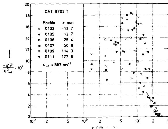
Fig. 11.3.5 Distributions of the specific Reynolds shear stress in a compressible boundary layer along a concave compression surface with a recovery section. ( T_w/T_r \approx 1.10 , origin not defined.) Jayaram et al. (1987).
