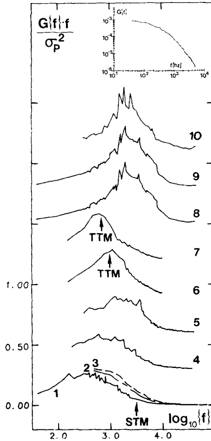
Figure 7 Power spectra at location of (\sigma_p)_{\max} (curves 1-3 on axes as shown; curves 4-10 are shifted 0.3 units of f \cdot G(f) / \sigma_p^2 upwards)
