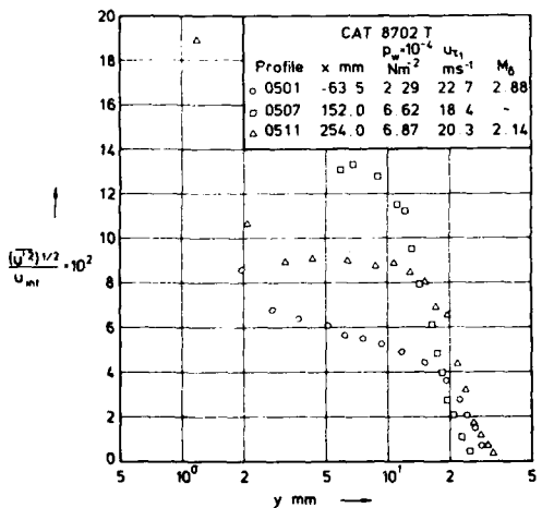
Fig. 11.2.15 Distributions of the root mean square of the fluctuating velocity u' in a compressible boundary layer long a concave compression surface with a recovery section ( T_w/T_r \approx 1.10 , origin not defined, u_{inf} = 519.6 ms -1 ). Donovan & Smits (1987).
