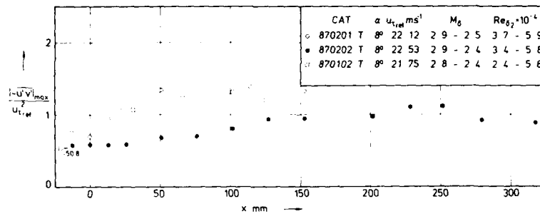
Fig. 11.3.1 Distributions of the maxima of the specific Reynolds shear stress in a compressible boundary layer along 3 compression surfaces with different concave curvature at the beginning ( T_w/T_r \approx 1.10 , origin not defined). Jayaram et al. (1987), Muck et al. (1987).
