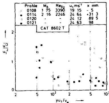
Fig. 11.2.8 Distributions of the specific Reynolds normal stress in a compressible boundary layer with a rapid expansion. (origin not defined, adiabatic wall, u_{\tau} from Chew (1978)). Dussauge & Gaviglio (1986).
