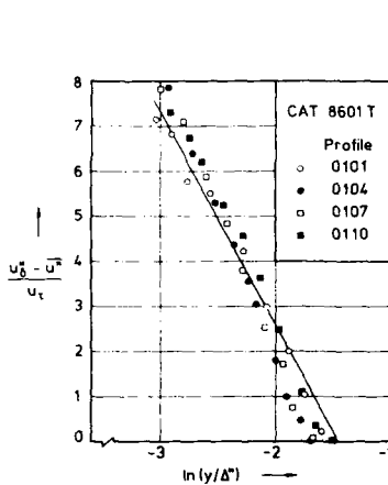
Fig. 10.1.3 Outer law for a compressible boundary layer with an adverse pressure gradient (origin not defined, T_w/T_r \approx 1.10 ). Fernando & Smits (1986).
