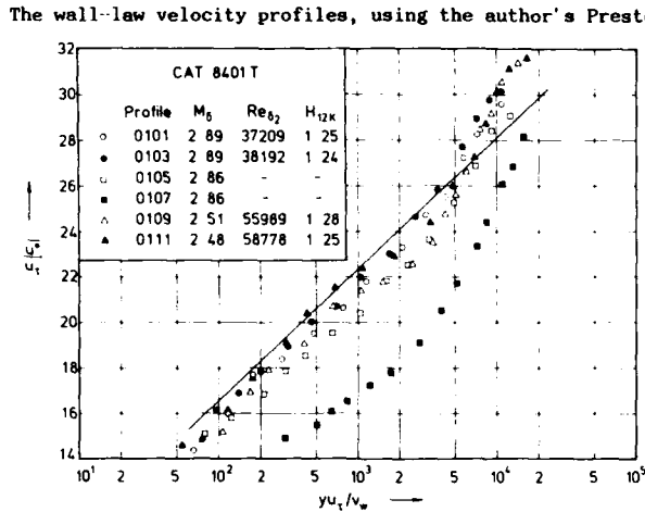
Fig. 10.2.2 Law of the wall for a compressible boundary layer along a concave compression surface (origin not defined, T_w/T_r \approx 1.10 , c_f from Preston tube). Taylor (1984).
